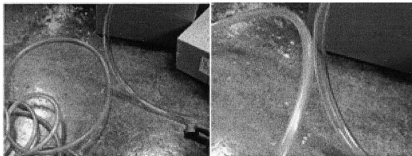
Figures 5.2 a and b: A comparison of the PVC tube used for Spirasol system experiments in Cambridge (left) and an unused PVC tube kept mostly in darkness (right). A) From afar, one can see the bluish tint beginning to develop. B) A close-up shot shows that the Spirasol tube has become rather opaque over the course of a month.
