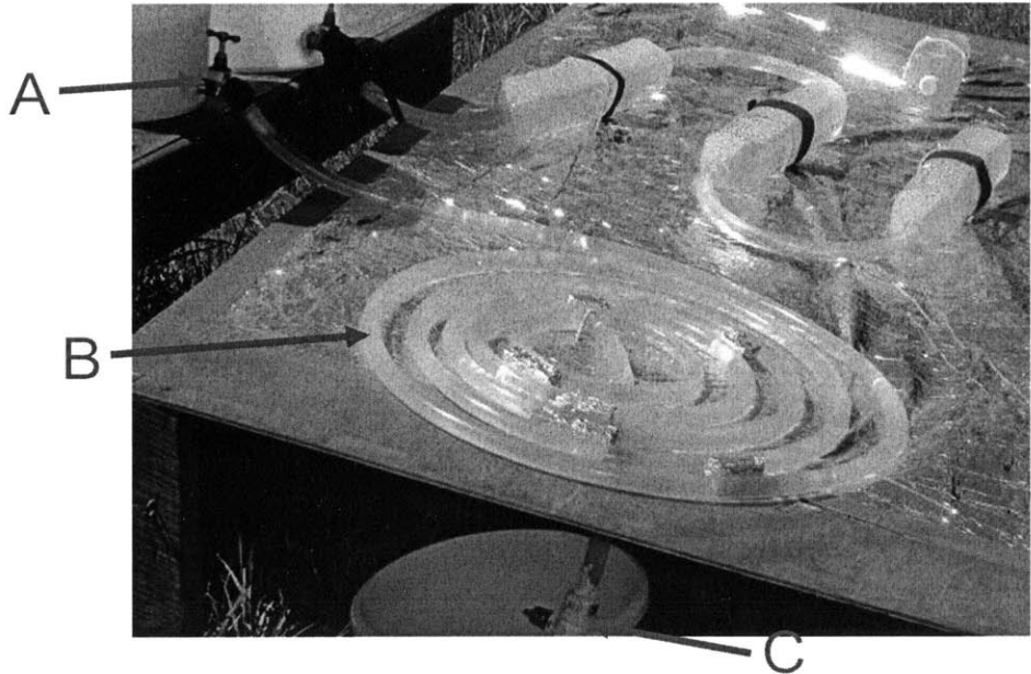
Figure 3.1: Constructed prototype of the Spirasol system. A) Three-quarter-inch faucet; B) Three-quarter-inch inner-diameter PVC tube; C) Three-quarter-inch PVC ball valve.
