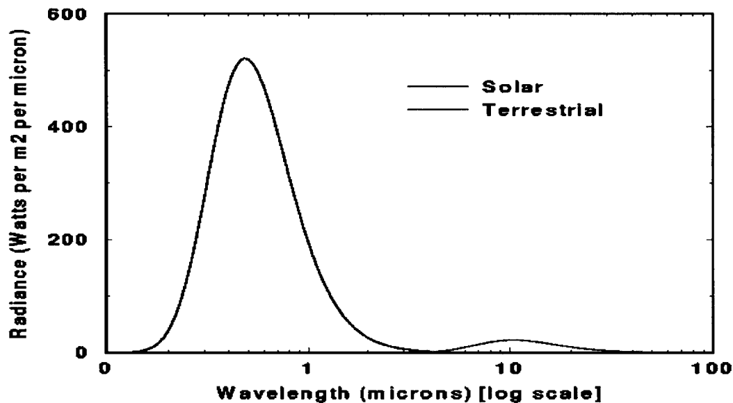
Figure 1.1: Solar and Terrestrial radiation spectra. (Grimes, 1999)
