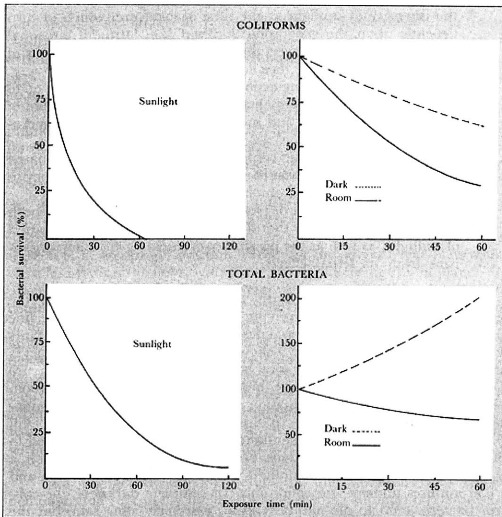
Figure 2.1: Germicidal effect of solar radiation on bacteria contaminating water held in blue glass containers. Identical samples of water kept in the dark and in a room served as controls for comparison. (Acra et al., 1984)
