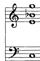
Figure 3-2: A chord.
