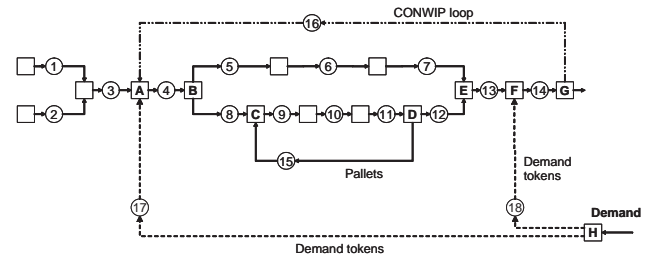
Fig. 2. Assembly/disassembly network with multiple-loop structures
