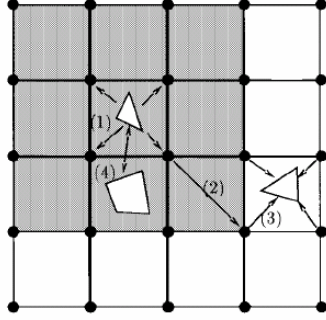
Fig. 1. Four steps of the pre-corrected FFT algorithm
