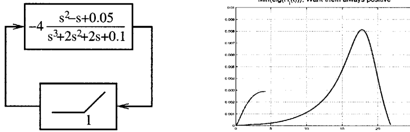
Figure 6-8: System with unstable A_1
