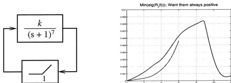
Figure 6-7: System with relative degree 7 (left); global stability analysis when k = 2 (right)
