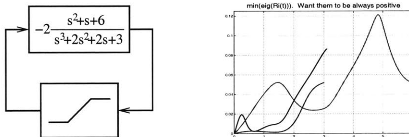
Figure 7-5: 3^{rd} -order system with unstable nonlinearity sector
