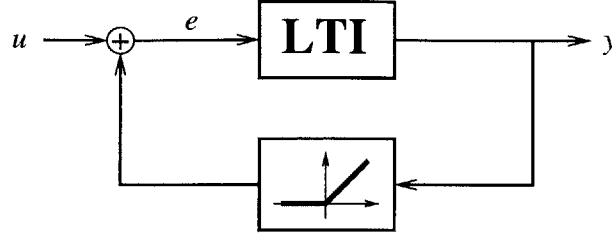
Figure 8-2: On/off system with output disturbance u
