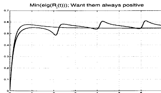
Figure 8-3: Origin is globally asymptotically stable
