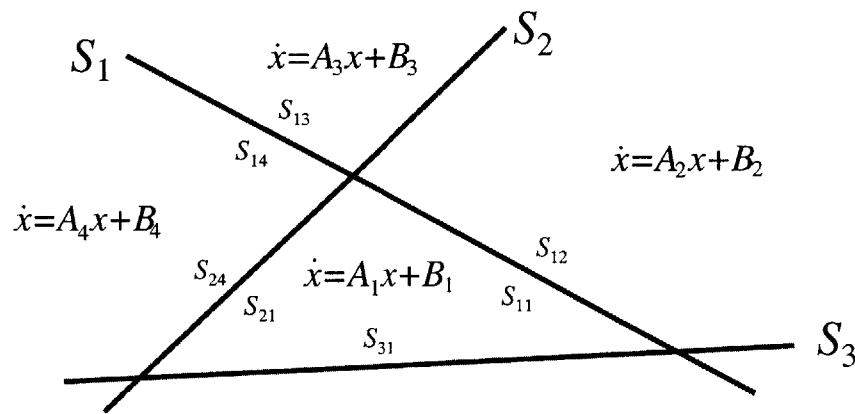
Figure 3-1: Piecewise Linear System with a memoryless switching rule
