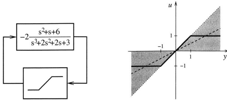
Figure 1-12: 3^{\text{rd}} -order system with unstable nonlinearity sector
