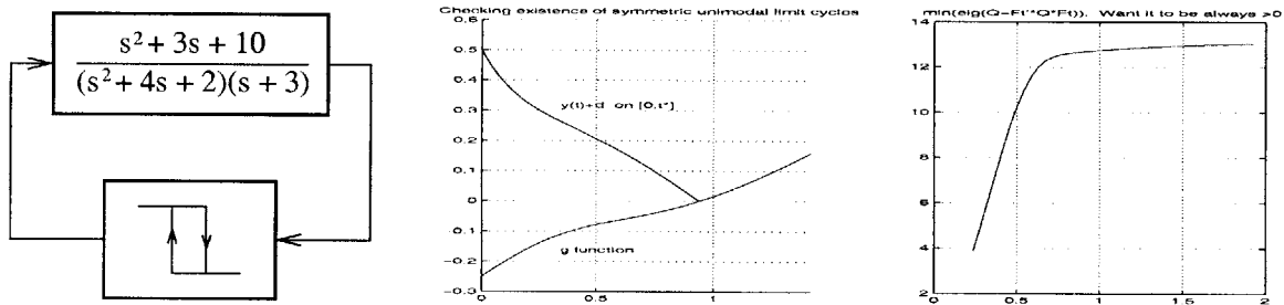
Figure 5-9: 3 rd -order minimum phase system
