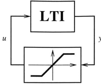
Figure 1-5: Saturation
