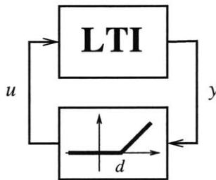
Figure 1-13: On/Off System
