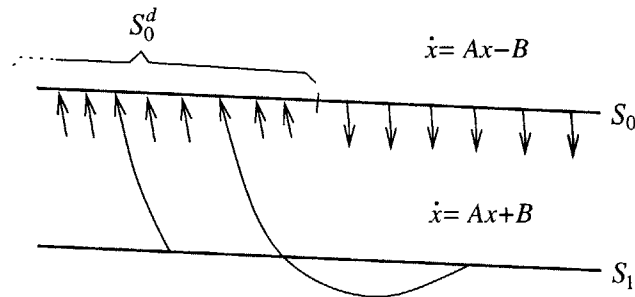
Figure 5-2: The arrival set S_0^d
