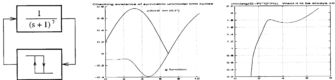
Figure 5-11: System with relative degree 7
