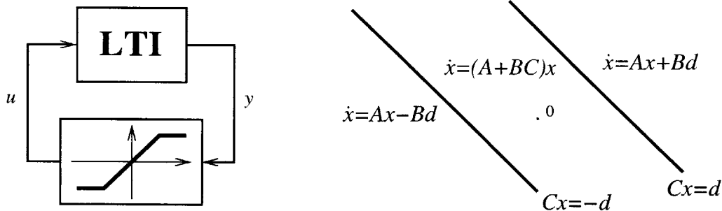
Figure 3-2: Left—Saturation system; Right—state space cells
