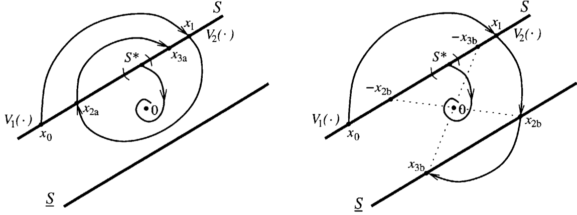
Figure 7-4: Possible state-space trajectories for a SAT
