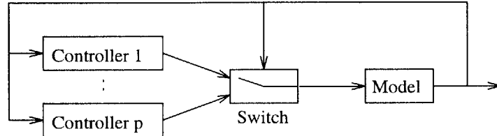
Figure 1-8: Switching between different controllers
