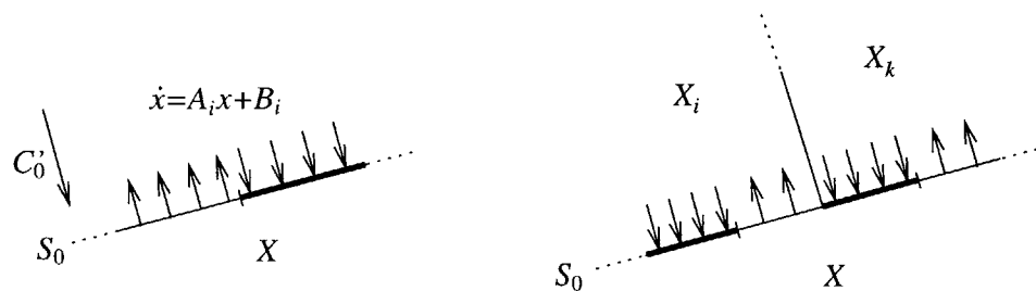
Figure 4-9: Sets in S_0 where S_0^d can be defined, for two different PLS
