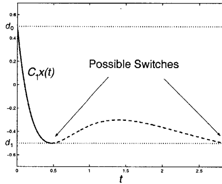
Figure 4-4: Existence of multiple solutions
