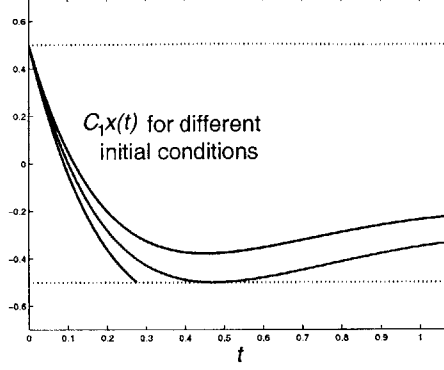
Figure 4-5: Map from \Delta_0 to \Delta_1 is not continuous
