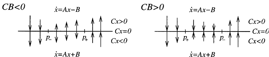
Figure 5-3: Existence of solutions when d = 0
