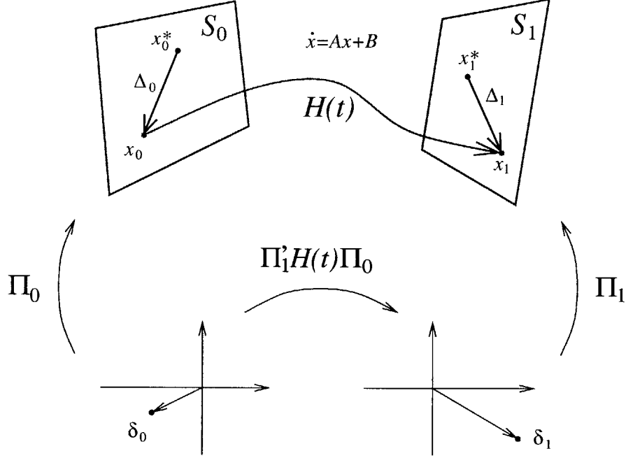
Figure 4-7: n - 1 dimensional map
