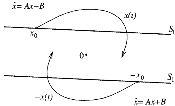
Figure 5-4: Symmetry around the origin
