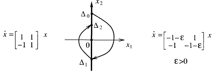
Figure 4-2: Maps from one switching surface to the next switching surface
