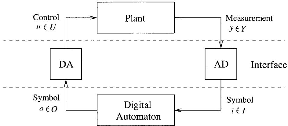
Figure 1-1: Sampled data system
