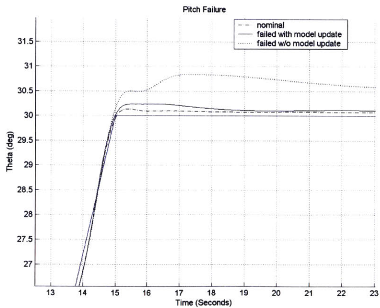
Figure 58: Pitch Frozen Reconfiguration Zoom
