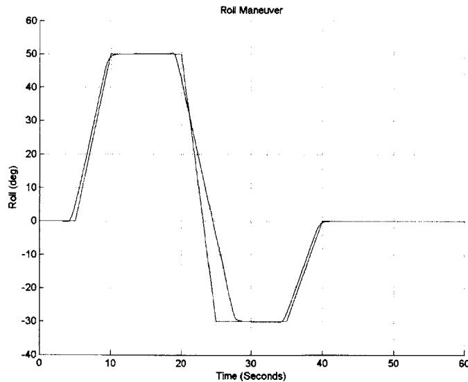
Figure 27: Bank Hold Response
