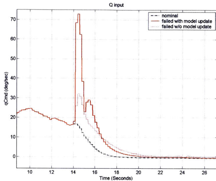
Figure 51: Pitch Controller Reconfiguration Zoom
