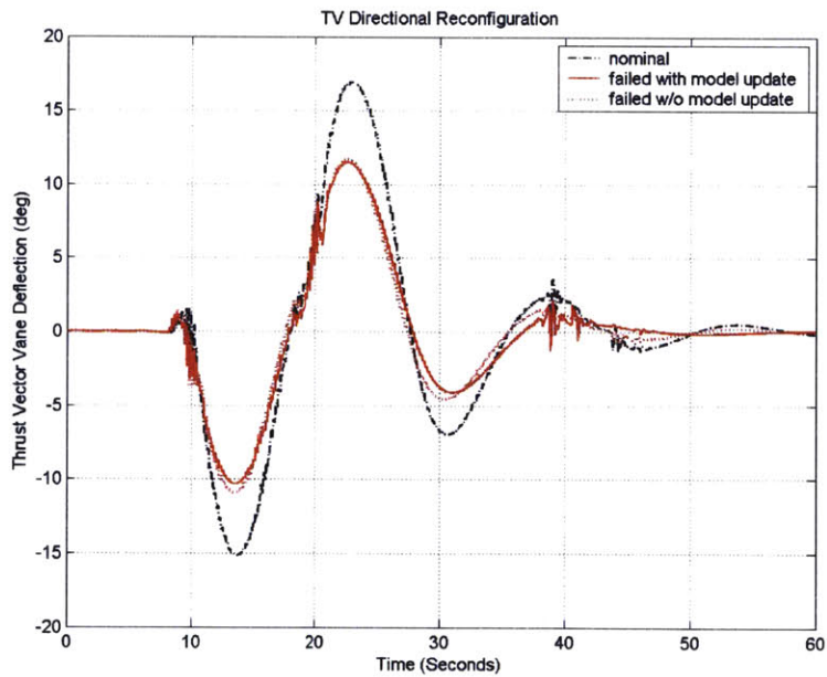
Figure 90: Frozen Rudder Failure Thrust Vane Reconfiguration
