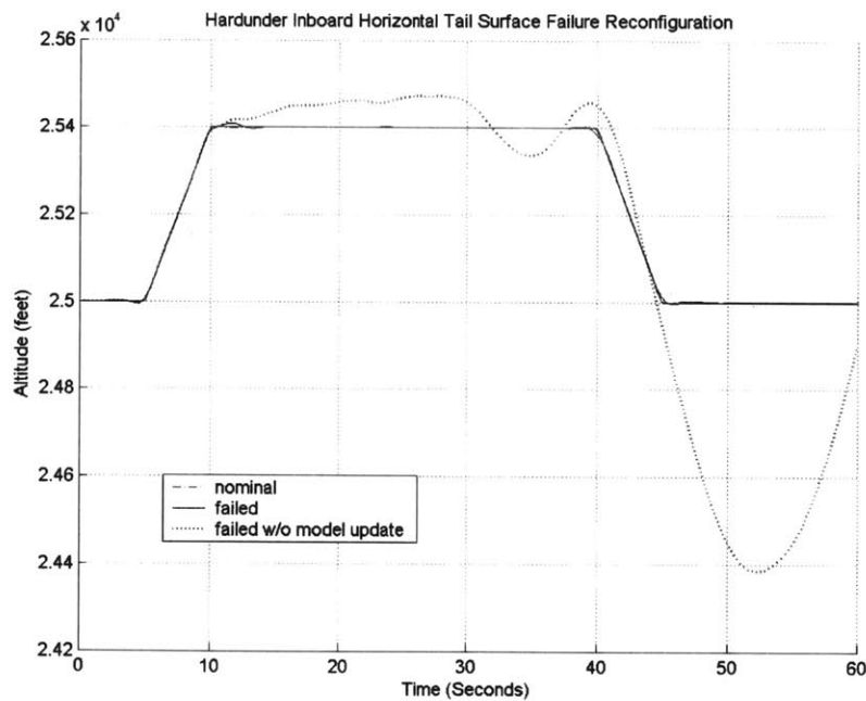
Figure 101: Hardouner Inboard Horizontal Tail Surface Failure Reconfiguration
