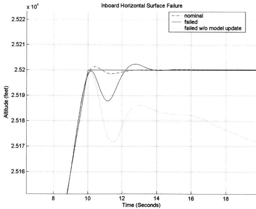
Figure 76: Hardover Inboard Horizontal Tail Surface Failure Reconfiguration with Relaxed Constraints Zoom
