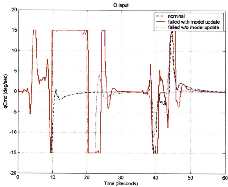
Figure 73: Pitch Rate Command for Hardover Inboard Horizontal Tail Surface Controller Reconfiguration
