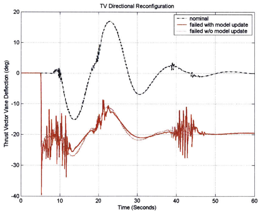
Figure 84: Hardover Rudder Thrust Vane Reconfiguration
