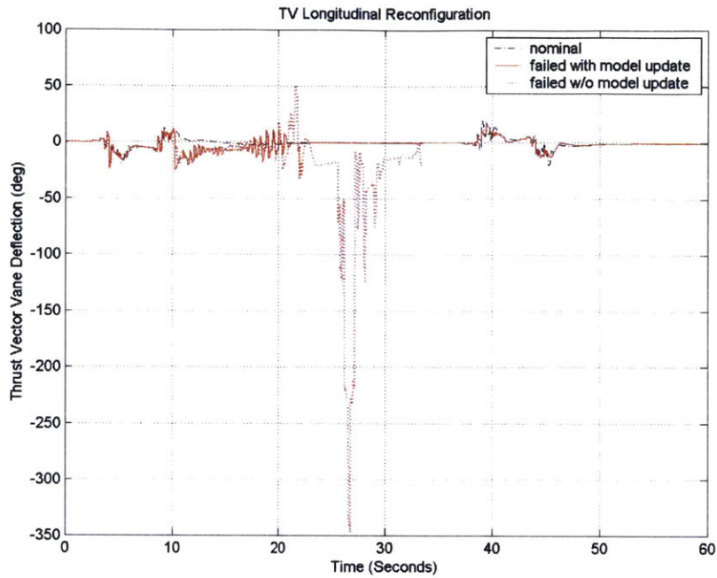
Figure 96: Hardover Inboard Horizontal Tail Surface Failure Thrust Vector Reconfiguration
