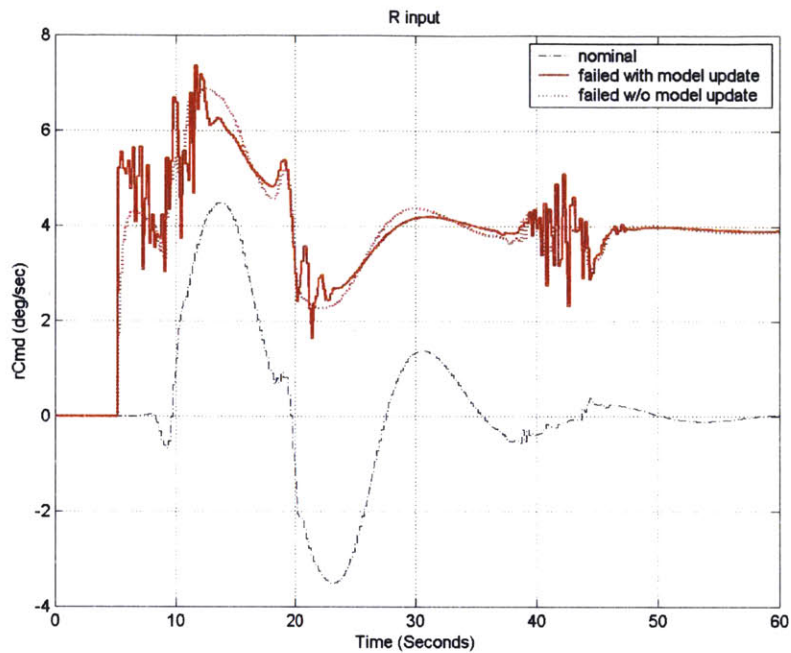
Figure 83: Yaw Rate Command for Hardover Rudder Failure Controller Reconfiguration
