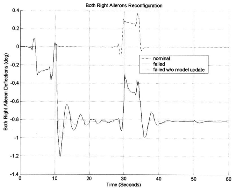
Figure 70: Inboard and Outboard Right Aileron Failure Reconfiguration
