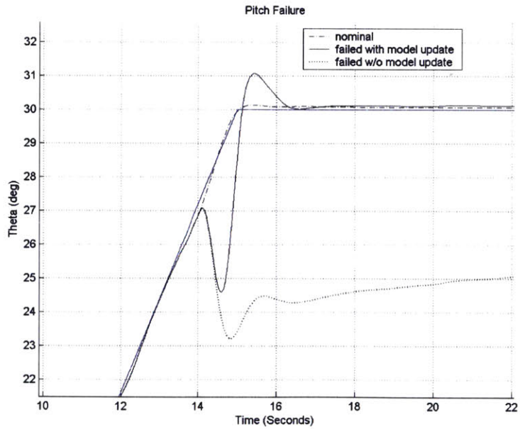
Figure 49: Pitch Failure Zoom
