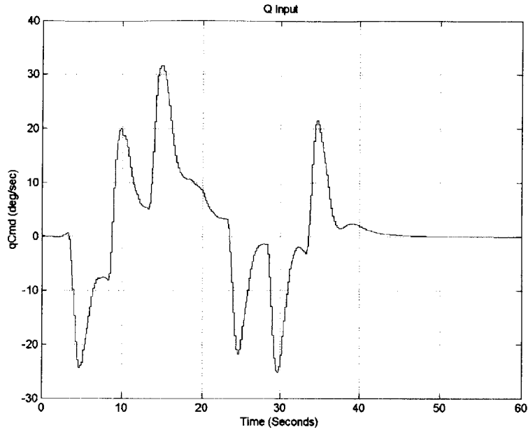
Figure 31: Q Input
