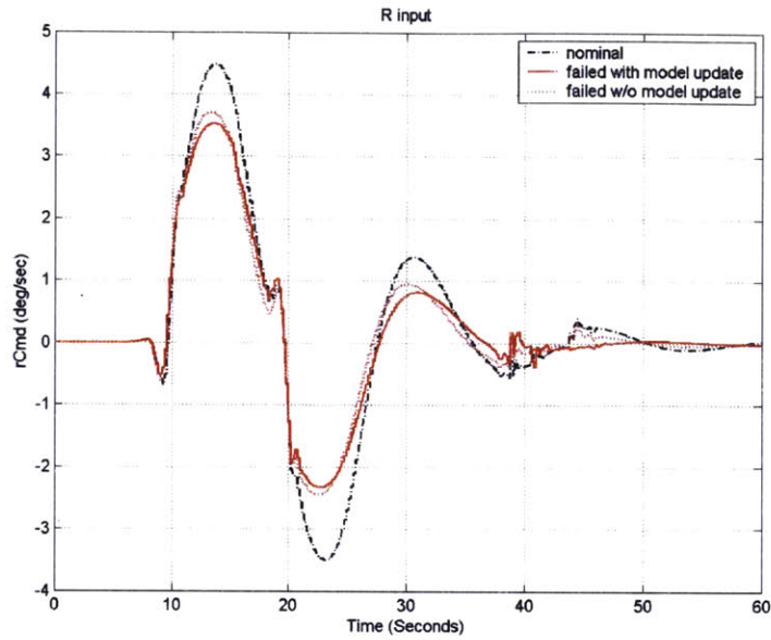
Figure 89: Yaw Rate Command for Frozen Rudder Failure Controller Reconfiguration
