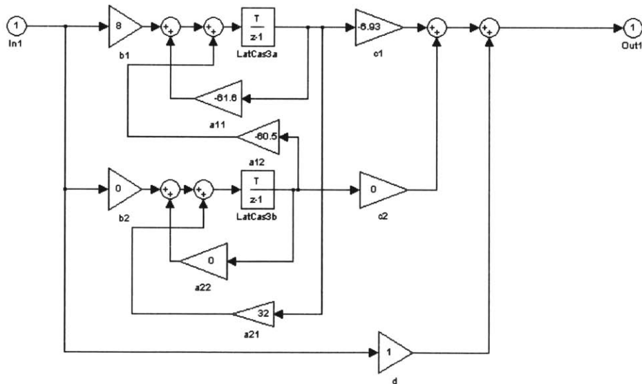
Figure 110: Filter with Explicit Integrators
