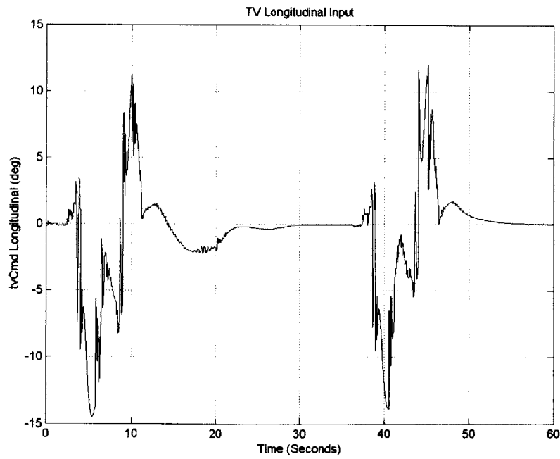
Figure 41: TV Longitudinal Command
