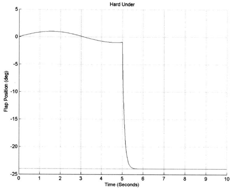
Figure 46: Hard Under Demonstration
