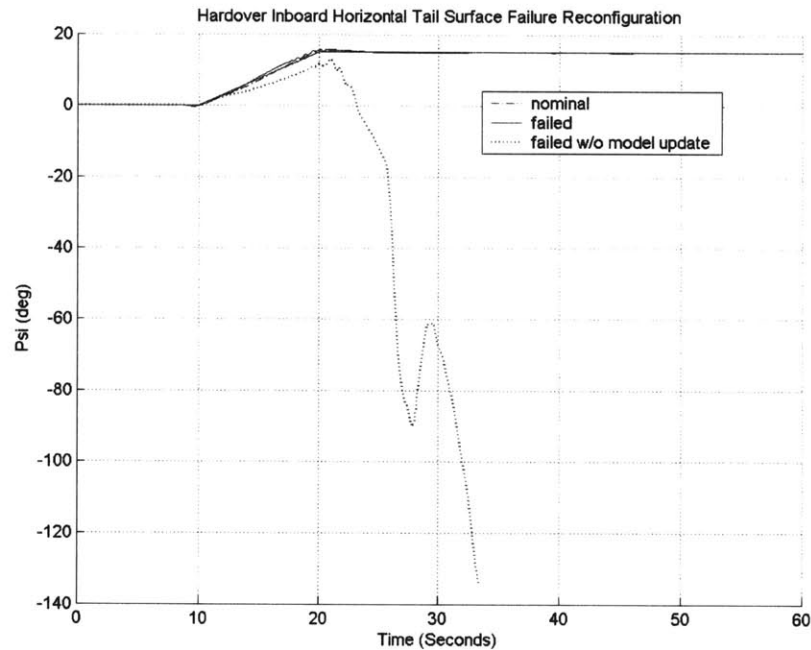
Figure 98: Hardover Inboard Horizontal Tail Surface Failure Reconfiguration
