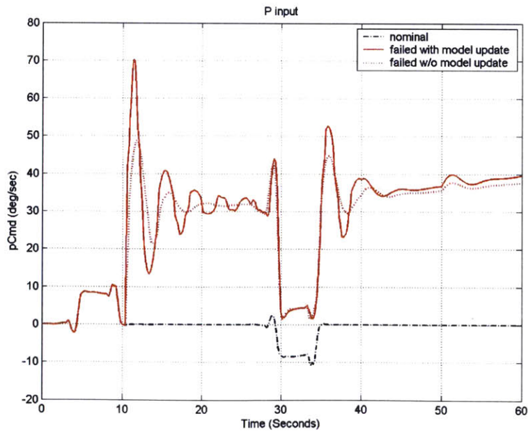
Figure 68: Roll Rate Command for Hardunder Outboard Left Aileron Controller Reconfiguration
