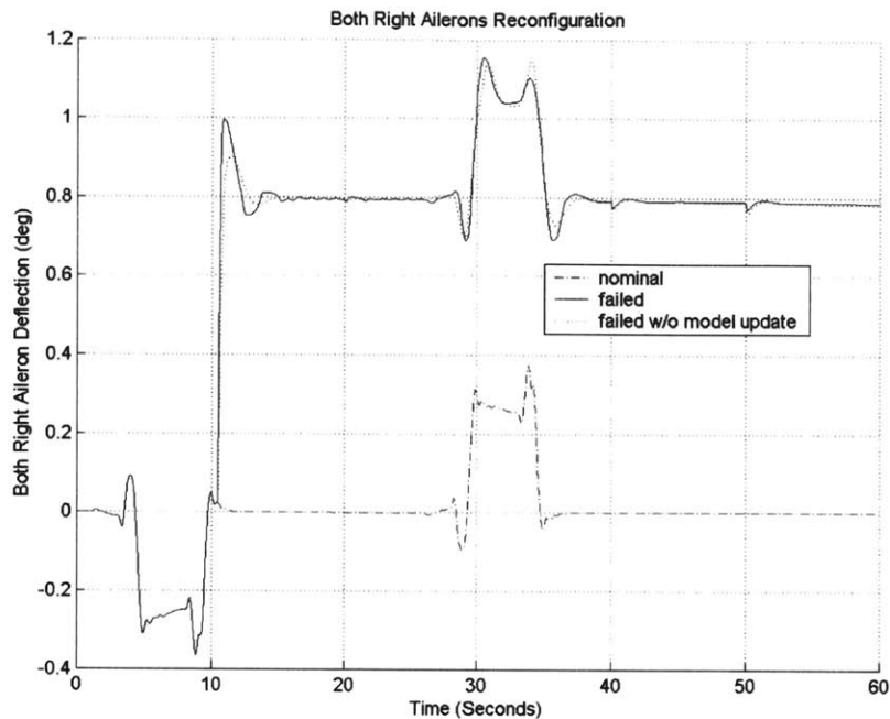
Figure 65: Inboard and Outboard Right Aileron Failure Reconfiguration
