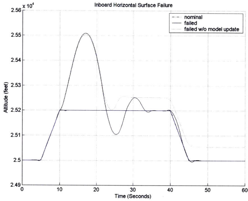
Figure 79: Hardunder Inboard Horizontal Tail Surface Failure Reconfiguration
