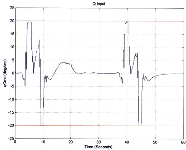
Figure 38: Q Input
