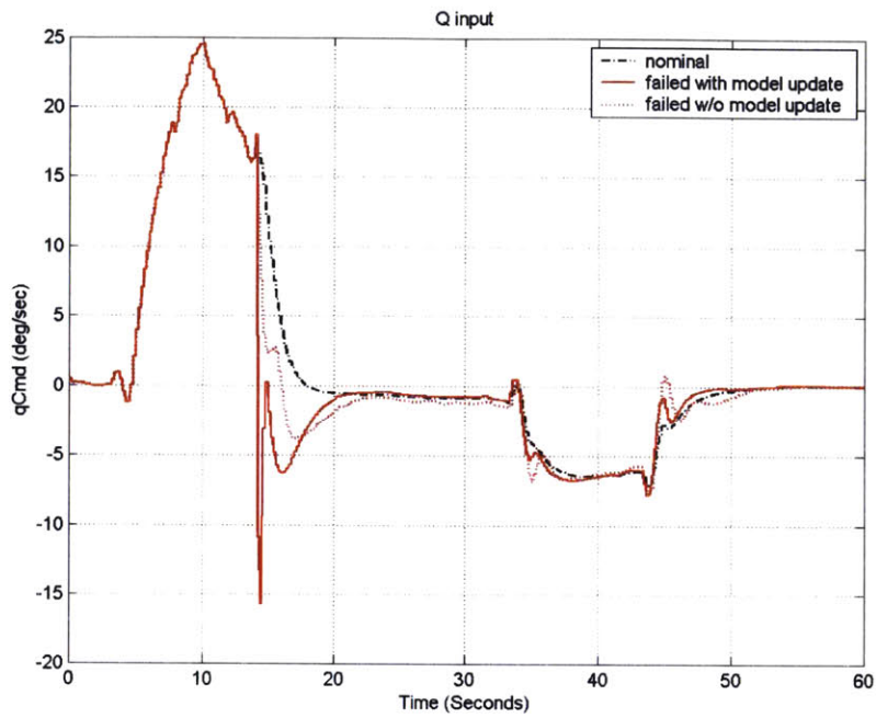
Figure 55: Pitch Hard Under Controller Reconfiguration
