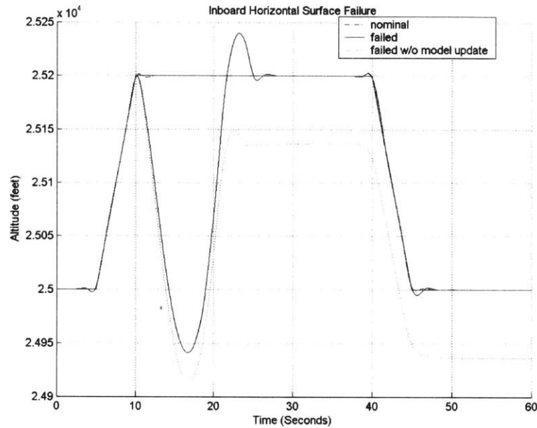
Figure 72: Hardover Inboard Horizontal Tail Surface Failure Reconfiguration
