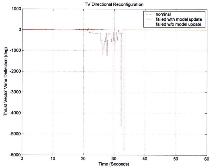
Figure 100: Hardover Inboard Horizontal Tail Surface Failure Thrust Vector Reconfiguration
