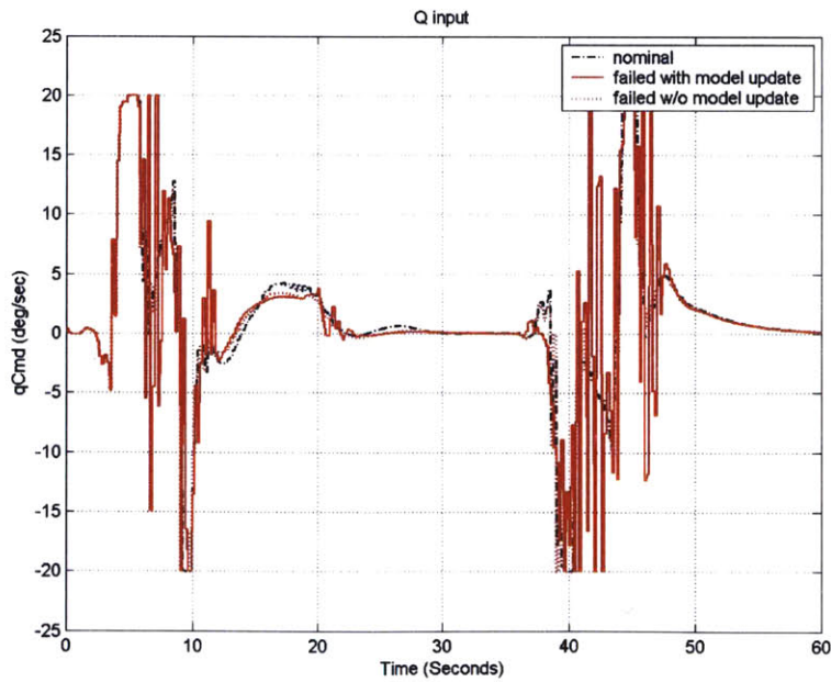
Figure 86: Altitude Rudder Hardover Controller Reconfiguration
