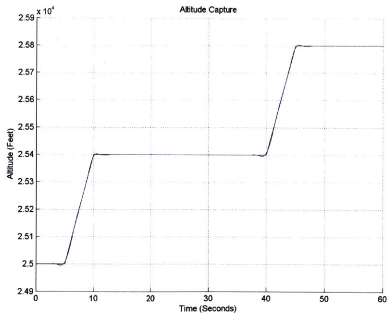
Figure 35: Altitude Capture
