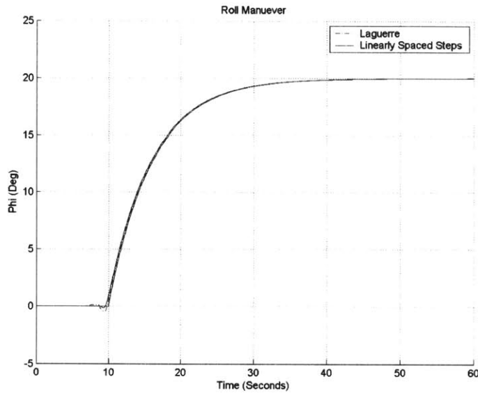
Figure 21: Exponential Maneuver Example
