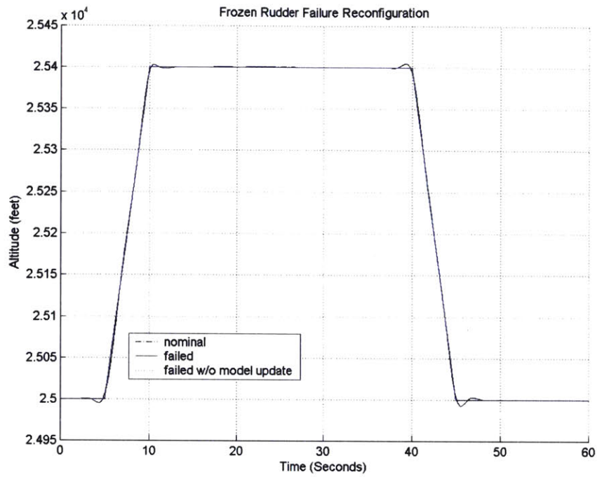
Figure 91: Altitude/Rudder Frozen Reconfiguration
