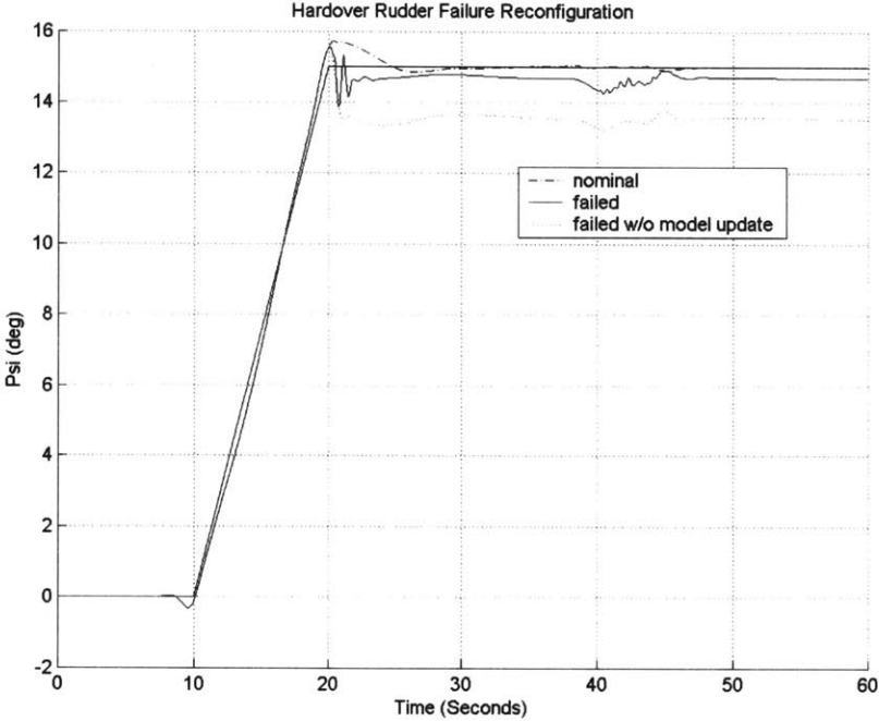
Figure 82: Hardover Rudder Failure Reconfiguration
