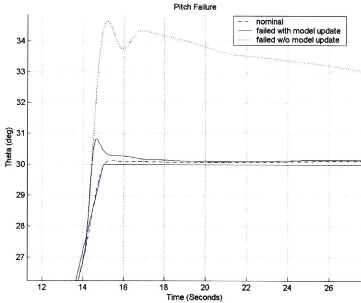
Figure 54: Pitch Hard Under Reconfiguration Zoom
