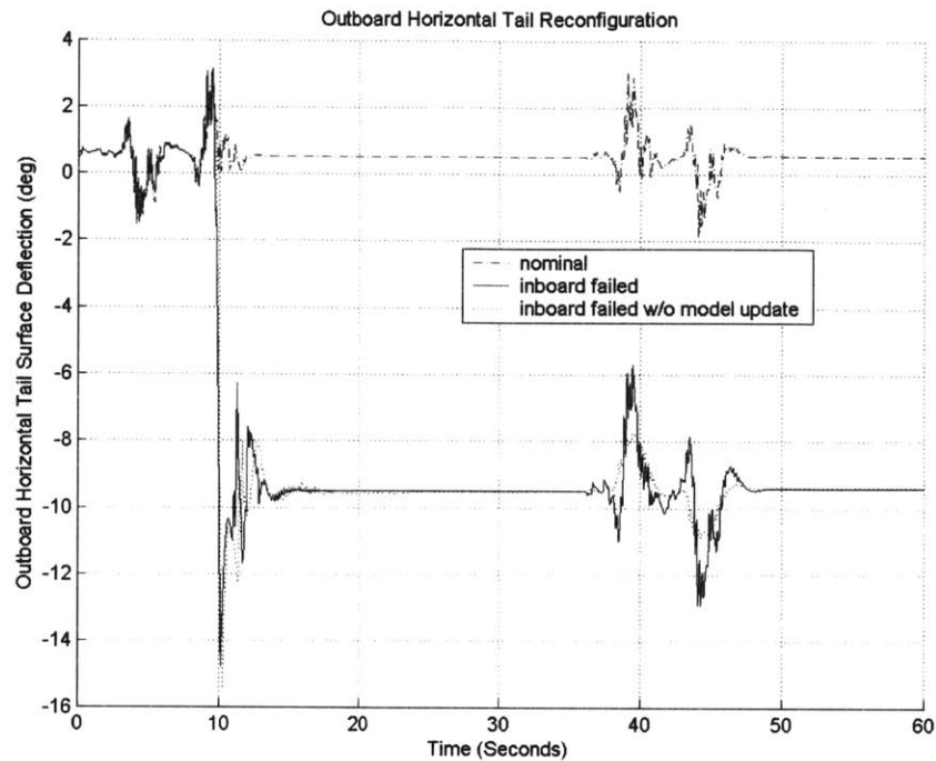
Figure 78: Outboard Horizontal Tail Surface Reconfiguration
