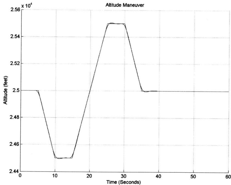
Figure 30: Altitude Capture
