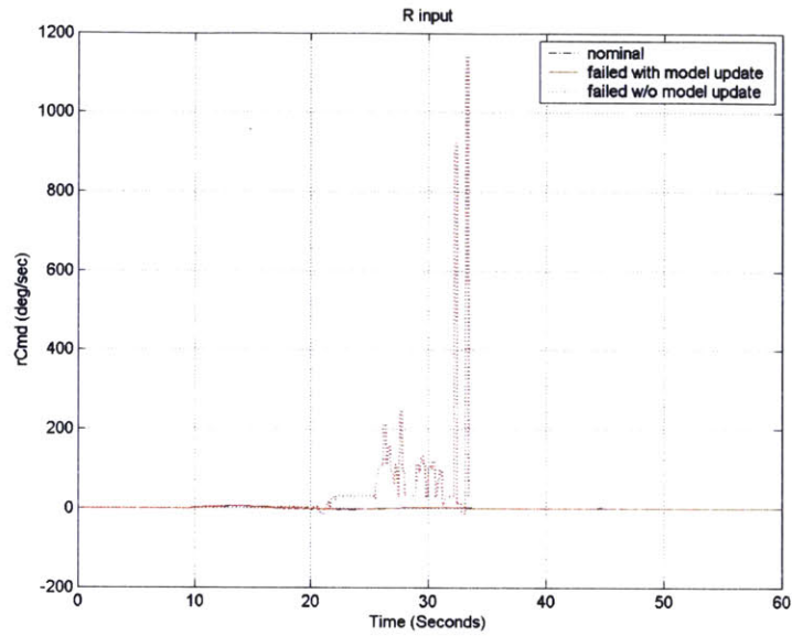
Figure 99: Yaw Rate Command for Hardover Inboard Horizontal Tail Surface Failure Controller Reconfiguration
