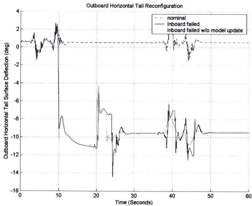
Figure 74: Outboard Horizontal Tail Surface Reconfiguration
