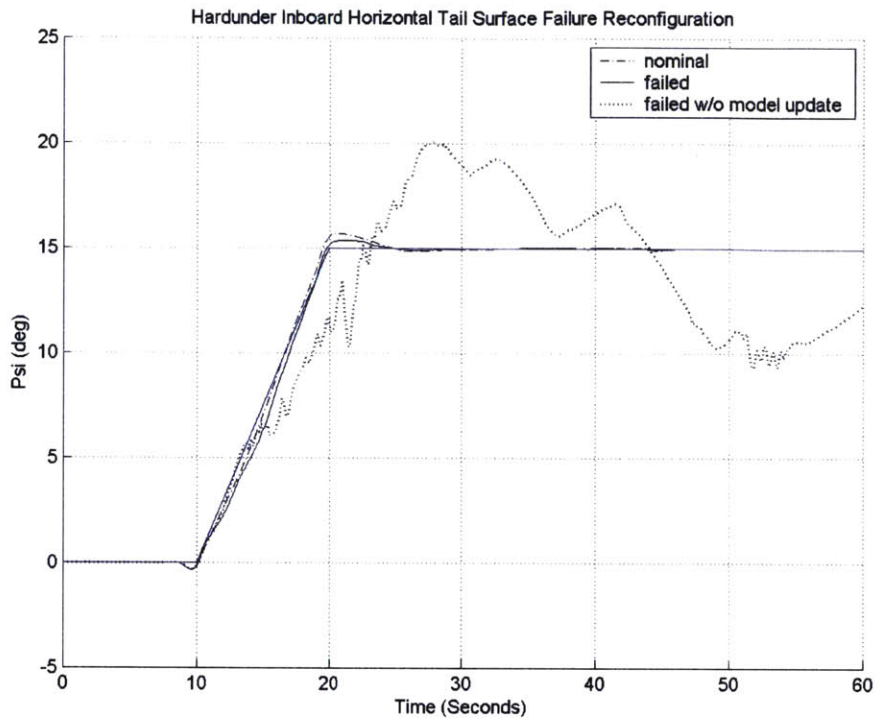
Figure 105: Hardover Inboard Horizontal Tail Surface Failure Reconfiguration
