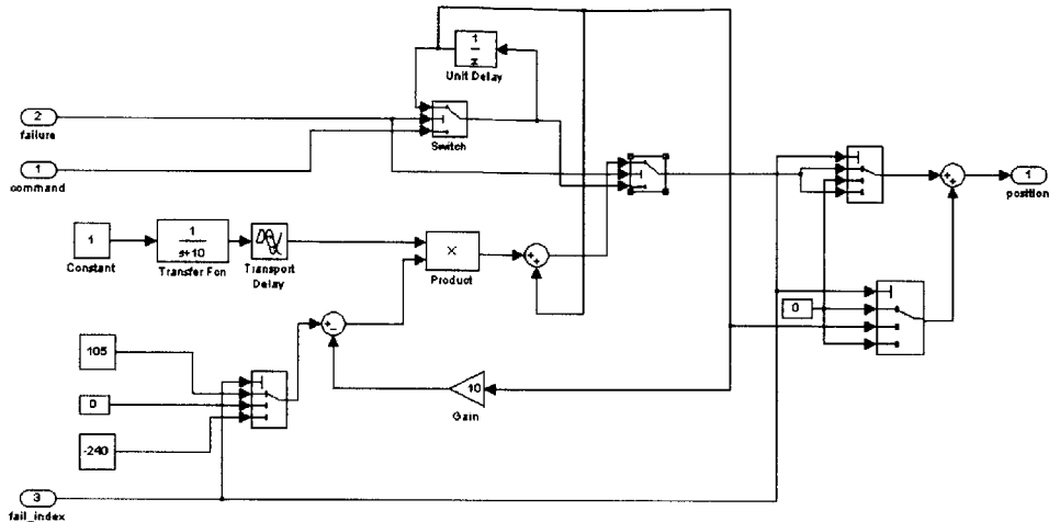
Figure 47: Failure Implementation
