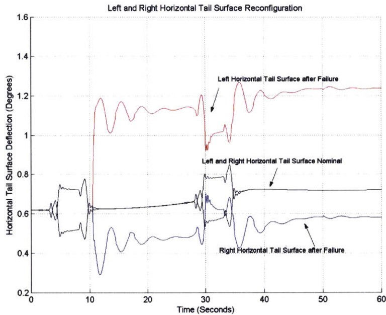
Figure 71: Horizontal Tail Reconfiguration
