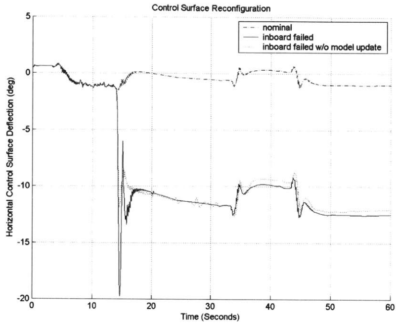
Figure 52: Control Surface Reconfiguration
