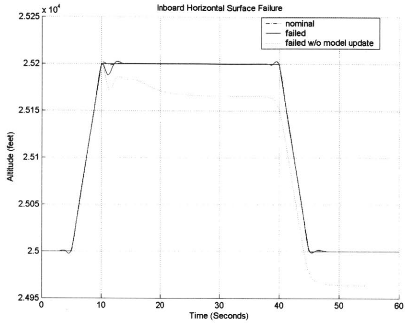
Figure 75: Hardover Inboard Horizontal Tail Surface Failure Reconfiguration with Relaxed Constraints
