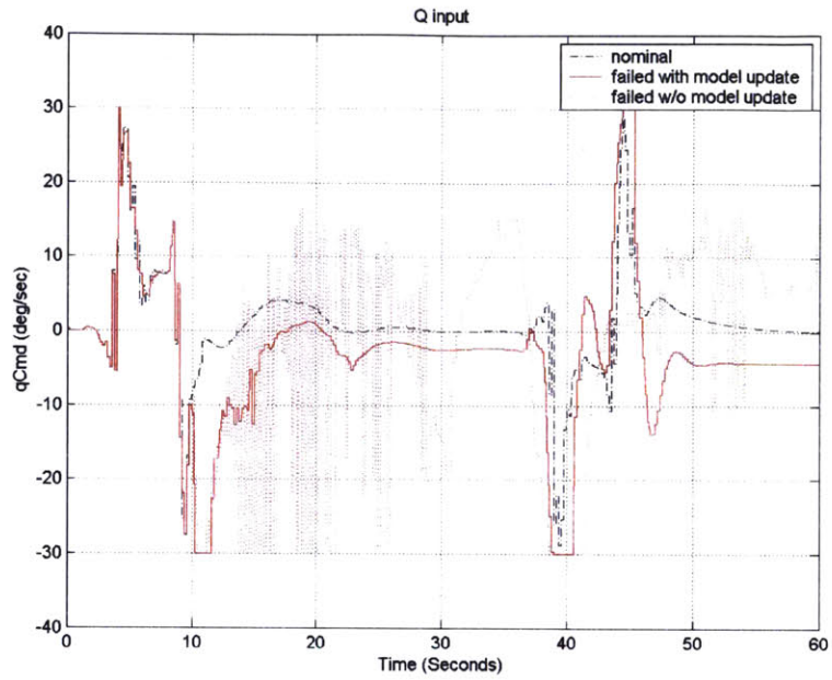
Figure 102: Pitch Rate Command for Hardunder Inboard Horizontal Tail Surface Failure Controller Reconfiguration
