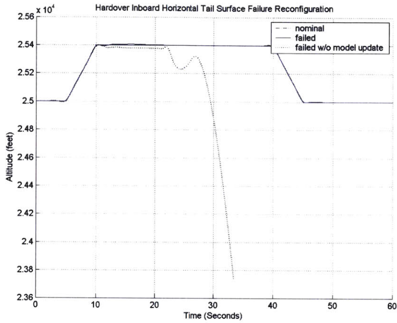
Figure 94: Hardover Inboard Horizontal Tail Surface Failure Reconfiguration
