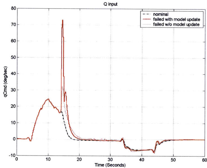
Figure 50: Pitch Controller Reconfiguration
