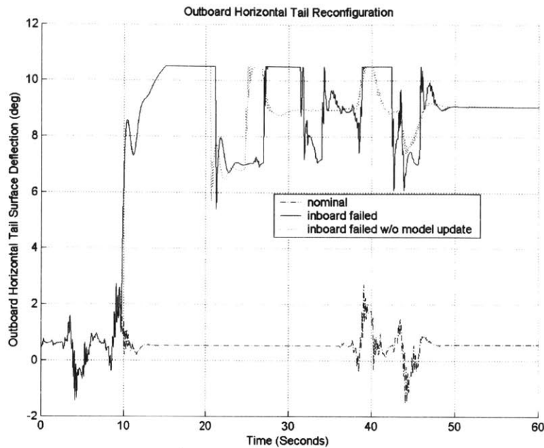
Figure 81: Outboard Horizontal Tail Surface Reconfiguration
