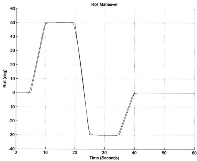
Figure 25: Bank Hold
