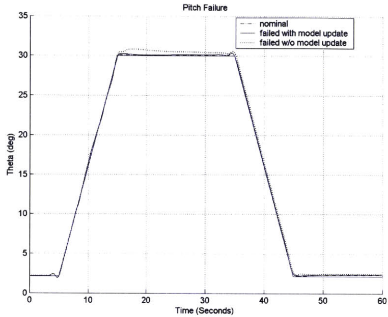
Figure 57: Pitch Frozen Reconfiguration
