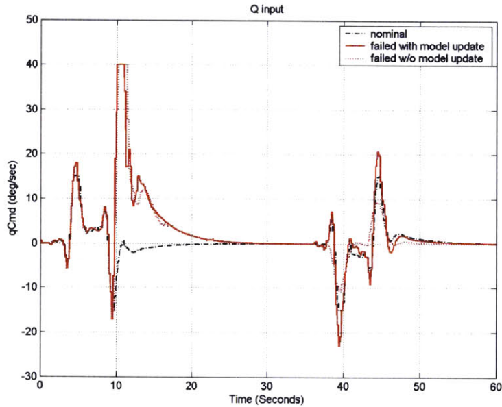
Figure 77: Pitch Rate Command for Hardover Inboard Horizontal Tail Surface Controller Reconfiguration
