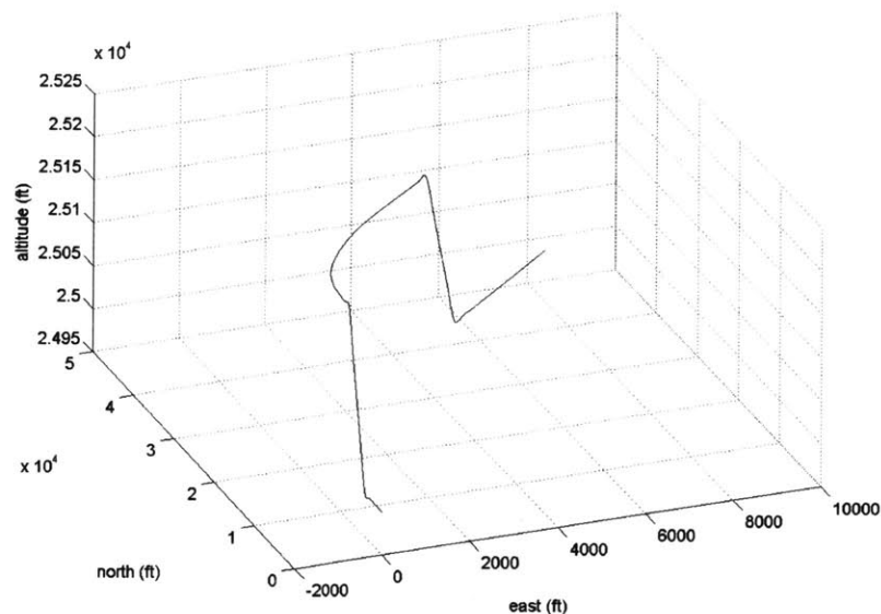
Figure 17: Sample Flight Path
