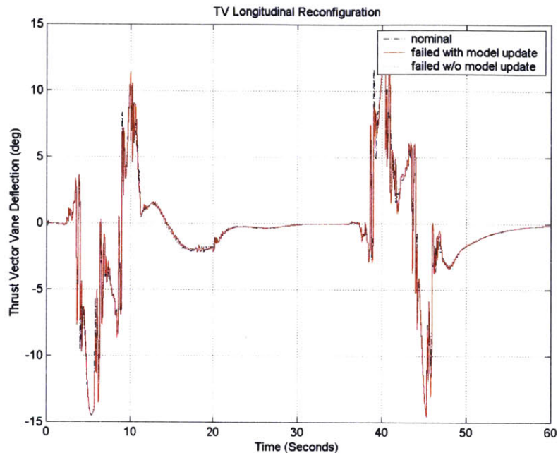
Figure 93: Frozen Rudder Thrust Vane Reconfiguration
