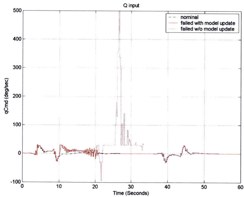
Figure 95: Pitch Rate Command for Hardover Inboard Horizontal Tail Surface Failure Controller Reconfiguration
