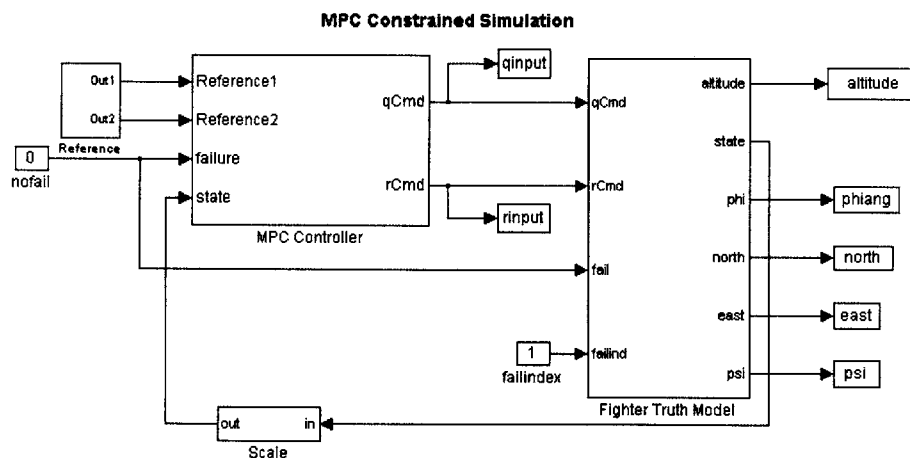
Figure 18: MPC Outer Loop
