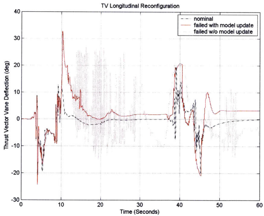
Figure 103: Hardunder Inboard Horizontal Tail Surface Failure Thrust Vector Reconfiguration
