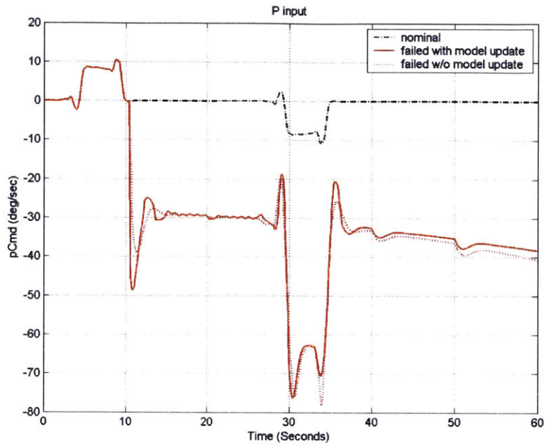
Figure 63: Roll Rate Command for Hardover Outboard Left Aileron Controller Reconfiguration
