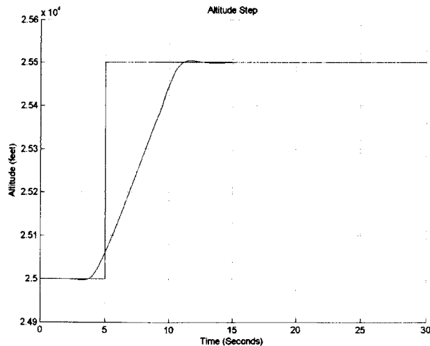
Figure 32: Altitude Step with Rate Constraint
