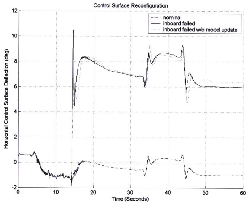
Figure 56: Pitch Hard Under Control Surface Reconfiguration
