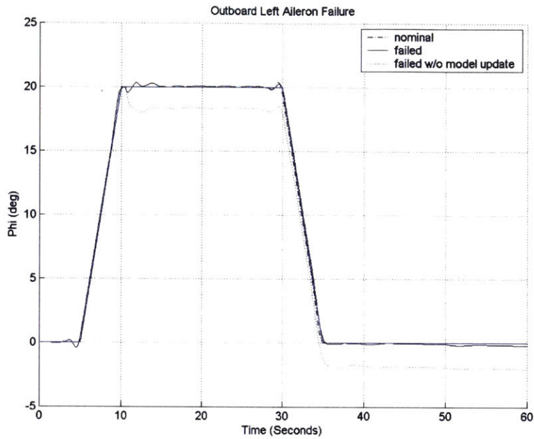
Figure 67: Outboard Left Aileron Hardunder Failure Reconfiguration
