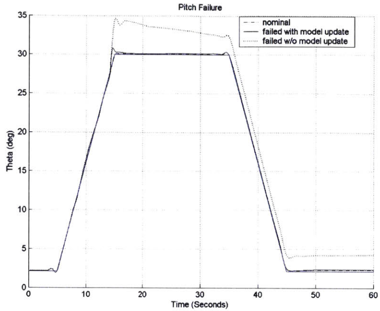
Figure 53: Pitch Hard Under Reconfiguration
