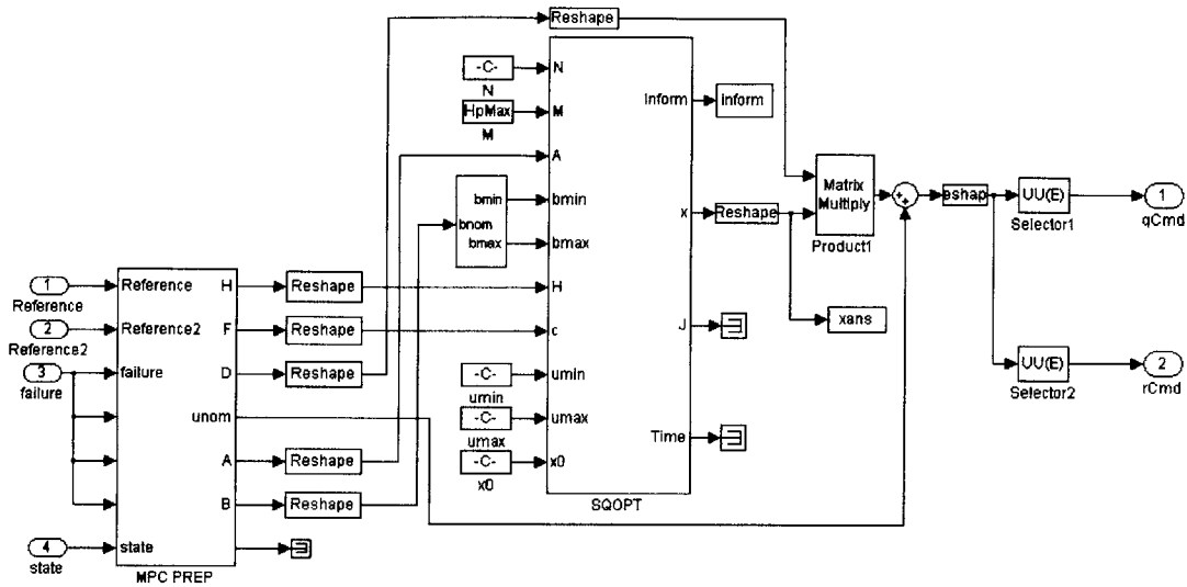
Figure 19: MPC Controller Structure
