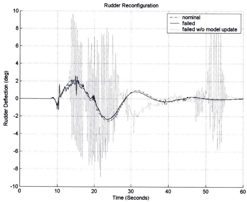
Figure 108: Rudder Reconfiguration
