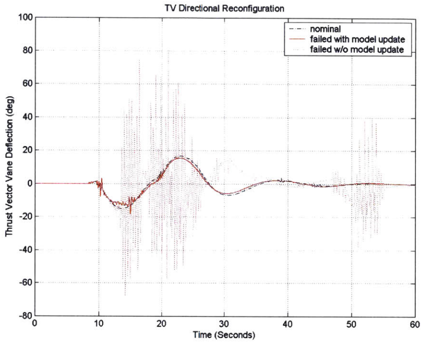
Figure 107: Hardunder Inboard Horizontal Tail Surface Failure Thrust Vector Reconfiguration
