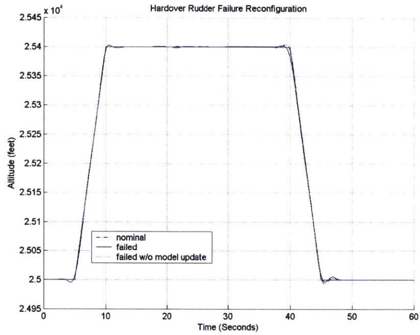
Figure 85: Altitude/Rudder Hardover Reconfiguration
