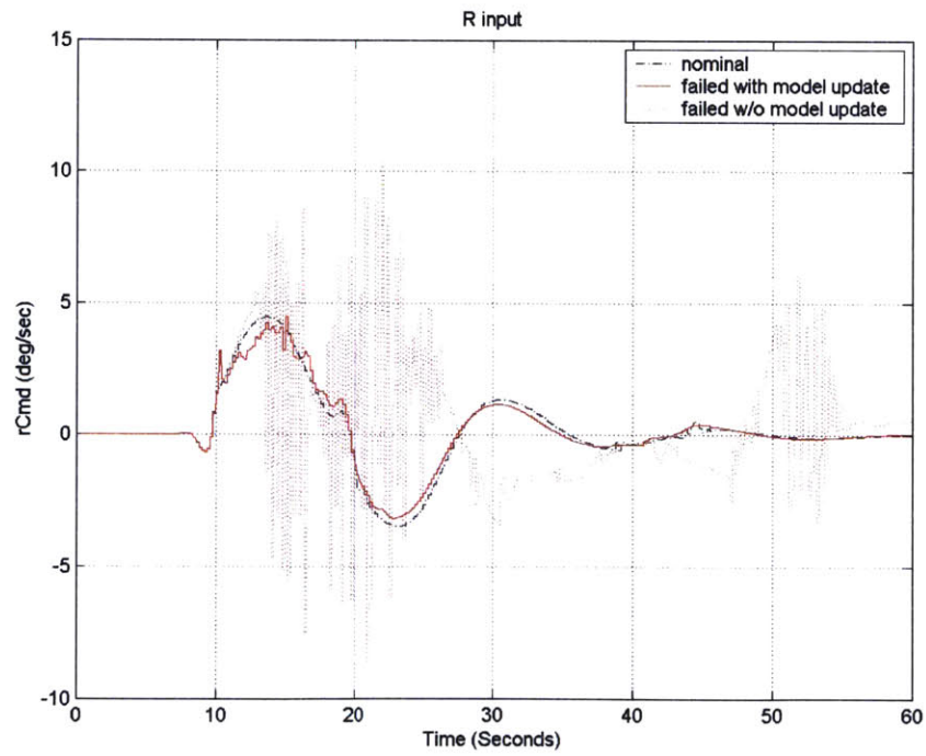
Figure 106: Yaw Rate Command for Hardunder Inboard Horizontal Tail Surface Failure Controller Reconfiguration
