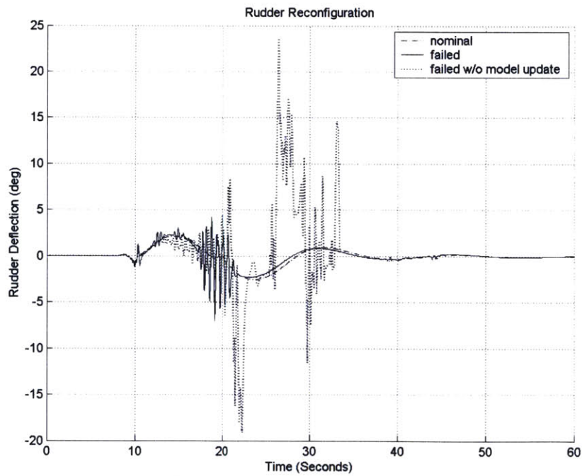
Figure 97: Hardover Inboard Horizontal Tail Surface Failure Rudder Reconfiguration
