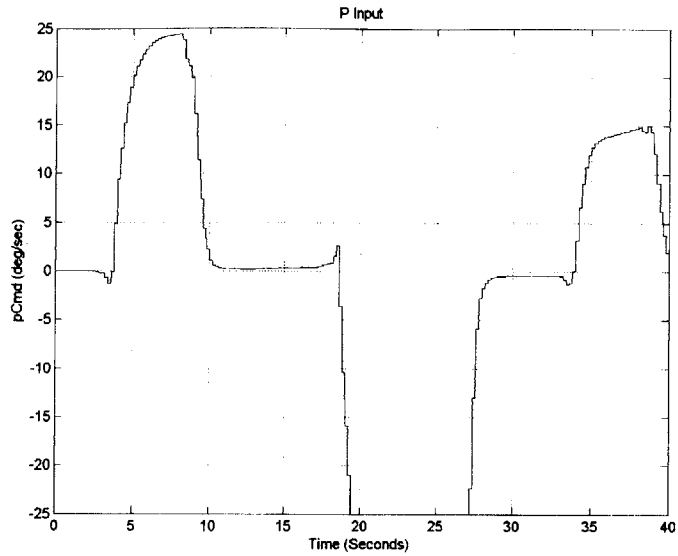
Figure 28: Bank Hold Input
