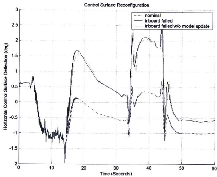
Figure 60: Pitch Frozen Horizontal Tail Reconfiguration
