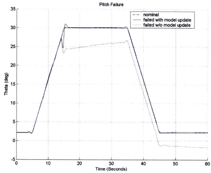
Figure 48: Pitch Failure
