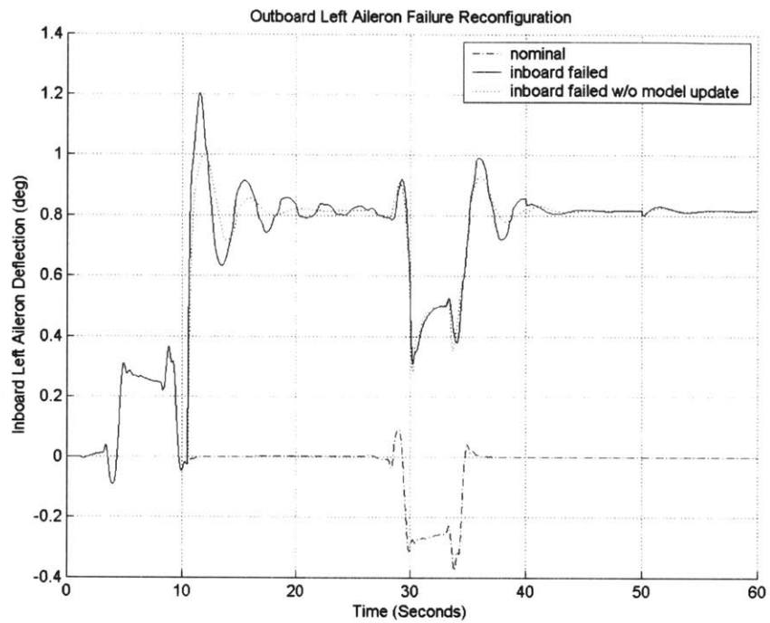
Figure 69: Hardunder Outboard Left Aileron Failure Reconfiguration
