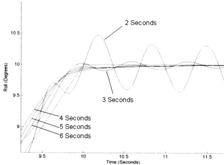
Figure 9: Prediction Horizon Comparison
