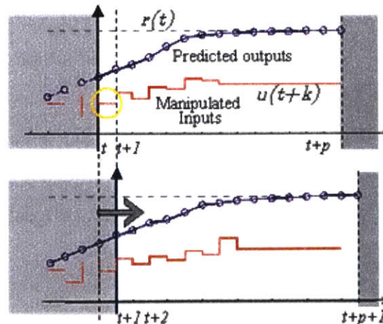
Figure 2: MPC Receding Horizon Graphic
