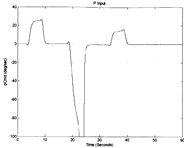
Figure 26: P Input
