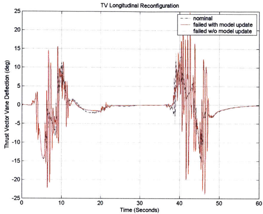
Figure 87: Altitude/Rudder Hardover Thrust Vane Reconfiguration
