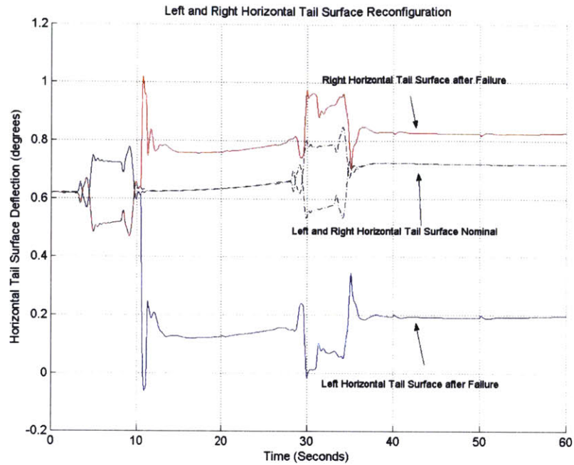
Figure 66: Horizontal Tail Reconfiguration
