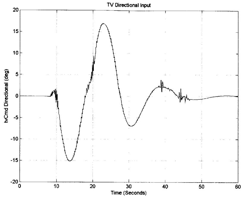
Figure 40: TV Directional Command
