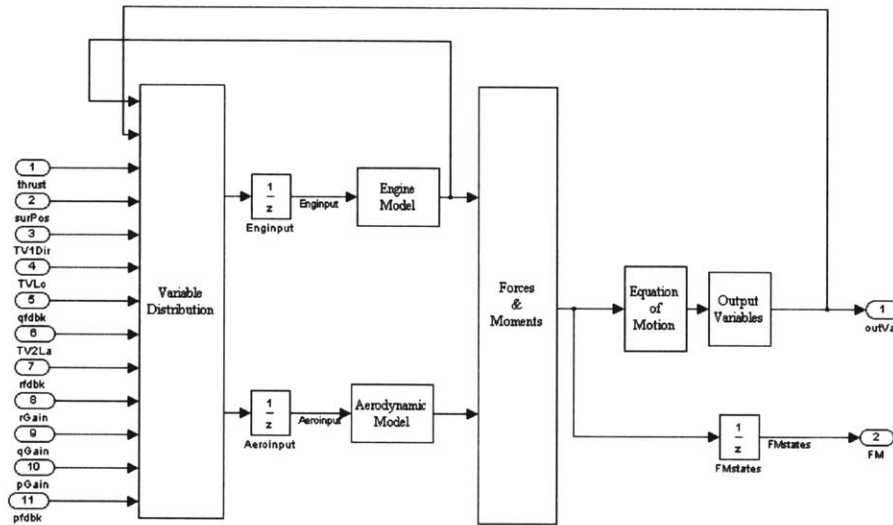
Figure 111: Aircraft Airframe with Delays
