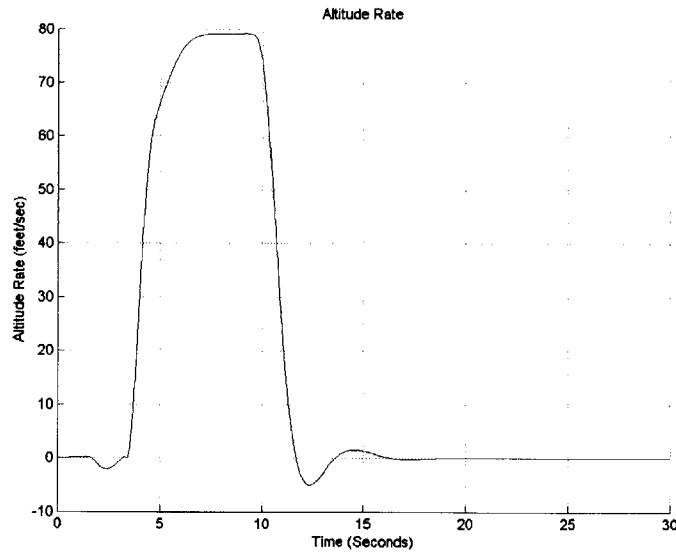
Figure 34: Altitude Rate for Altitude Step with Rate Constraint
