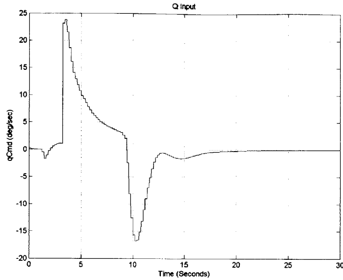
Figure 33: Pitch Rate Command for Altitude Step with Rate Constraint
