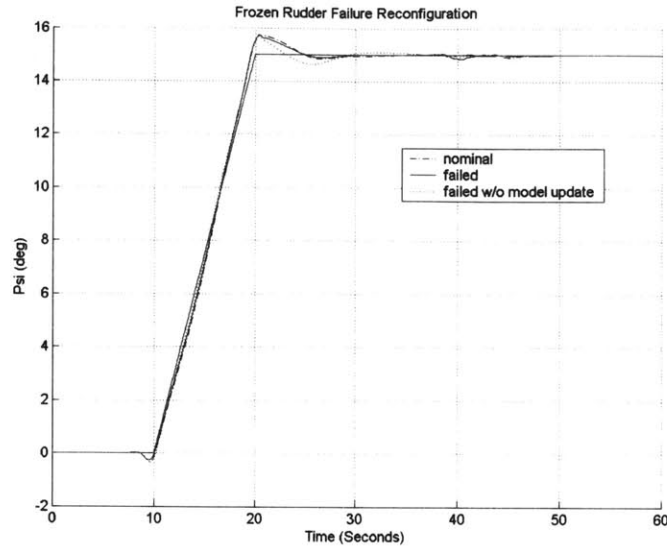
Figure 88: Frozen Rudder Failure Reconfiguration
