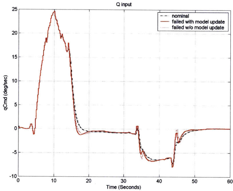
Figure 59: Pitch Frozen Controller Reconfiguration
