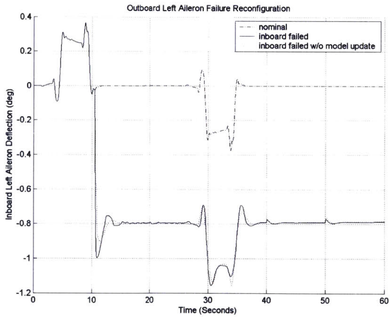
Figure 64: Hardover Outboard Left Aileron Failure Reconfiguration
