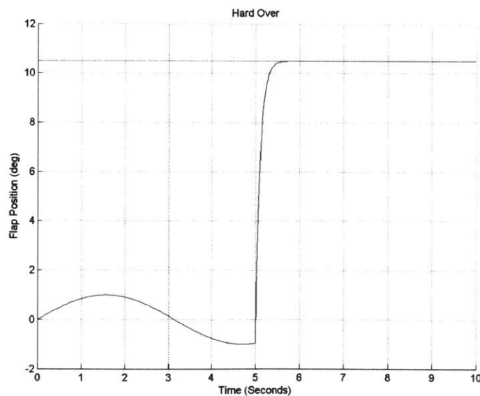
Figure 44: Hard Over Demonstration
