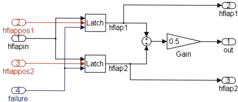
Figure 43: Control Surface Split
