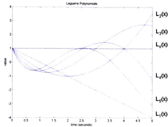
Figure 20: Laguerre Polynomials
