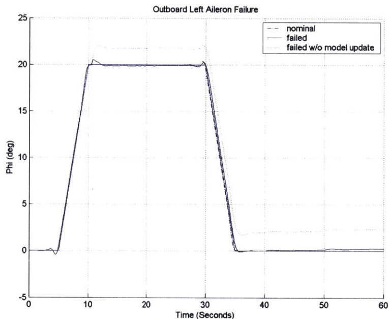
Figure 61: Outboard Left Aileron Hardover Failure Reconfiguration
