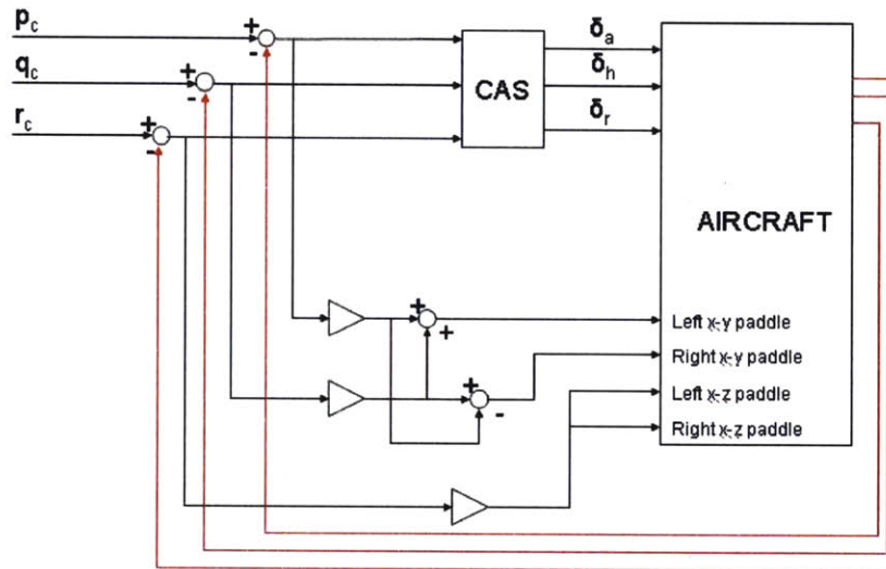
Figure 16: Thrust Vectoring Control
