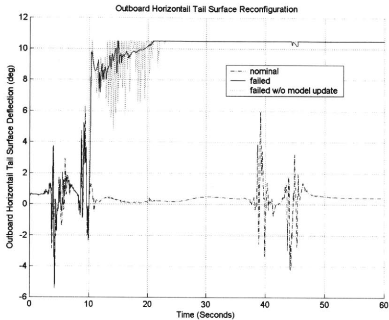
Figure 104: Outboard Horizontal Tail Surface Reconfiguration
