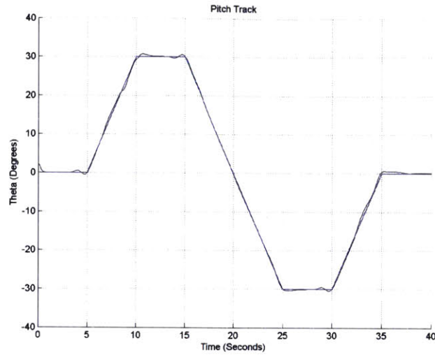
Figure 23: Pitch Doublet
