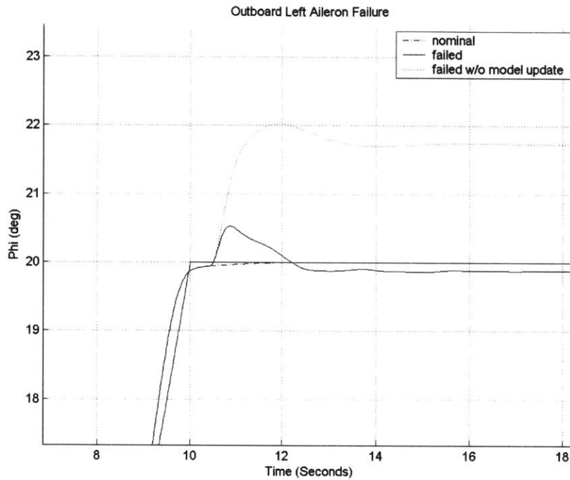
Figure 62: Hardover Outboard Left Aileron Failure Reconfiguration Zoom
