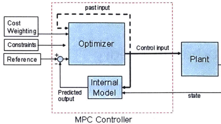
Figure 1: MPC Graphical Layout
