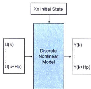
Figure 3: Nonlinear Propagator
