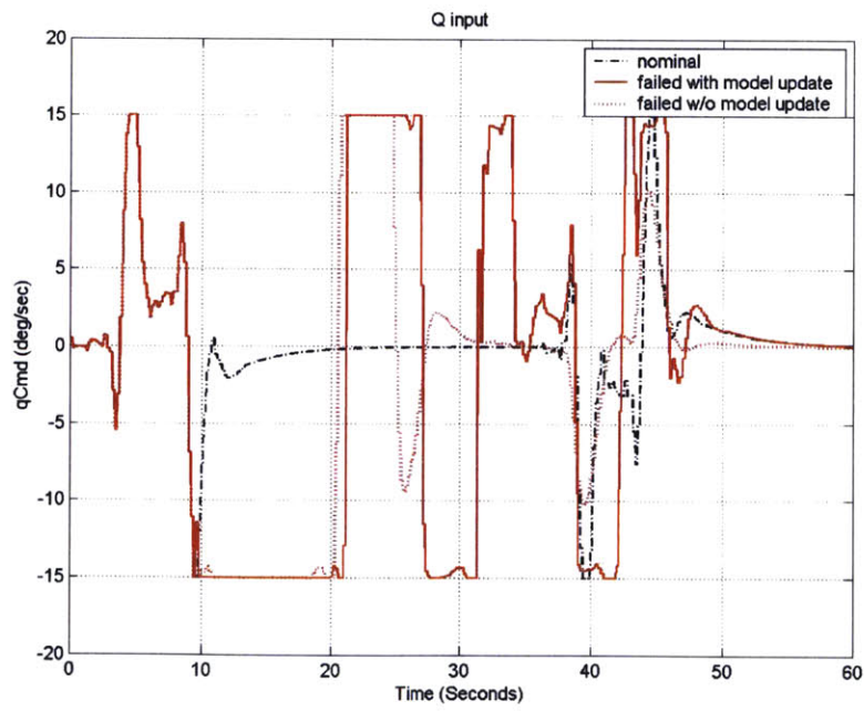
Figure 80: Pitch Rate Command for Hardunder Inboard Horizontal Tail Surface Controller Reconfiguration
