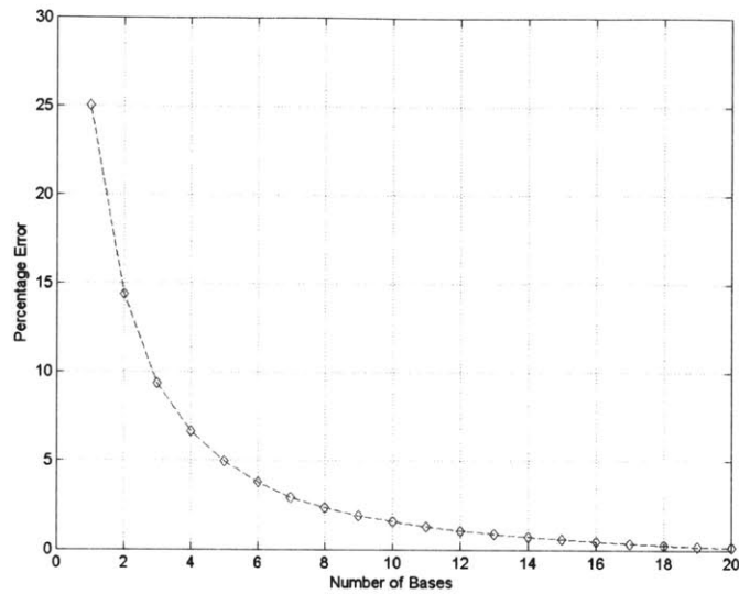
Figure 7: Basis Percentage Error
