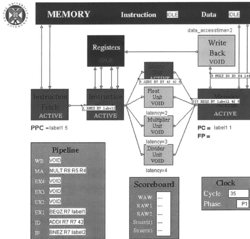
Figure 1-2: HASE Applet Used To Demonstrate A DLX Processor with Scoreboarding
