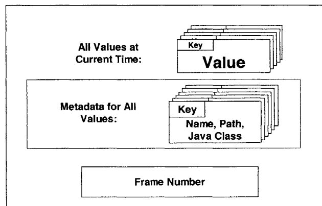
Figure 3-4: Diagram of an Image Object
