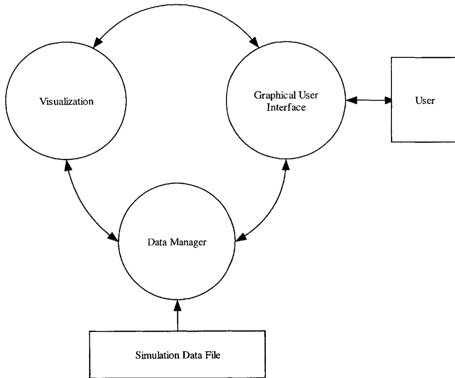
Figure 2-5: Conceptual Component Model of the VISTA Environment
