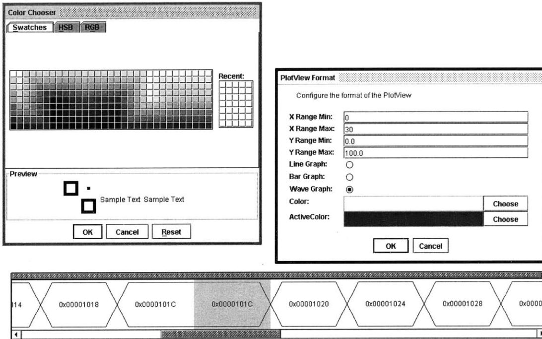
Figure 5-8: A Plot View Object with a Property Box and Color Chooser
