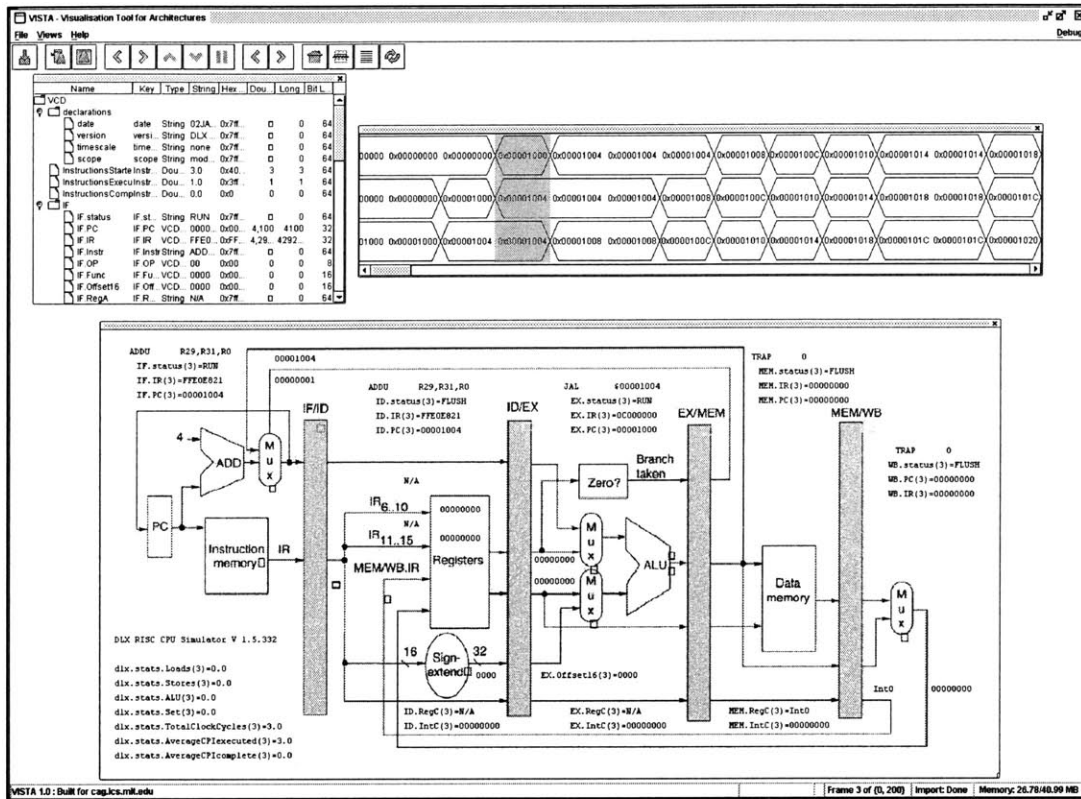
Figure 5-1: The Graphical User Interface of the VISTA Environment
