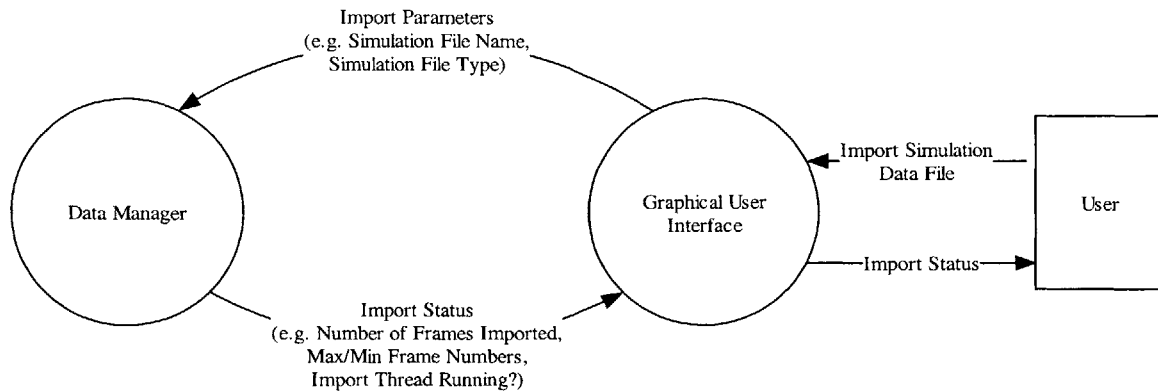
Figure 2-6: Interface Between GUI and Importing and Managing Simulation Data Components
