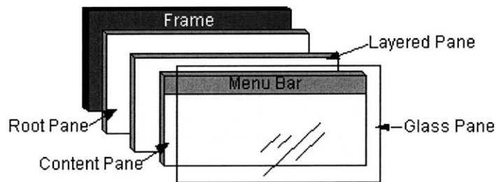
Figure 5-3: The Structure of a Top-Level Container
