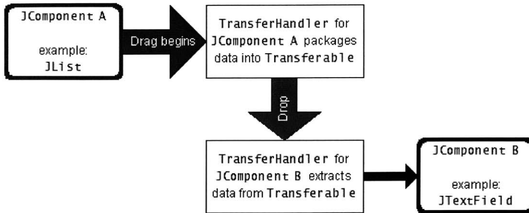
Figure 5-4: The Use of Swing Transfer Handlers in Drag and Drop
