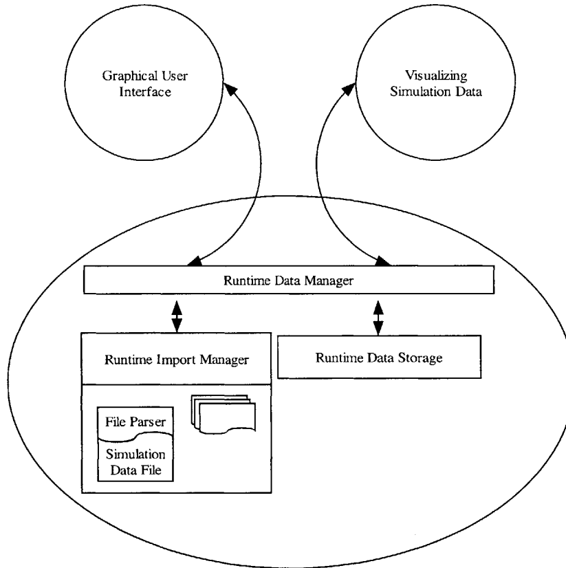
Figure 2-9: Conceptual Model of the Components of Data Components
