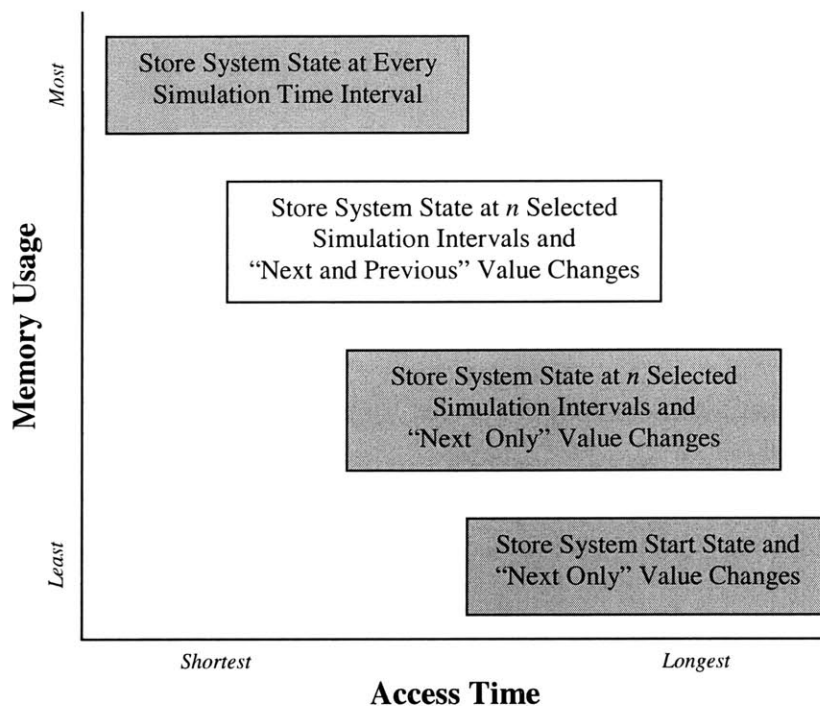
Figure 2-4: The Memory and Access Time Cost of Various Value Change Schemes
