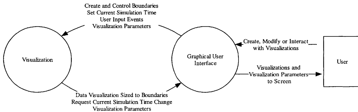
Figure 2-7: Interface Between the GUI and the Visualization
