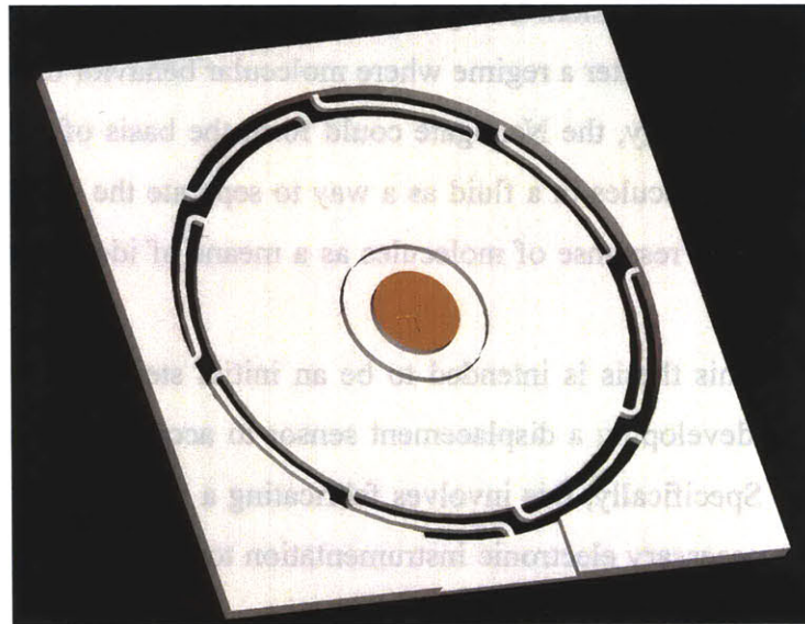
Figure 2: CAD model of the Nanogate silicon diaphragm
