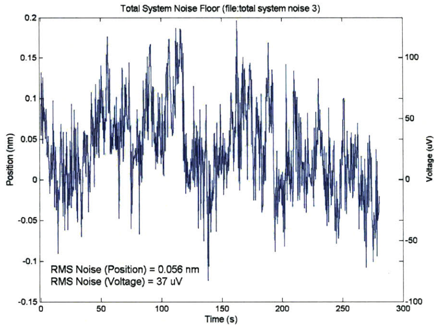
Figure 28: Noise waveform of the full differential capacitive sensing circuit
