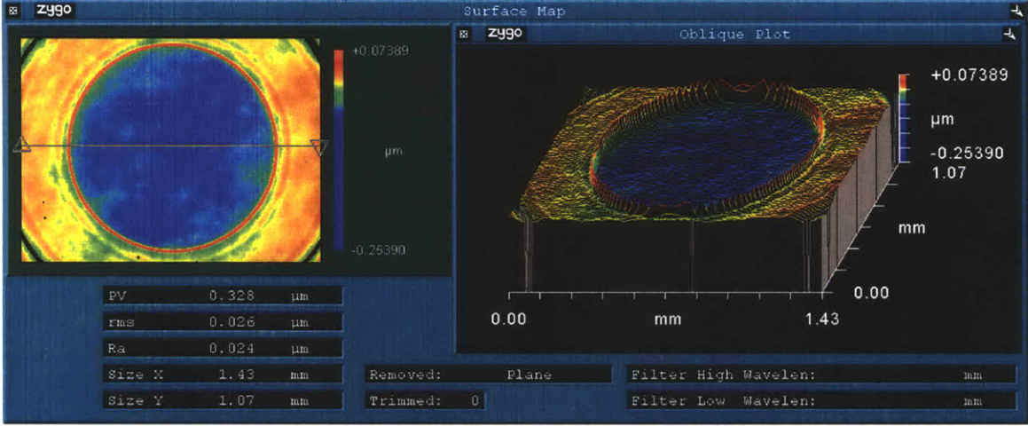
Figure 10: Profilometer scan of the Pyrex wafer after bonding. The reflow of the Pyrex wafer can be seen conforming to the shape of the silicon valveland. The remains of the fulcrum can be seen at the corners.
