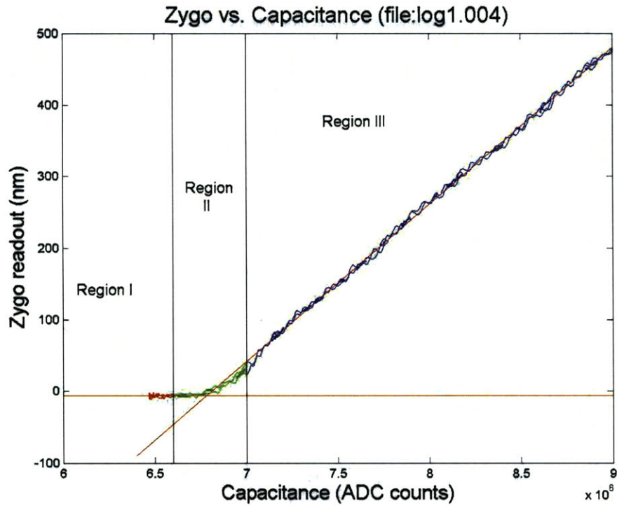
Figure 25: Zygo vs. Capacitance divided into 3 regions
