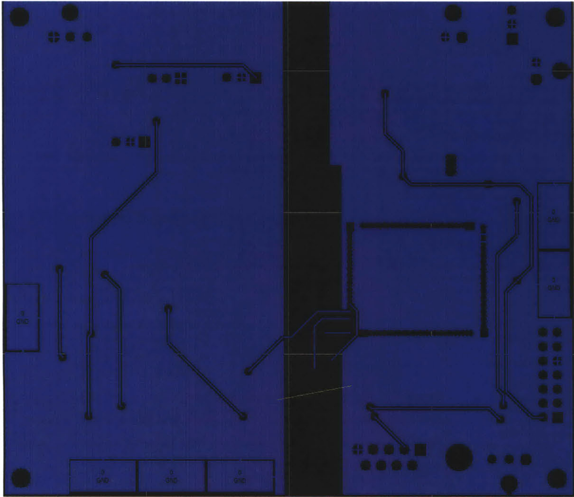
Figure 43: Data acquisition PCB layout, bottom layer
