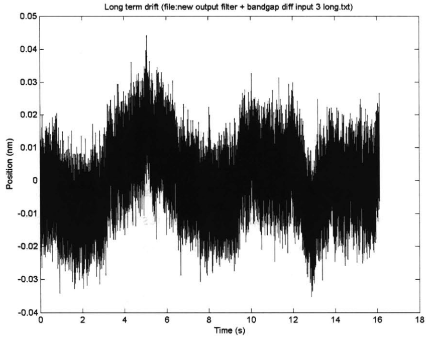
Figure 29: Drift from bandgap reference and output filter
