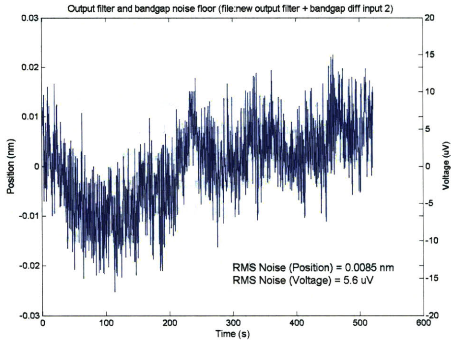
Figure 27: Noise waveform from the output filter and bandgap reference
