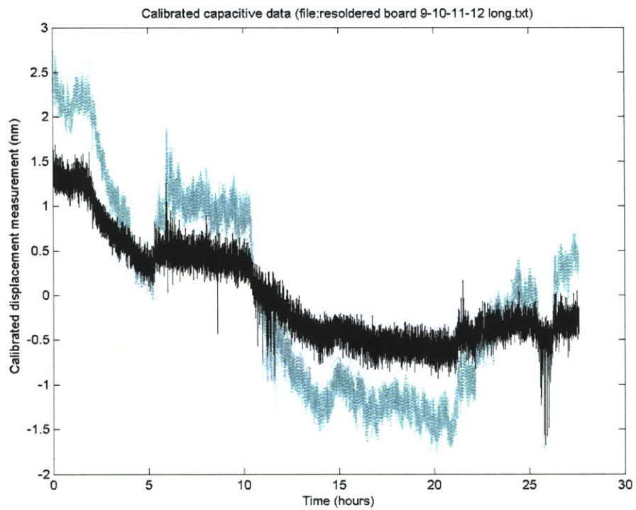
Figure 34: System output with calibration in the presence of external disturbances
