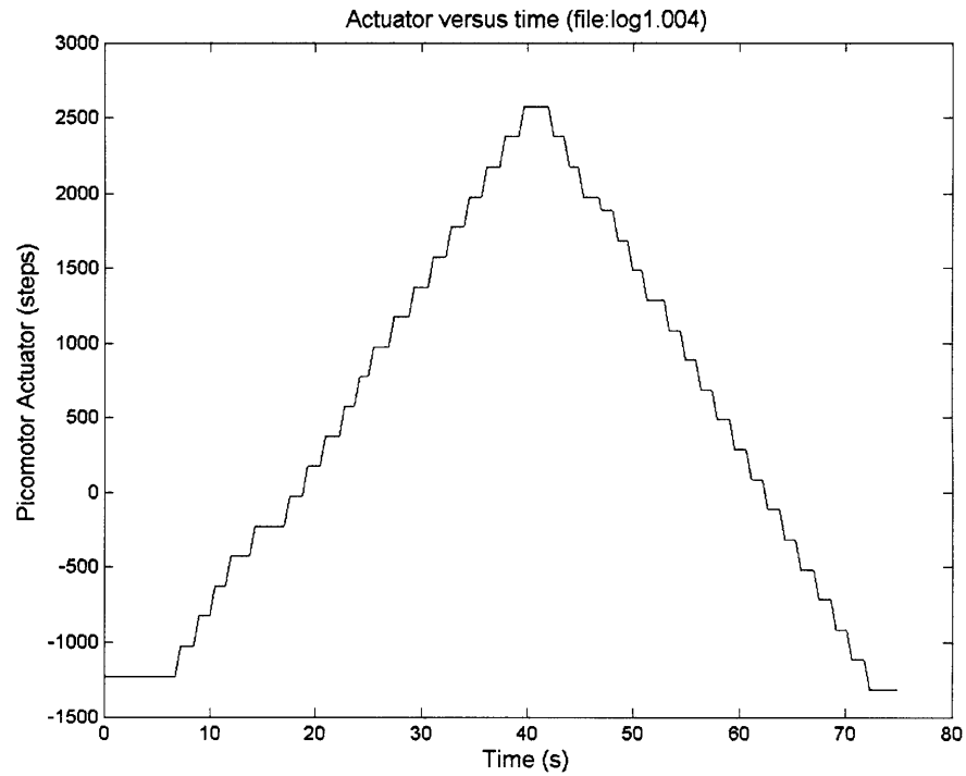
Figure 22: Actuator command versus time
