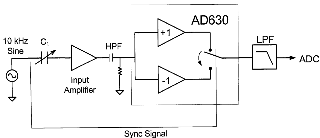
Figure 12: Capacitive sensing front-end
