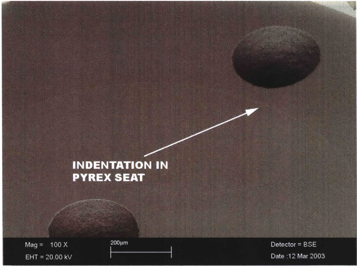
Figure 11: SEM of the Pyrex surface after bonding. The faint circle shows the indentation made by the silicon during the anodic bonding process.
