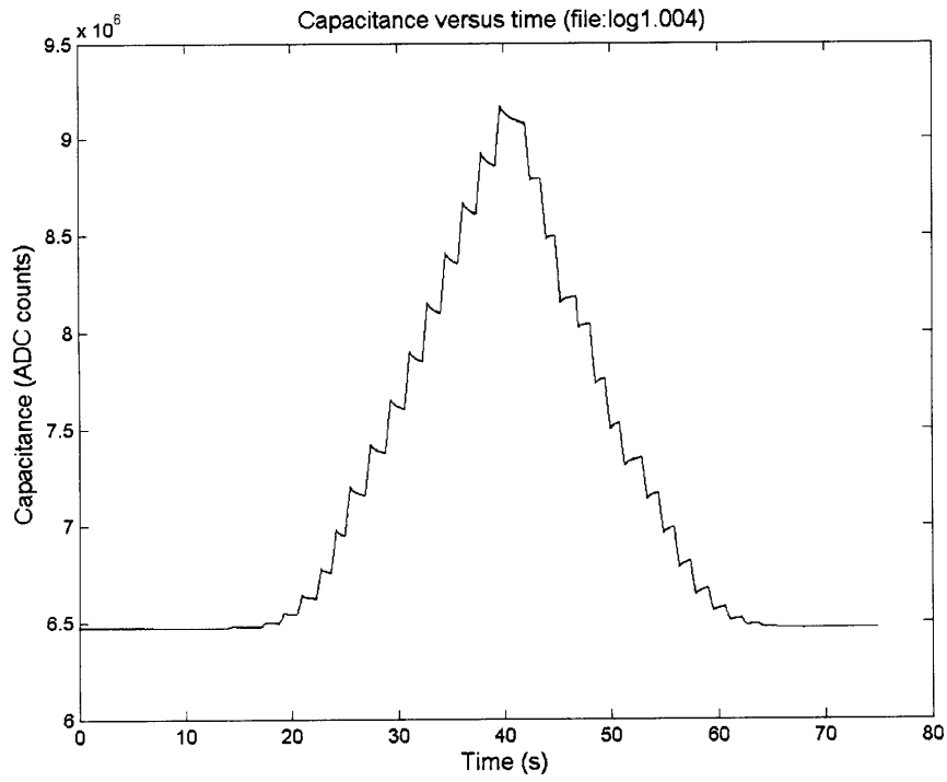
Figure 23: Capacitance output in ADC counts versus time
