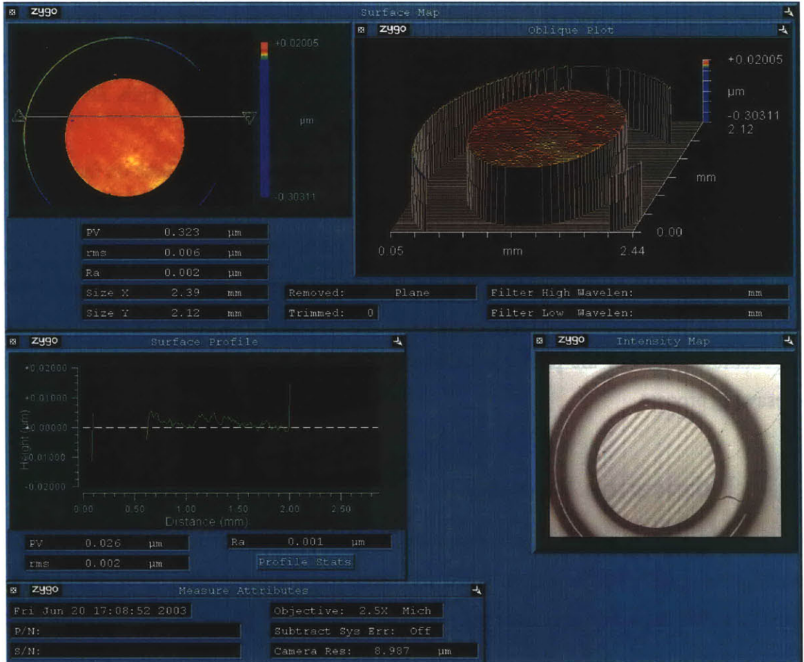
Figure 8: Profilometer scan of the silicon valveland showing 2nm rms surface roughness.
