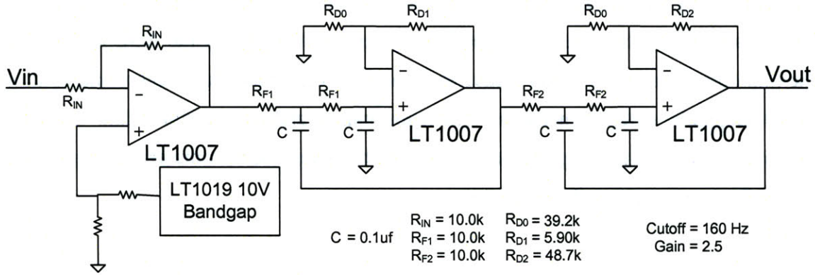
Figure 15: Level shifter and 4-pole VCVS low-pass filter
