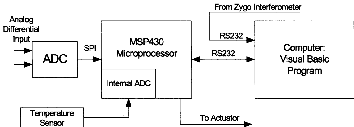
Figure 17: Data Acquisition System
