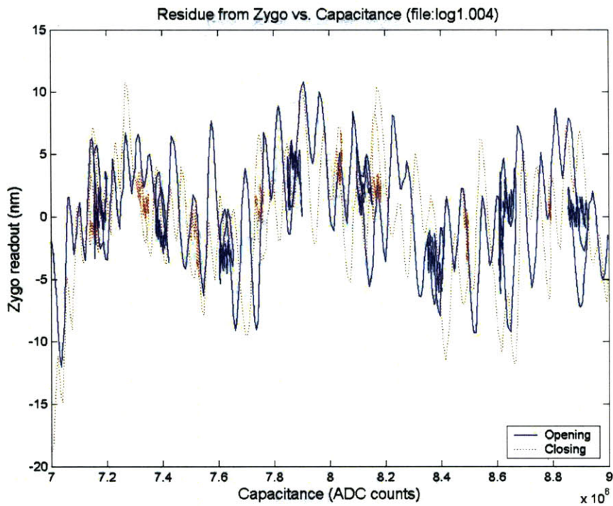
Figure 26: Residue plot of Zygo vs. Capacitance minus its linear fit line in region III of Figure 25
