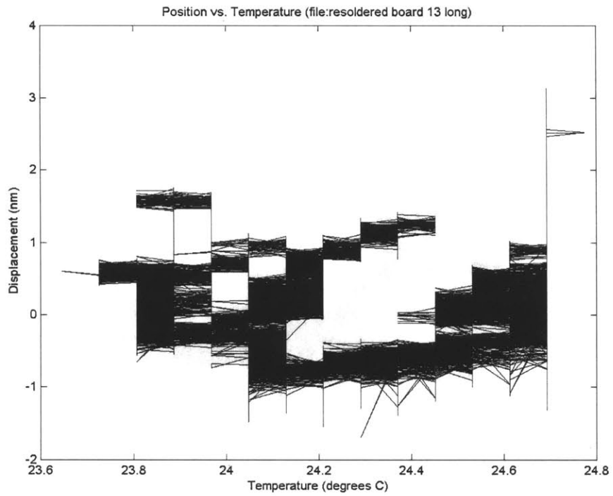
Figure 32: Temperature dependence of drift
