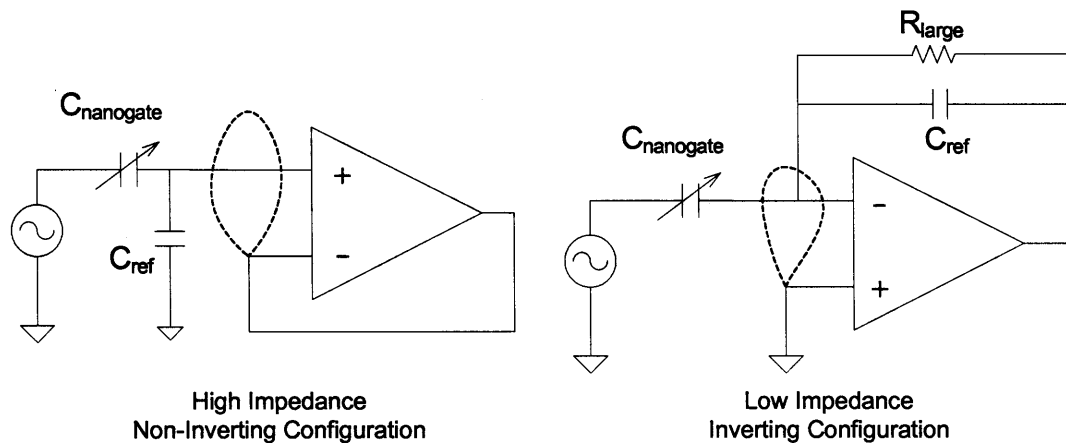
Figure 13: Input amplifier in high and low impedance configuration
