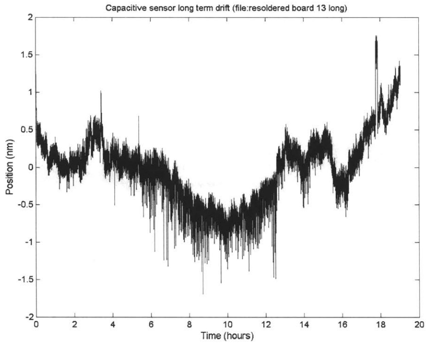
Figure 31: System output without calibration
