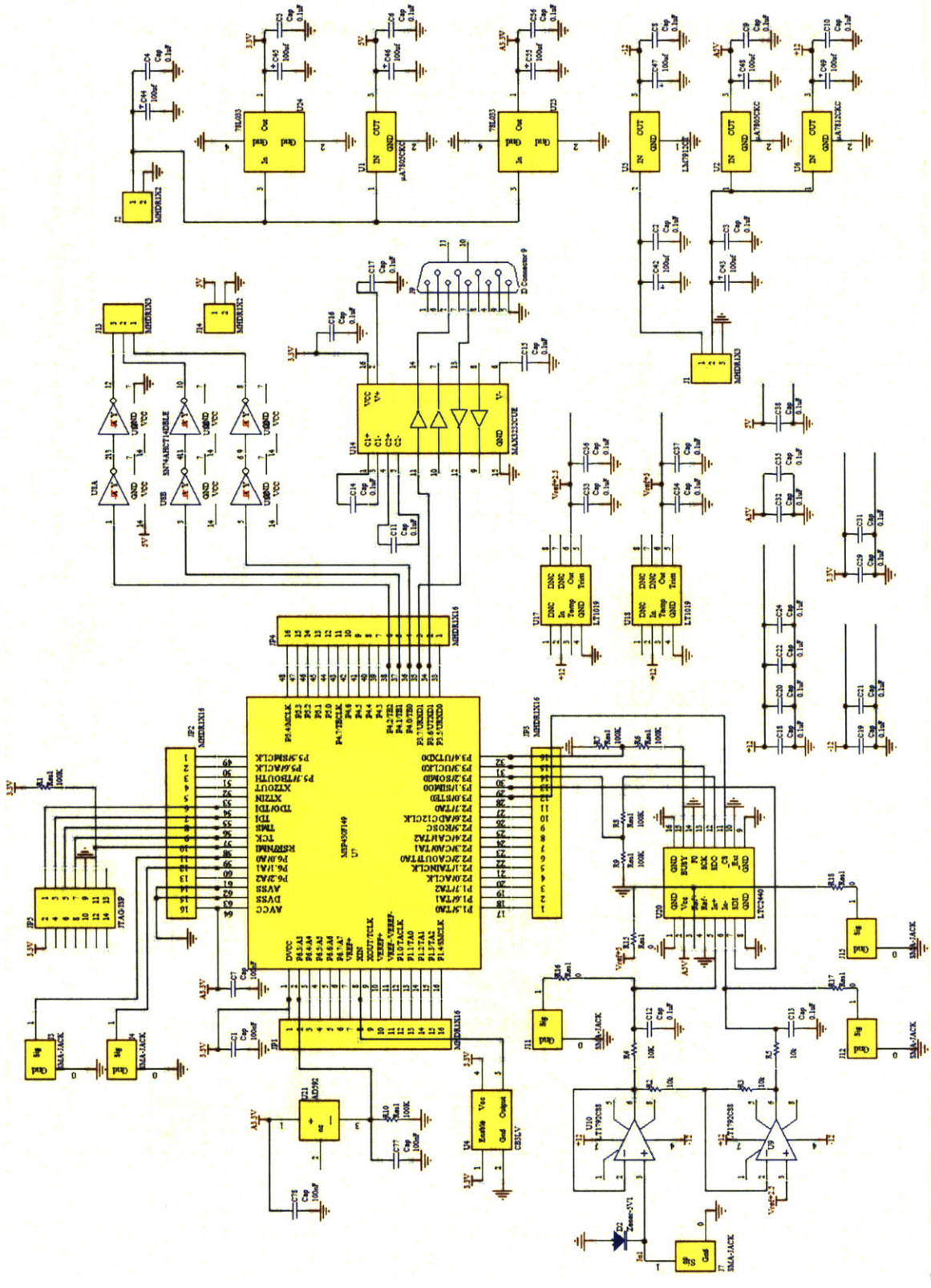
Figure 39: Data acquisition circuit full schematic
