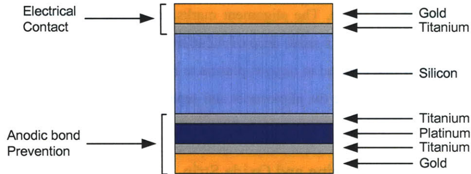
Figure 7: Metal Deposition on Silicon Wafer (not to scale)
