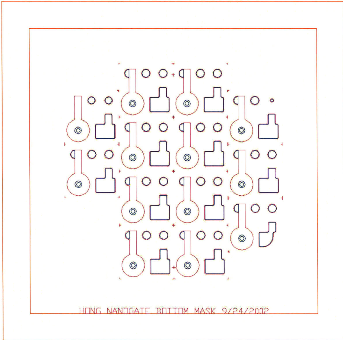
Figure 35: Mask for the Nanogate wafer bottom side (color inverted)
