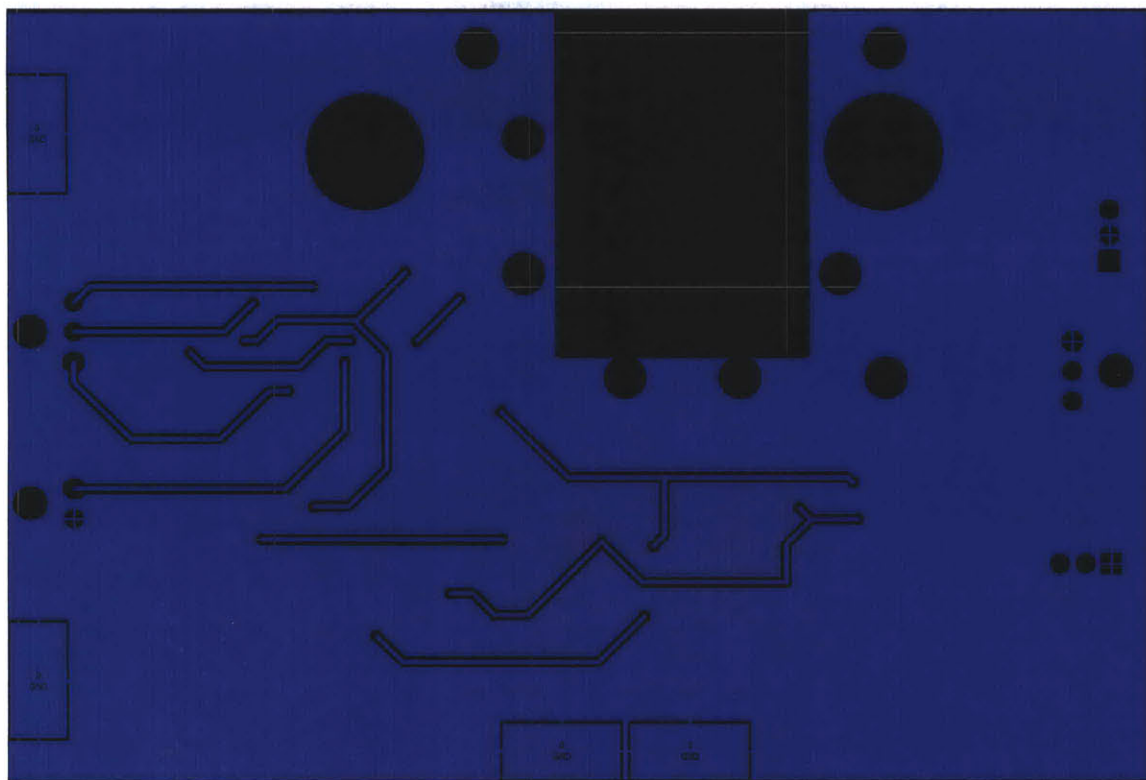
Figure 41: Analog front-end PCB layout, bottom layer
