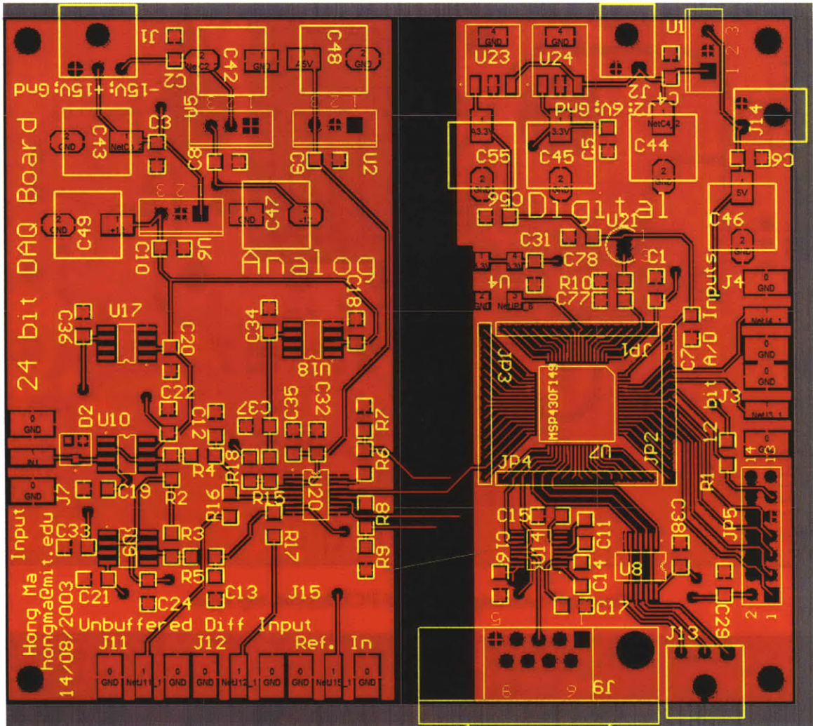
Figure 42: Data acquisition PCB layout, top layer
