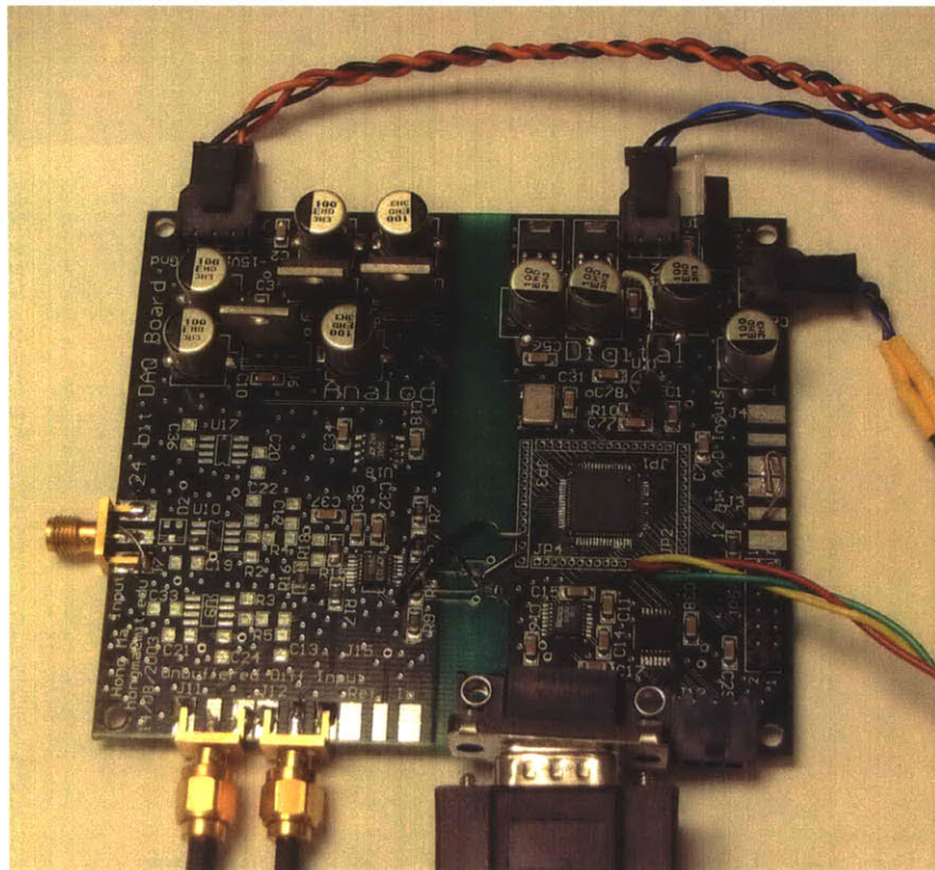
Figure 21: Photograph of the data acquisition PCB showing split ground planes for the ADC (left side) and microprocessor (right side)
