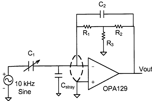
Figure 14: Input Amplifier Schematic
