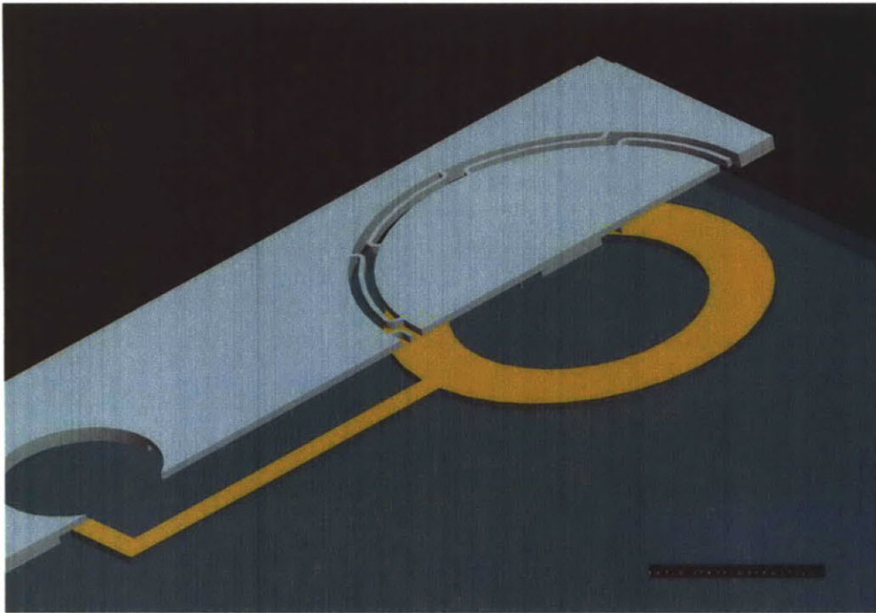
Figure 3: Cut-away diagram of the capacitive sensing electrodes. The silicon diaphragm is offset from the Pyrex diaphragm
