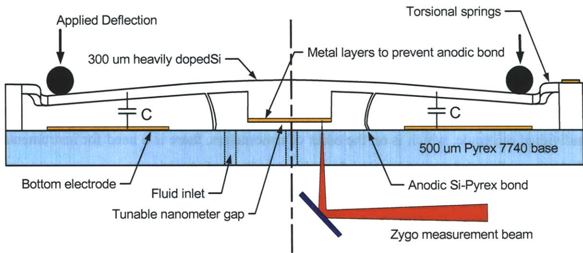
Figure 1: Cross section of the Nanogate with Added Capacitive Sensor Electrodes
