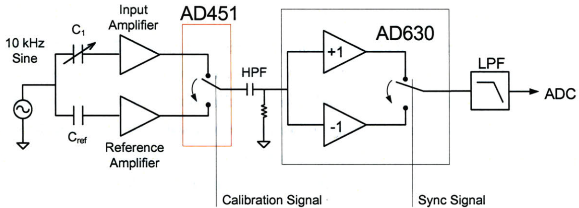
Figure 16: Switched calibration circuit
