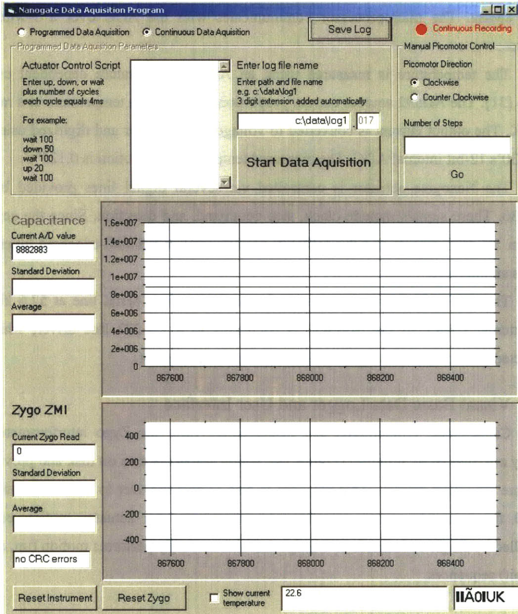
Figure 18: Screen-shot of the Visual Basic data collection and user interface program
