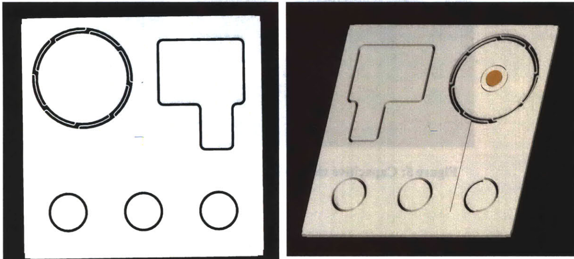
Figure 4: Nanogate die 3D model. Left: topview, Halo's are used to reduce etching time. Right: bottom view, a trench is designed to accommodate the capacitive electrodes on the Pyrex.
