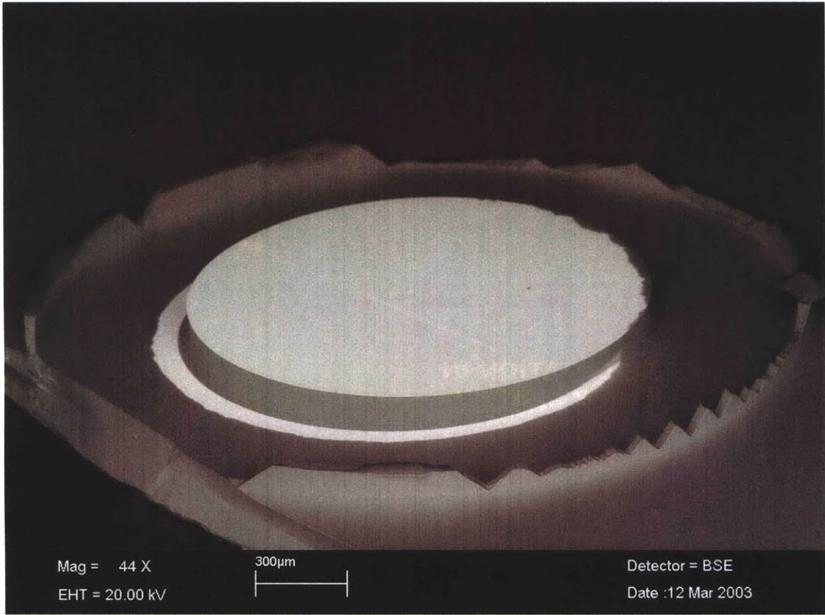
Figure 9: SEM Micrograph of the silicon diaphragm after the fulcrum is deliberately broken from the anodic bond with the Pyrex wafer
