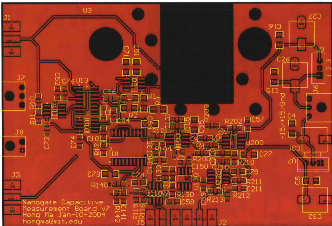
Figure 40: Analog front-end PCB layout, top layer
