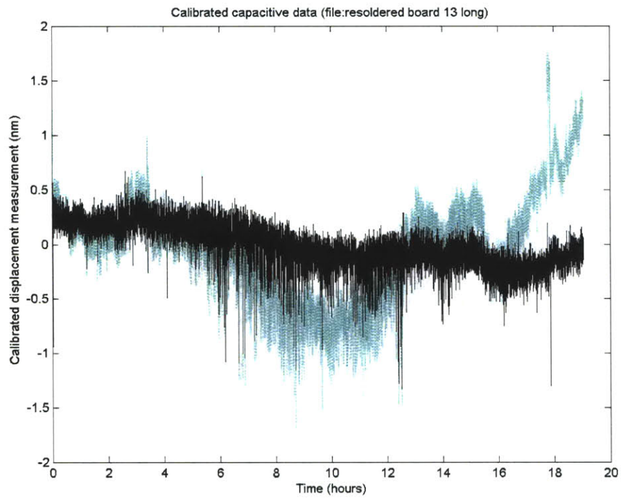
Figure 33: System output with calibration showing less than 1nm drift
