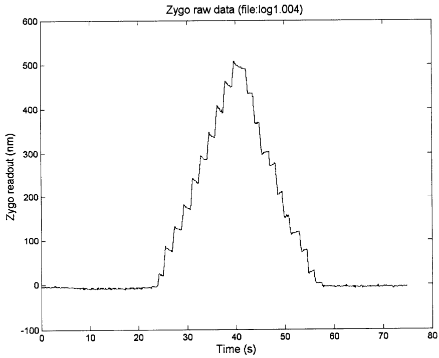
Figure 24: Zygo output versus time
