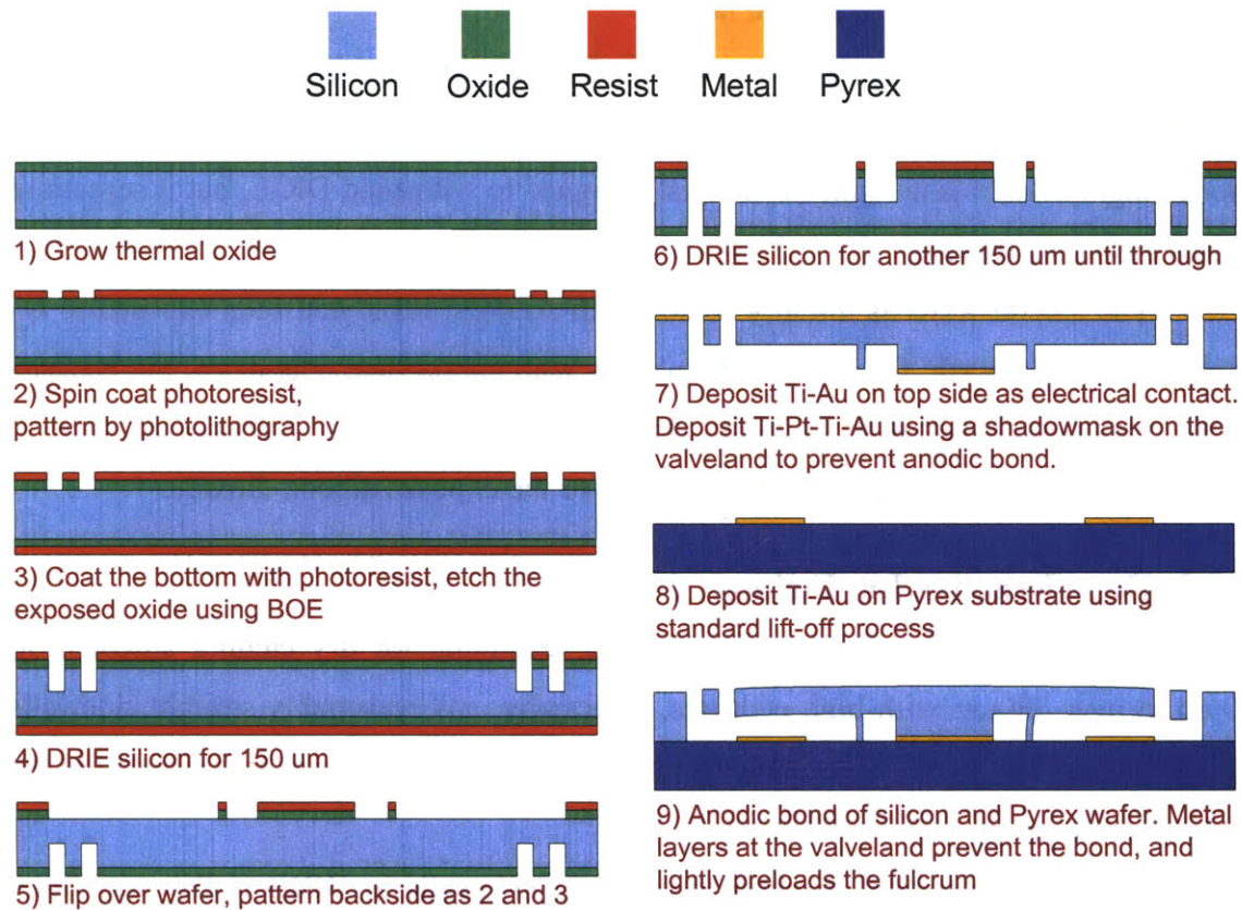
Figure 6: Outline of the Nanogate fabrication process, wafer shown in cross-section.
