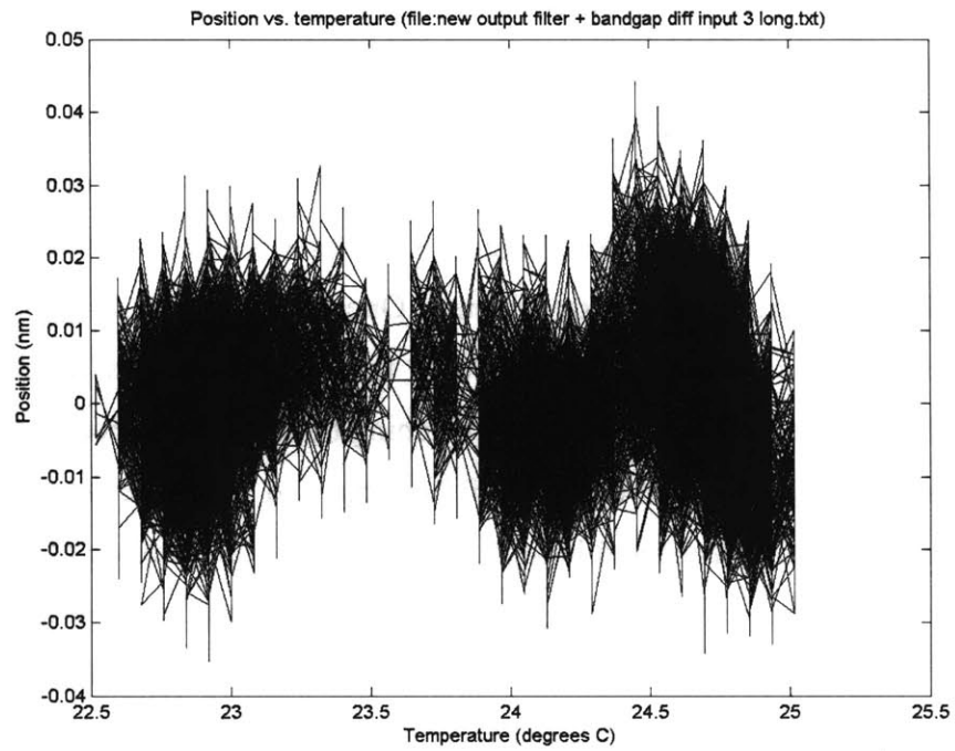
Figure 30: Temperature dependence of drift from bandgap reference and output filter
