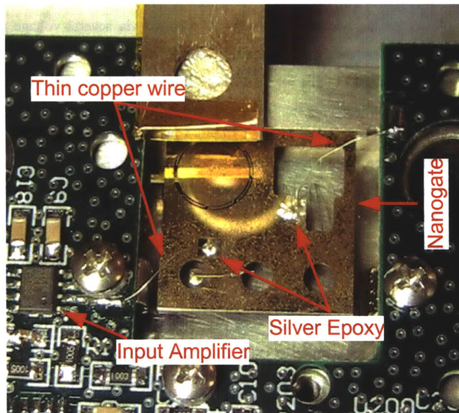
Figure 19: Electrical connection between capacitive electrodes and input amplifier
