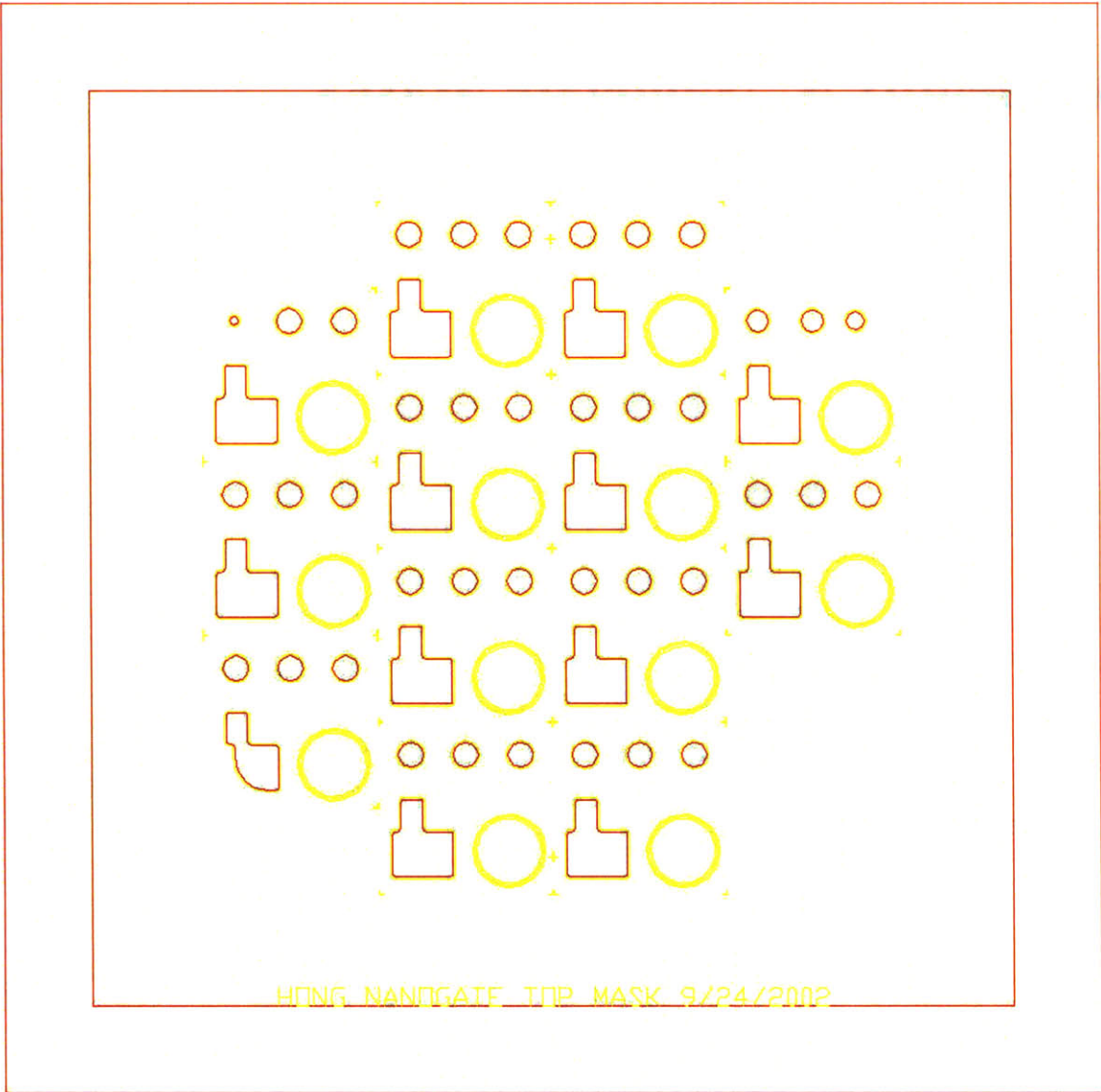
Figure 36: Mask for the Nanogate wafer top side (color inverted)
