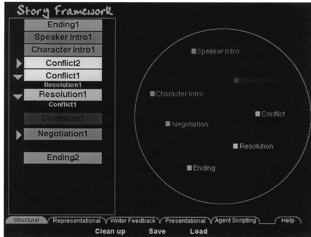
Fig. 20 A screen shot of the Structural Environment with a sample story framework. To build a story framework, the user drags the primitives in the circle across the screen and into the rectangle of the Story Framework.
