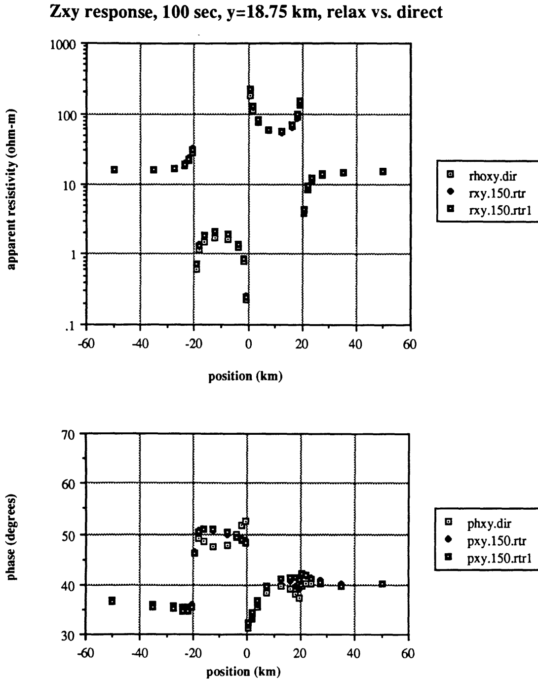
Figure 2-24. The Z_{xy} response along a profile at a strike position of y=18.75 km for a period of 100 seconds comparing the direct solution results with the results from both the MINRTRACC algorithm and the MINRTR algorithm, each time stopping after 150 iterations.
