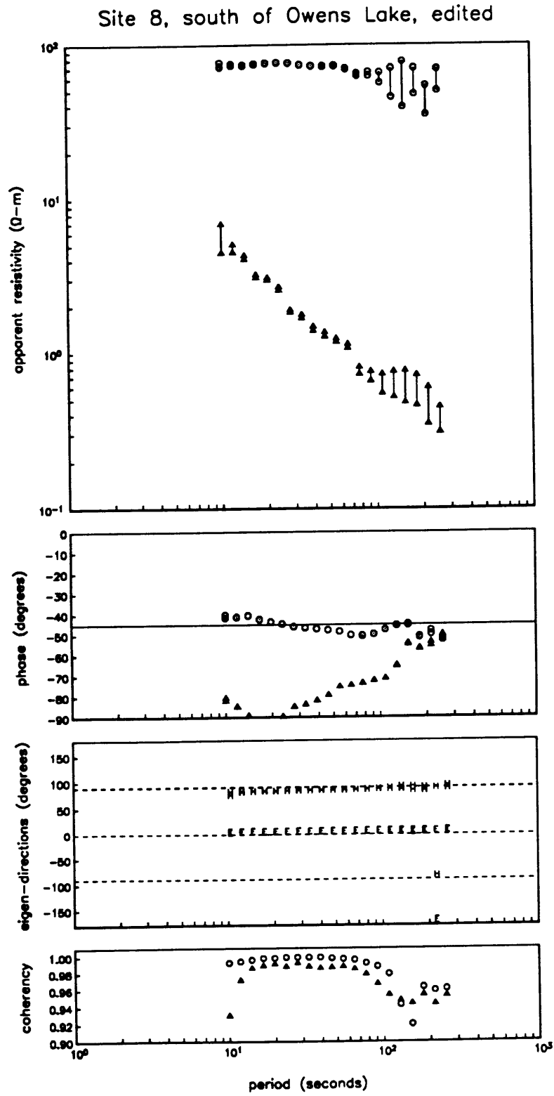
Figure 4-38. MT data after editing for site 8.
