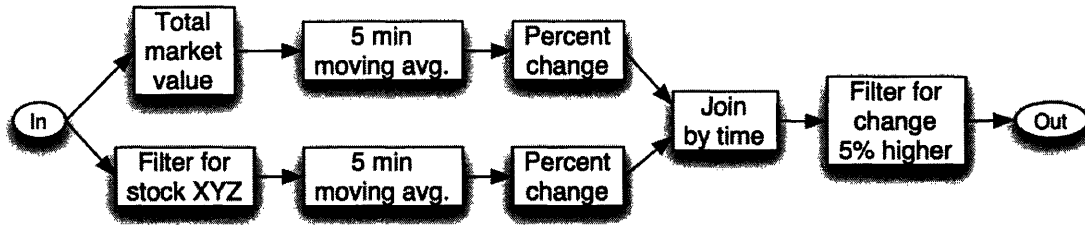
Figure 1-1: Example of an Aurora Query
