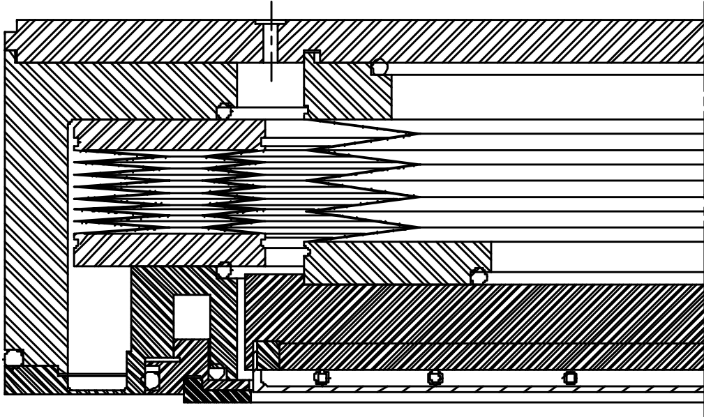
Figure 6-22: CAD assembly drawing of the wafer carrier showing the integration of leaf level DPs
