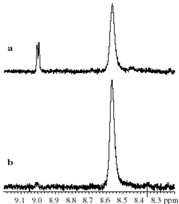
Figure 3.9. ^1\text{H} NMR spectra ( 0^\circ\text{C} , \text{C}_6\text{D}_5\text{Br} ) for the ortho pyridyl region after addition of 1-hexene to a solution of 37 activated with [\text{HNMe}_2\text{Ph}][\text{B}(\text{C}_6\text{F}_5)_4] a) after 1 h; b) initially.
