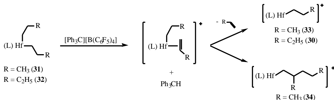
Scheme 3.4. Activation of 31 and 32 with [\text{Ph}_3\text{C}][\text{B}(\text{C}_6\text{F}_5)_4] ( 0^\circ\text{C} , \text{C}_6\text{D}_5\text{Br} ). \text{L} = [\text{MesNpy}]^{2-} , anion = [\text{B}(\text{C}_6\text{F}_5)_4]^- .
