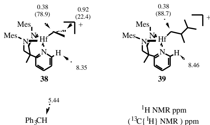
Figure 3.4. Species present in solution upon activation of 37 with [\text{Ph}_3\text{C}][\text{B}(\text{C}_6\text{F}_5)_4] ( -20\text{ }^\circ\text{C} , \text{C}_6\text{D}_5\text{Br} ).
