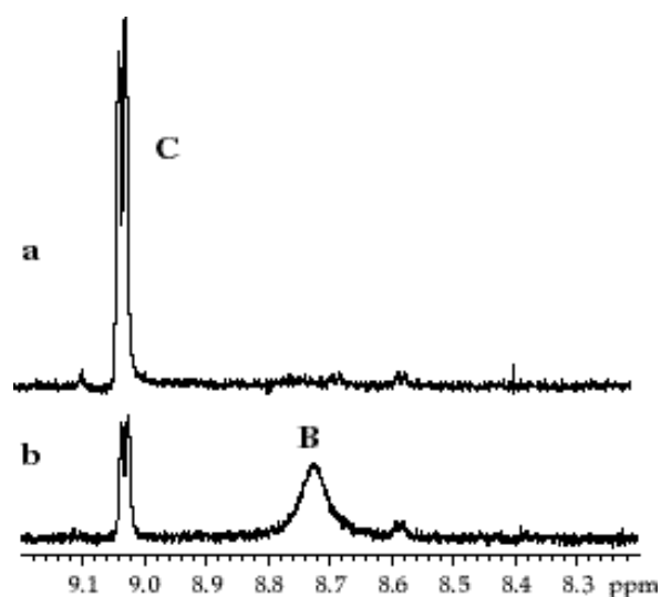
Figure 4.13. ^1\text{H} NMR spectra ( 0^\circ\text{C} , \text{C}_6\text{D}_5\text{Br} ) for the ortho pyridyl region after addition of 18 equiv \text{NMe}_2\text{Ph} and 1-hexene to 43 a) after 2 h; b) initially.
