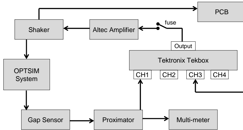
Figure 5-5: Tekbox Data Acquisition Setup
