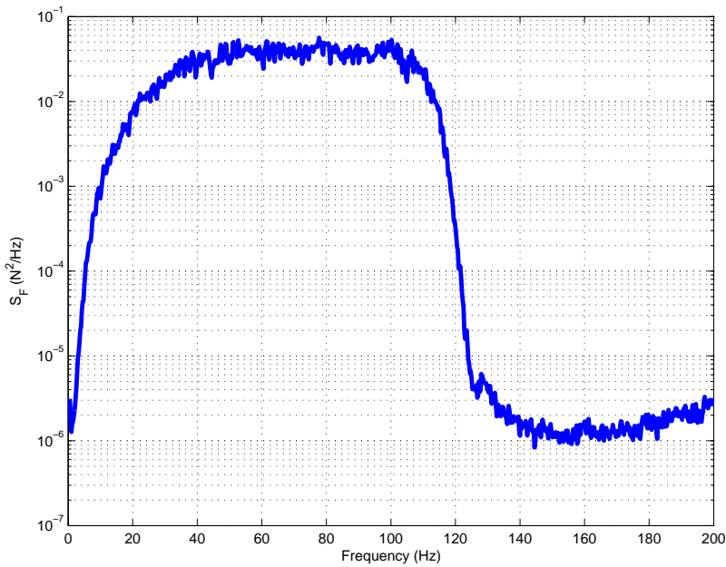
Figure 5-6: Input Noise Spectrum ( N^2/Hz )
