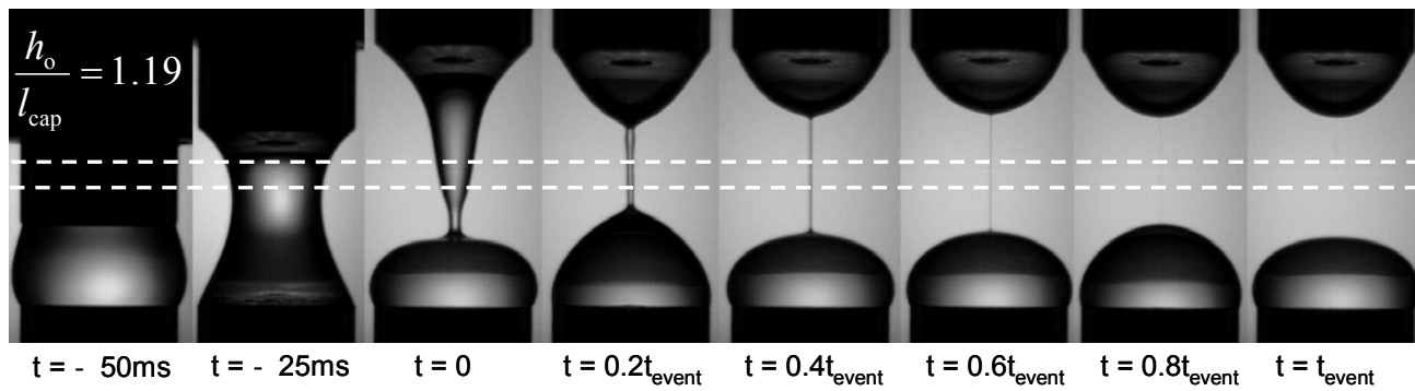
Figure 6. Filament thinning of the 0.3% PEO solution for an initial gap height of h_o = 3 mm and \Lambda = 1.61 , in which the total time of the event, t_{event} = 110 ms.
