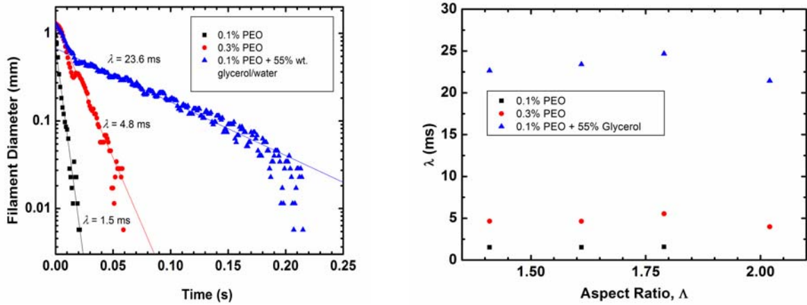
Figure 10. (a) Exponential decay of the fluid filament diameter for \Lambda=1.61 and h_0 = 3\text{mm} and (b) relaxation time as a function of aspect ratio, for the 0.1% PEO, 0.3% PEO and 0.1% PEO/glycerol solutions in which h_0 = 3\text{mm} .
