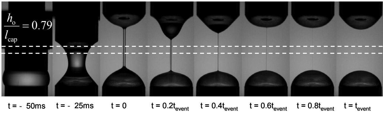
Figure 5. Filament thinning of the 0.3% PEO solution for an initial gap height of h_o = 2 mm and \Lambda = 1.61 , in which the total time of the event, t_{event} = 100 ms
