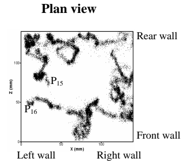
Fig. 8. Tracer trajectory in plan view over certain time period 1000-1320 s for cases C (surface waves).
