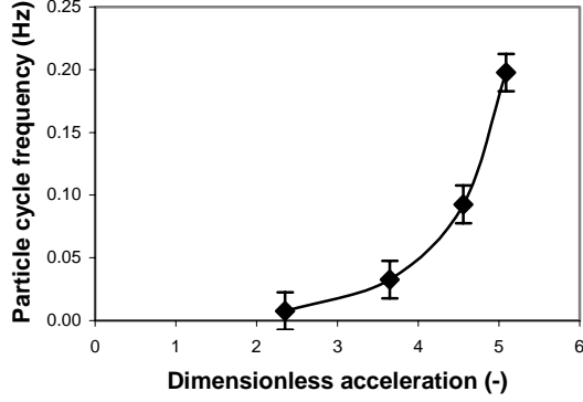
Fig. 9. Effect of vibration amplitude on the particle cycle frequency.
