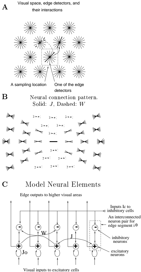
Figure 1: A : Visual inputs are sampled in a discrete grid by edge/bar detectors, referred to as edge or edge segments, modeling RFs in V1. Each grid point has K neuron pairs (see C ), one per edge segment. All cells at a grid point share the same RF center, but are tuned to different orientations spanning 180^\circ , thus modeling a hypercolumn. An edge segment in one hypercolumn can interact with another in a different hypercolumn via monosynaptic excitation J (the solid arrow from one thick bar to another), or disynaptic inhibition W (the dashed arrow to a thick dashed bar). See also C . B : A schematic of the neural connection pattern from the center (thick solid) edge to neighboring edges within a finite distance. J 's contacts are shown by thin solid edges. W 's are shown by thin dashed edges. All edges have the same connection pattern, suitably translated and rotated from this one. C : An input edge segment is associated with an interconnected pair of excitatory and inhibitory cells, each model cell models abstractly a local group of cells of the same type. The excitatory cell receives visual input and sends output g_x(x_{i\theta}) to higher centers. The inhibitory cell is an interneuron. Activity levels g_x(x_{i\theta}) often oscillate over time [27, 28], which is an intrinsic property of a population of recurrently connected excitatory and inhibitory cells. Temporal averages over multiple time constants after input onset are taken as the model output. The region dependence of the phases of the oscillations in this model could be exploited for segmentation[22], although it is beyond this paper. The visual space has toroidal (wrap-around) boundary conditions.
