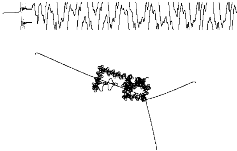
Figure 10. Three flies chasing each other. All the flies are controlled by the linear D_l(\psi) with nonlinear saturation of the total torque of each fly (see text). The velocity is constant. This apparently chaotic behavior is observed for small \Delta t (such as for instance \Delta t = .001 ). The inset above the figure shows the error angle of one of the fly relative to one of the other two as a function of time.
