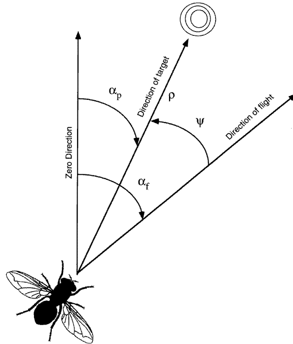
Figure 1. The angles used in our model and \rho , the distance of the fly to the target. \alpha_p is the direction of the target relative to the vertical; \alpha_f is the direction of flight relative to the vertical; \psi = \alpha_p - \alpha_f is the error angle.
