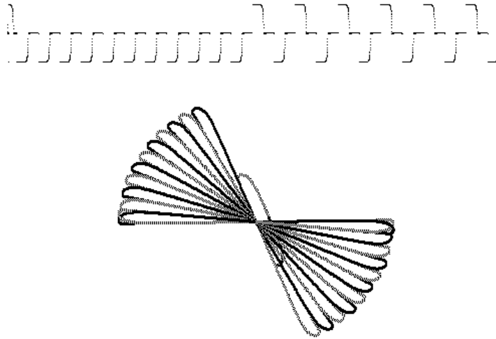
Figure 8. The behavior of two flies chasing each other. Both flies use now the nonlinear D_n(\psi) . The velocity is constant for both flies. In this simulation \Delta t = .001 but the same behavior is observed for a broad range of dt . As usual, the upper inset shows the error angle of one fly relative to the other plotted as a function of time.
