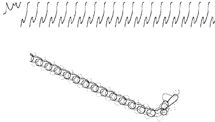
Figure 9. The behavior of three flies chasing each other. All the flies are controlled by the linear D_l(\psi) . The velocity is constant. This behavior is observed for a wide range of parameters (see later figures). The inset above the figure shows the error angle as a function of time.
