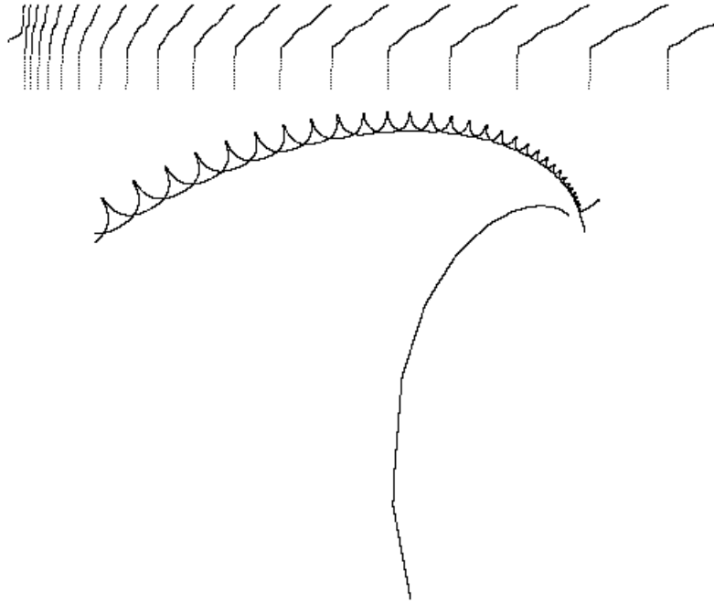
Figure 12. Three flies, two of which are chasing the others while one is escaping (its D_i(\psi) appears with a negative sign, see text). All the flies are controlled by the linear D_i(\psi) . The velocity is constant. This behavior is the most frequent and has been observed for a wide range of \Delta t 's (from 0.1 to 0.001). The inset above the figure shows the error angle of one of the chasing flies relative the other chasing fly as a function of time.
