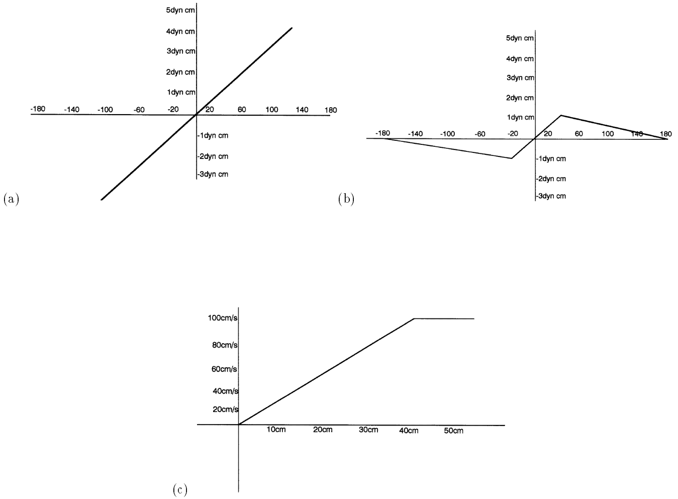
Figure 2a. The linear D_l(\psi) function describing how the torque generated by the fly depends on the error angle . This function seems to describe free-flight chasing by male flies Musca domestica (see Reichardt & Poggio, 1981). The ordinate is torque (dyn cm); the abscissa is degrees of visual angle. 2b) The nonlinear D_n(\psi) function describing how the torque generated by the fly depends on the error angle . This function seems to describe tracking in female flies Musca domestica (see Poggio & Reichardt, 1981). The ordinate is torque (dyn cm); the abscissa is degrees of visual angle. 2c) The function v(\rho) describing how the forward velocity is controlled depending on the distance to the target in chasing situations (see Poggio & Reichardt , 1981).
