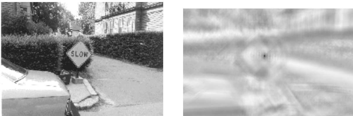
Figure 3: On the left, image Slow3. On the right, the ambiguity surface of image Slow3 computed for all possible translations given fixed angle and scaling parameters. A deterministic search would compute each value on this surface. A steepest descent procedure would fail because of local minima. Therefore, a stochastic search is used to find the best correlation value (here the darkest pixel value).
