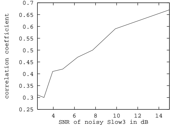
Figure 10: Correlation coefficient for sign recognition in noisy versions of image Slow3.
