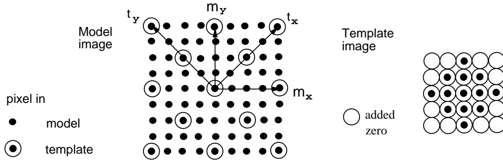
Figure 1: A 5 \times 5 template image is obtained from a 9 \times 9 model image using parameters s_x = s_y = 2 and \tau = 45 degrees.
