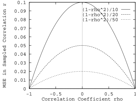
Figure 8: Mean squared error of r for p_T = 100, 400 and 2500 .
