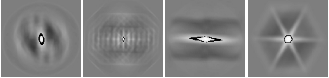
Figure 9: Auto-correlation of model images Footpath, Stop, E-no-entry, and Yield. To illustrate how fast the auto-correlation falls off, the e-folding lengths, i.e., pixels (x, y) with R(x, y) \approx 1/e , are shown on a dark contour.
