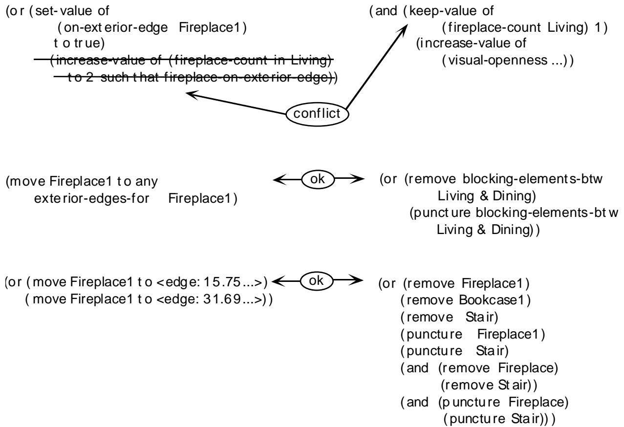
Figure 7.15: Lookahead results for fireplace-on-exterior-edge goal.
