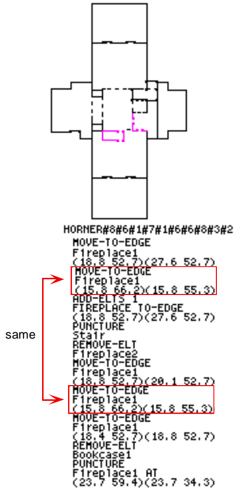
Figure 7.38: Nonminimal solution avoided by sequential with lookbehind. Identical suggestions are boxed; lookbehind pruned second suggestion.
