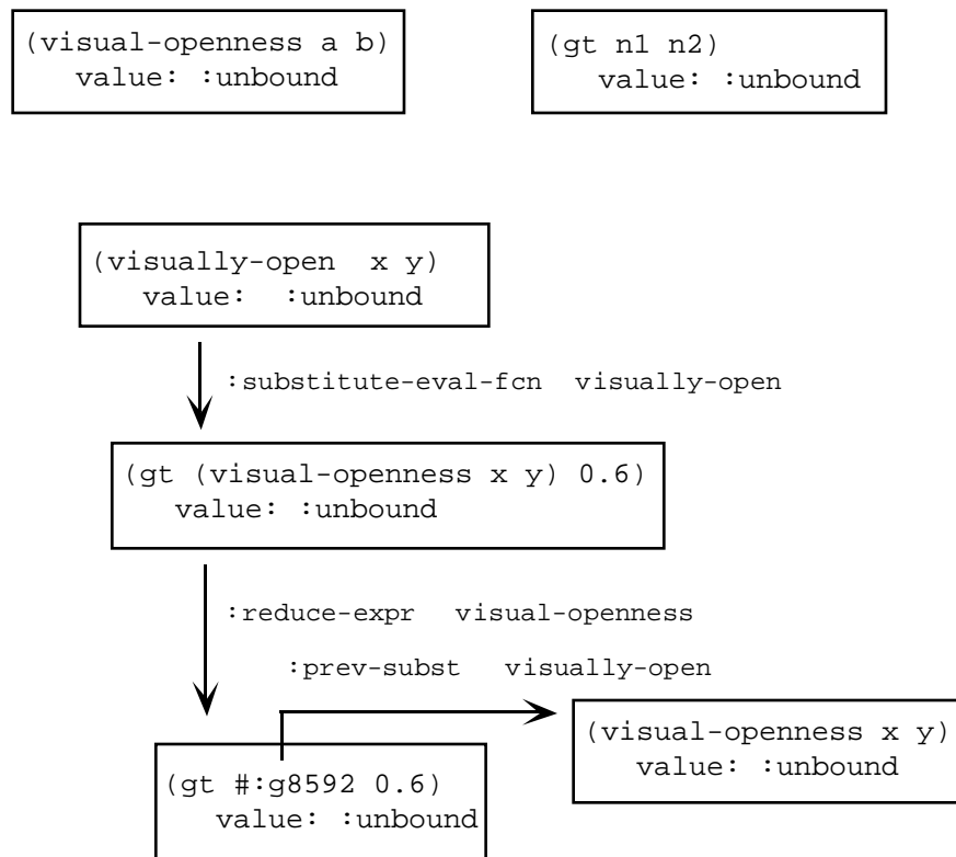
Figure E.1: Three explanation templates.
