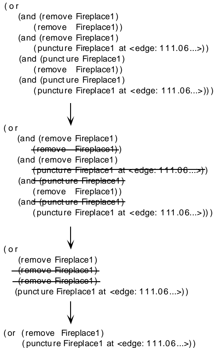
Figure 7.24: Pruning of suggestions for visually-open and visible-center goals.
