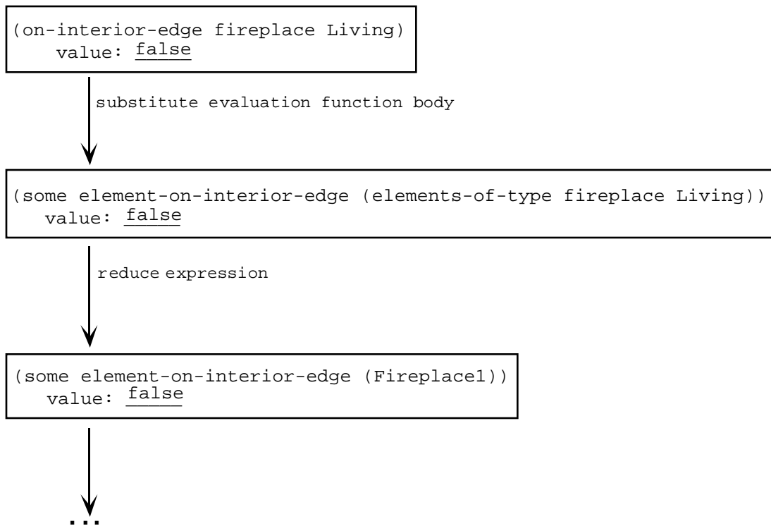
Figure 5.6: Part of explanation for (on-interior-edge fireplace Living) .
