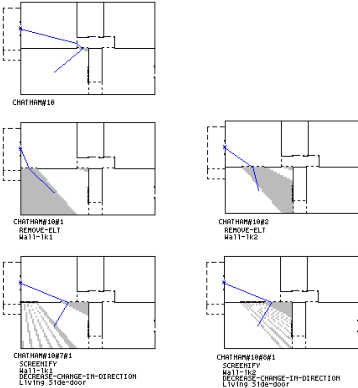
Figure 8.23: Starting design (top), solutions for Living visual openness and path from side door: 0.3 < \text{visual openness} < 0.8 , and 10 \text{ degrees} < \text{path direction change} < 120 \text{ degrees} . Shaded areas are visible; * is viewpoint; path is from side door to center of Living.
