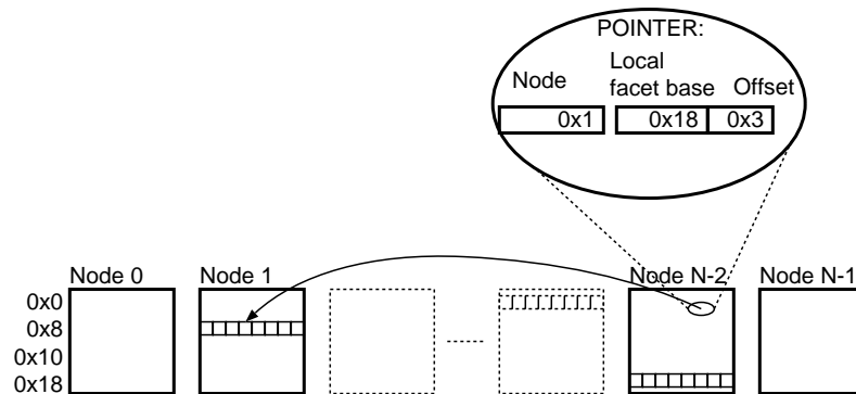
Figure 3.2: A sparsely faceted array with facets on a subset of nodes, and a pointer to element 3 on node 1. Note that within a node, pointers to the SFA on other nodes are represented in terms of the local facet address.
