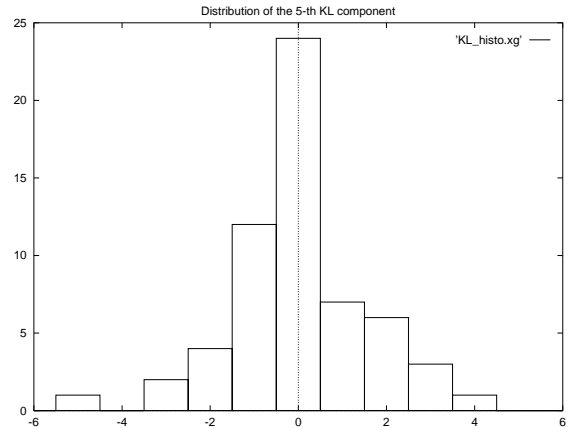
Figure 13: The distribution of the values of the 5-th principal component computed from 60 eyes images. Note the clear unimodality of the distribution which suggests the effectiveness of using a quadratic classifier in the feature subspace. The other components present a similar distribution.
