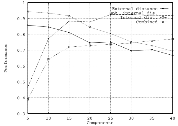
Figure 17: Performance of different strategies based on the computation of principal components. The horizontal axis reports the number of components used in the expansion, while the vertical axis reports the percentage of eyes correctly located (see text for a detailed explanation).
