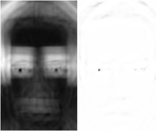
Figure 14: The map of the residual size (left) and of the projection probability (right). Note how the probability is low in regions where the reconstruction is good. The darker the value the lower the distance and the higher the probability.
