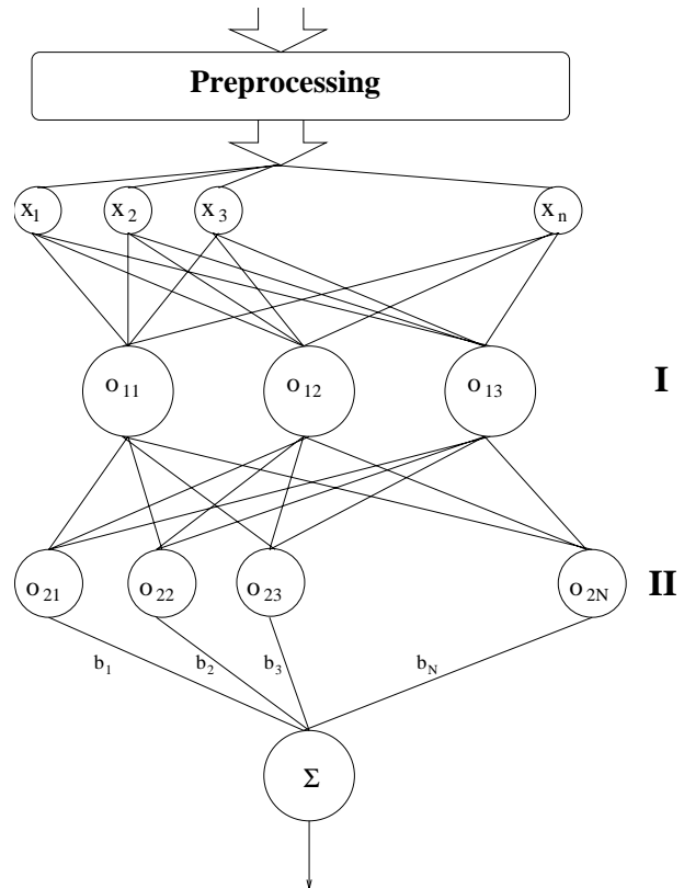
Figure 19: An approximation network for template matching. The preprocessing stage applies simple transformation to the input pattern (e.g. to emphasize high frequency components).
