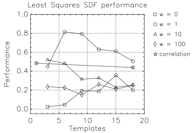
Figure 18: Performance of least squares SDF with different amount of regularizing noise. Correlation performance is also reported using the average template and the whole set of available templates. The horizontal axis reports the number of patterns used in building the filters, while the vertical axis reports the percentage of eyes correctly located (see text for a detailed explanation).
