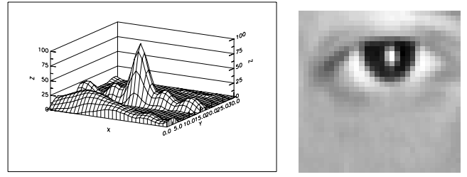
Figure 8: Non linear processing can be employed. The figure represent the result of preprocessing the image to extract the local image contrast (intensity value over the average value in a small neighborhood). This kind of preprocessing emphasizes high frequencies and results in a sharp correlation peak.
