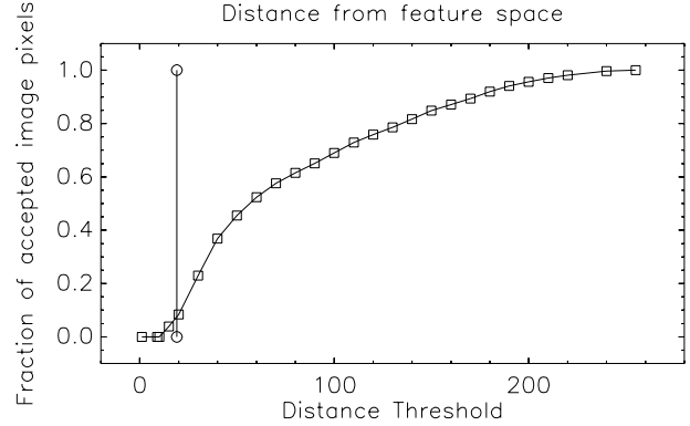
Figure 12: The fraction of image pixels classified as right eye as a function of the threshold on the residual. The first 10 eigenvectors from a population of 60 images were used. The image used for the plot was of a person not in the database. The vertical line represent the threshold computed by summing the residual eigenvalues. The correct eye is the only selected region for d < 11 , the other eye being selected next.
