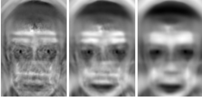
Figure 6: The output of the correlation with an SDF computed using the spectral envelope of 10 training images and different amounts of white noise (left: \alpha = 1 , middle \alpha = 5 ) compared to the output of normalized cross-correlation using one of the images used to build the SDF but without any spectral enhancement. The darker the image the higher the corresponding value. Note that an increased amount of white noise improves the response of the filter.
