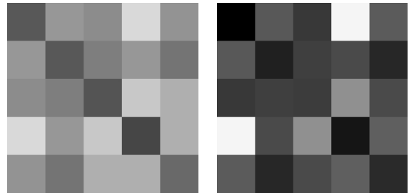
Figure 10: The square of coordinates ij represents the average value of distances of views of the i -th and j -th clip (darker values represent smaller distances). LEFT: euclidean distances of views of the different clips; RIGHT: distances computed using the learned metric W_0^T W_0
