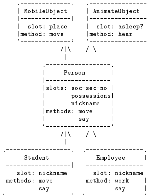
Figure 1: An example delegation-based instance.
