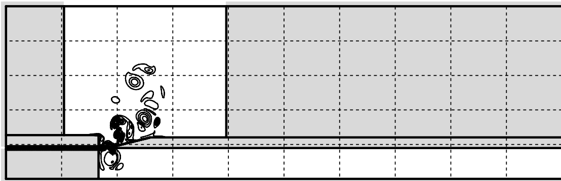
Figure 8: Simulation of a 20 cm closed-end soprano recorder. Picture is 30 ms after startup. Iso-vorticity contours are plotted. The dashed lines show the decomposition of the problem into 22 workstations. The gray-shaded areas are not simulated.
