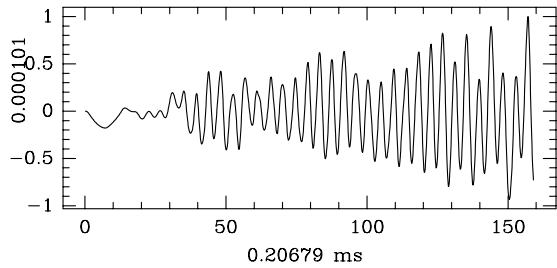
Figure 5: Simulation, 1108 cm/s
