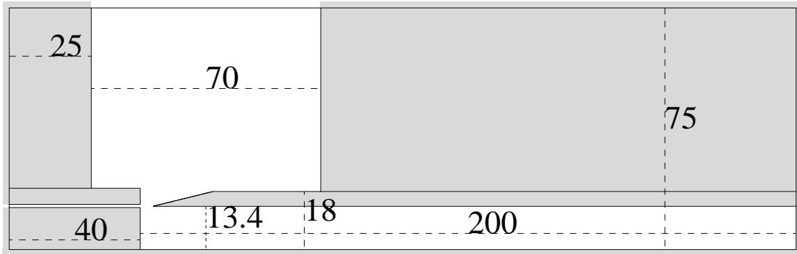
Figure 7: The two-dimensional geometry of the soprano recorder which is used in the simulations. The numbers shown correspond to millimeters. The pipe is located at the bottom of the picture, and measures 20 cm long and 1.34 cm wide. The flue channel is located at the bottom left corner, and measures 4 cm long and 0.1 cm wide. At a distance of 0.4 cm in front of the flue channel, there is a sharp labium which measures an angle of 14 degrees approximately, and is positioned slightly below the midline of the flue channel. Namely, the tip of the labium is located at 1.34 cm from the bottom of the pipe, and the flue channel is located between 1.3 cm and 1.4 cm.
