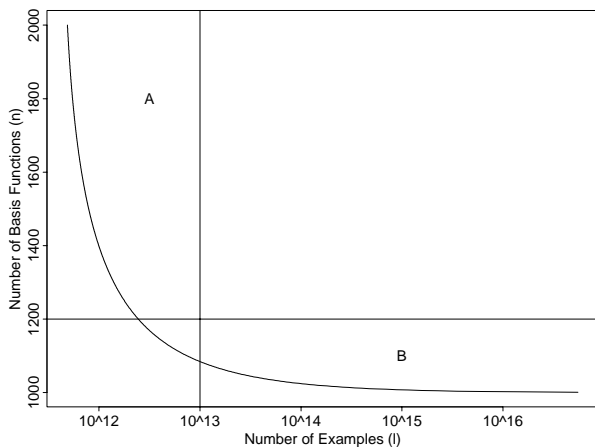
Figure 4: This figures shows various choices of (l, n) which give the same generalization error. The x -axis has been plotted on a log scale. The interesting observation is that there are an infinite number of choices for number of basis functions and number of data points all of which would guarantee the same generalization error (in terms of its worst case bound).
