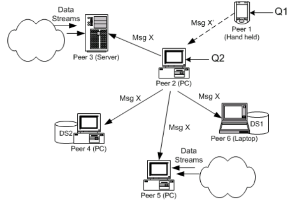
Fig. 5. Overview of CQ-Buddy Network.
