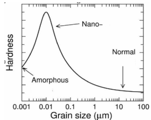
Fig. 1. Hardness evolution with change of grain size
