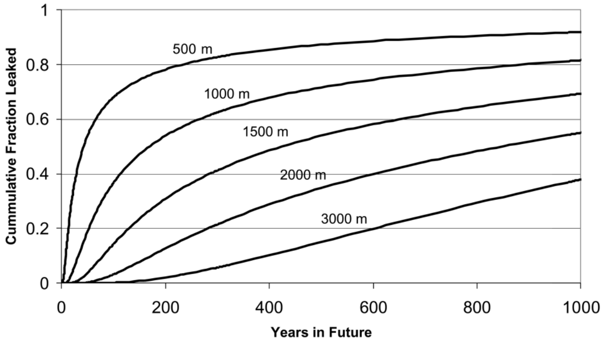
Figure 1. Leakage over time as a function of injection depth.
