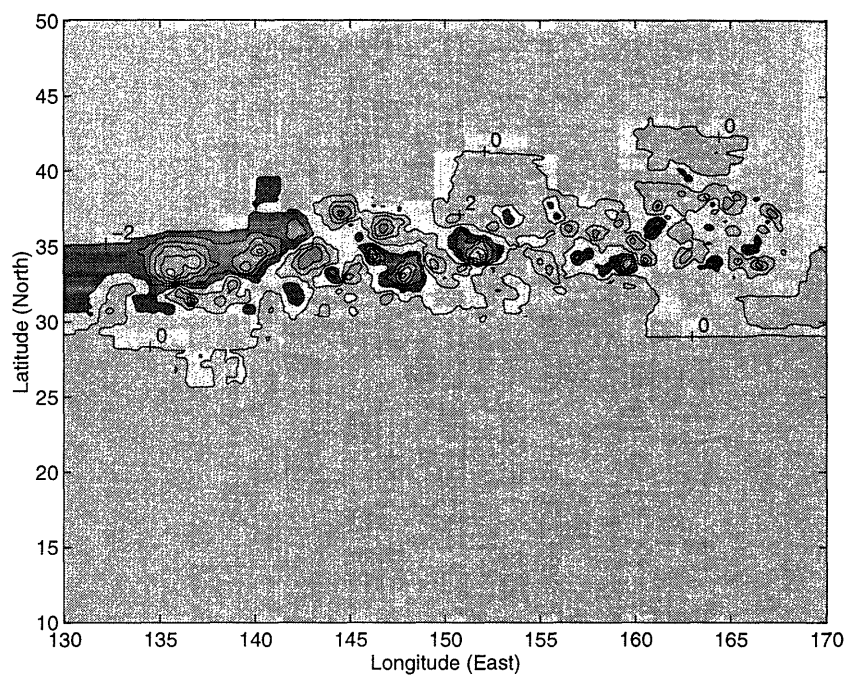
Figure 12: Differences (in cm) in the estimates produced by a homogeneous multiscale model and a model accounting for the presence of the Kuroshio.
