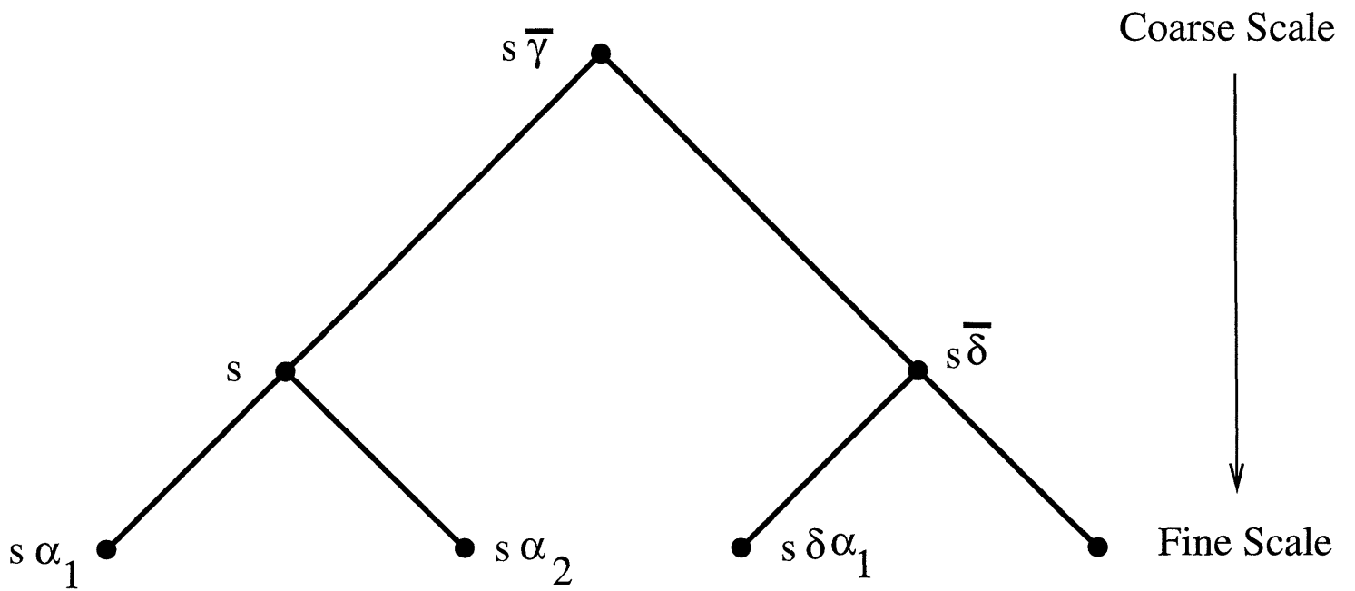
Figure 15: Simple multiscale tree demonstrating node nomenclature
