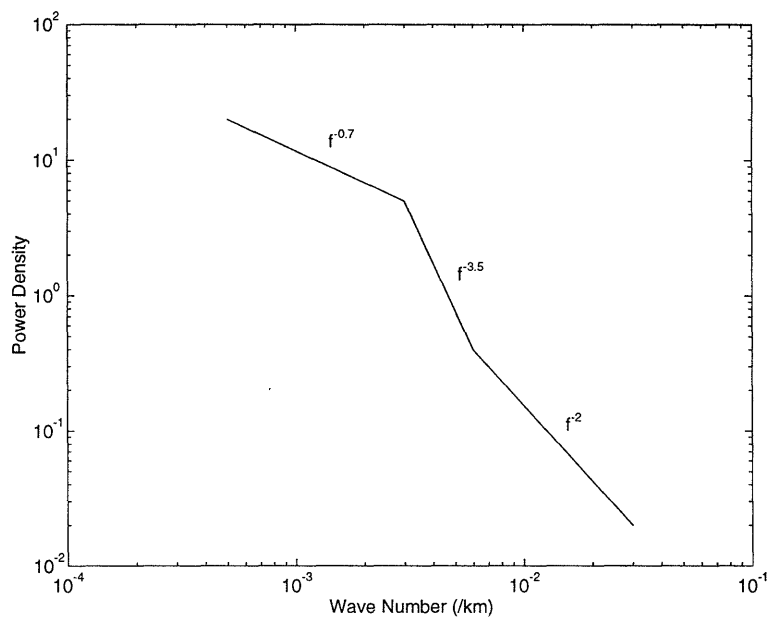
Figure 4: Rough characterization of global power spectrum (from [8])
