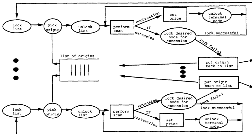
Figure 4: Flow diagram of the parallel forward-only auction shortest paths algorithm for the all origin - one destination problem.
