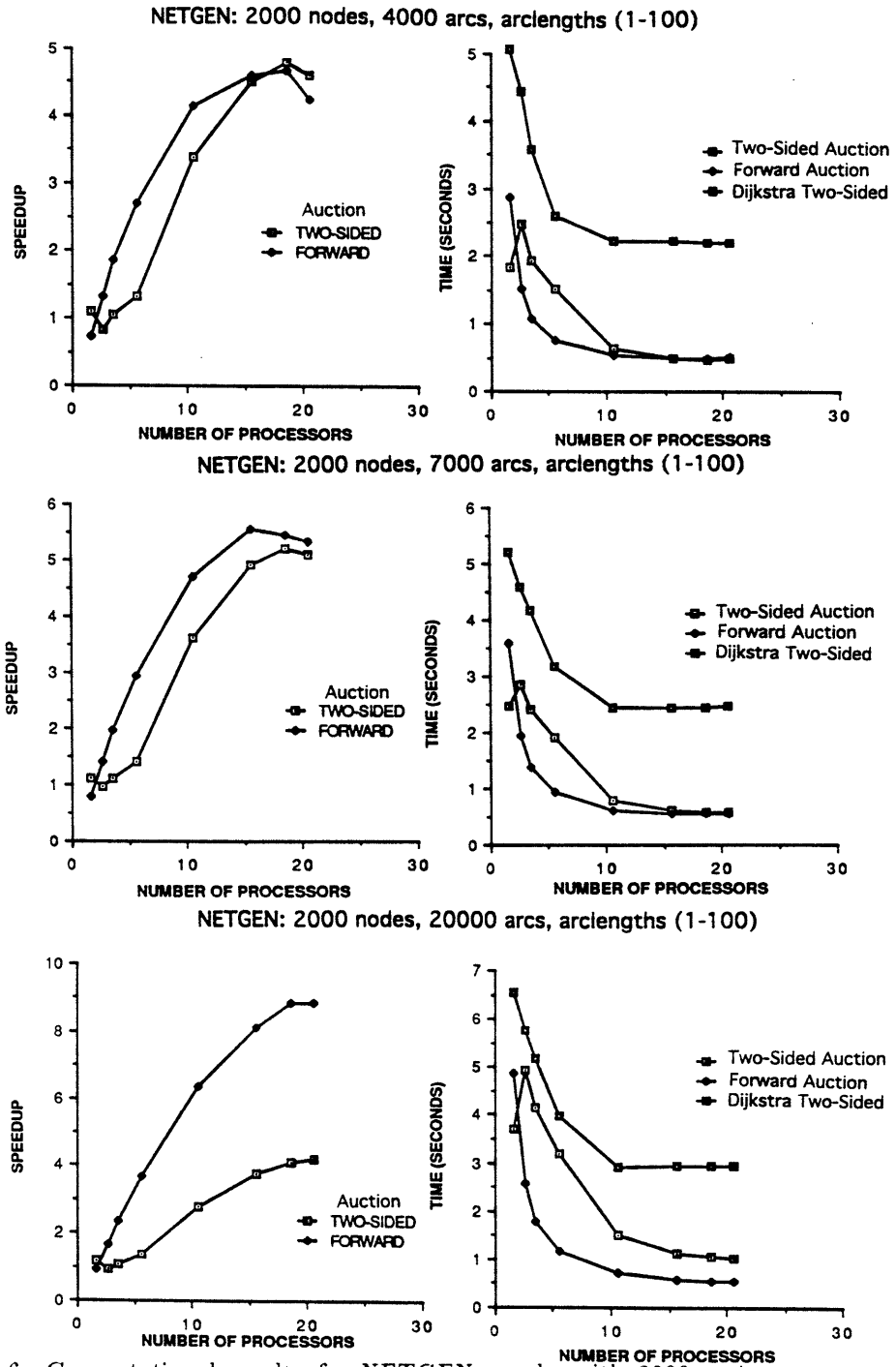
Figure 6: Computational results for NETGEN graphs with 2000 nodes and 4000, 7000 and 20000 arcs respectively. The arc lengths range from 1 to 100. We see that as the density of the graph increases the factor of superiority of the forward-only auction over the two-sided algorithm increases. The auction schemes are much faster than the parallel two-sided Dijkstra algorithm.
