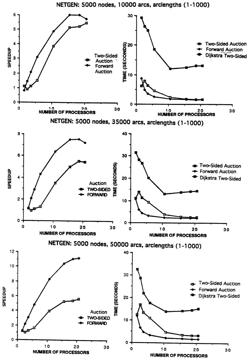
Figure 5: Computational results for NETGEN graphs with 5000 nodes and 10000, 35000 and 50000 arcs respectively. The arc lengths range from 1 to 1000. We see that as the density of the graph increases the factor of superiority of the forward-only auction over the two-sided algorithm increases. The auction schemes are much faster than the parallel two-sided Dijkstra algorithm.
