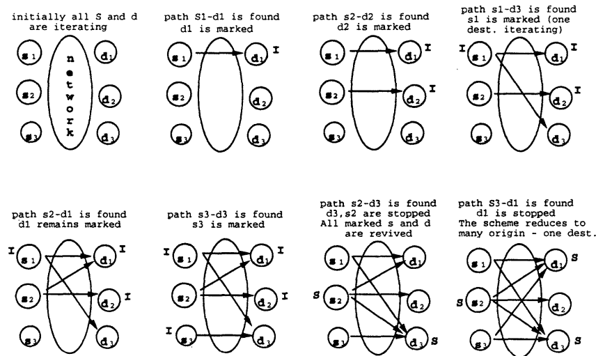
Figure 3: A demonstration of the many origin - many destination serial auction. A node with I on its side is marked idle. A node with S on its side has become inactive.
