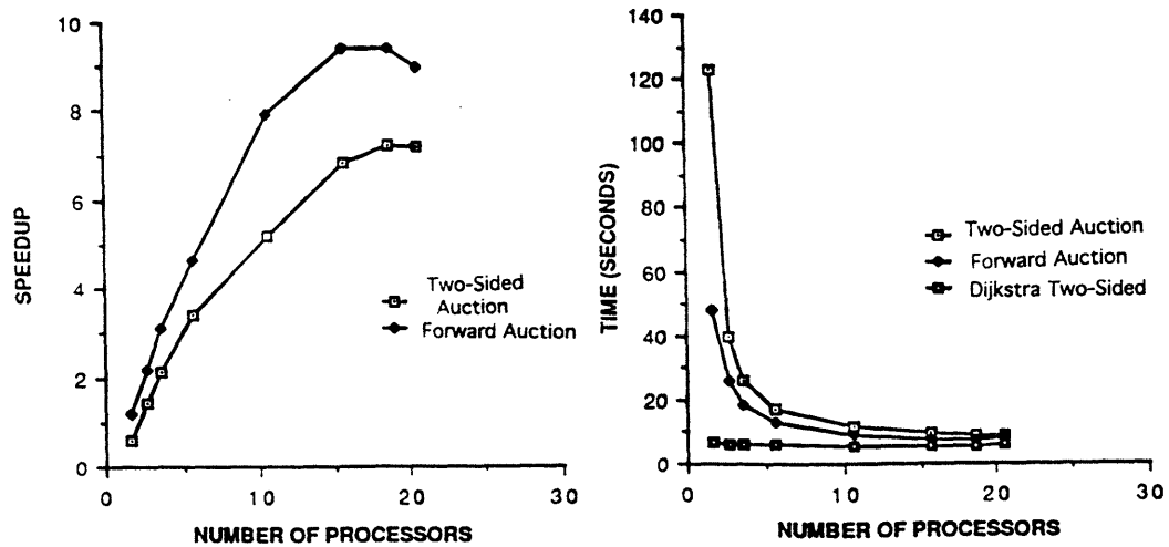
SQUARE GRID: 4900 nodes, 14421 arcs, arclengths (1-100)
