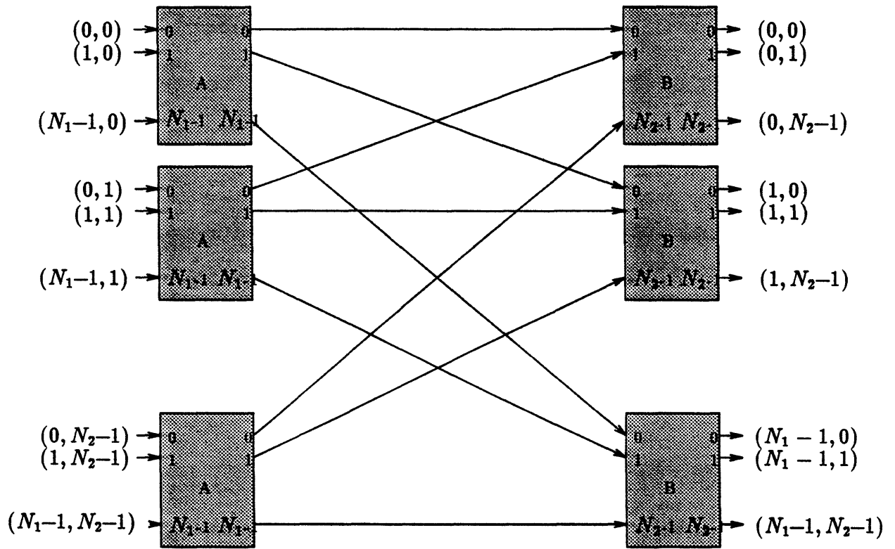
Figure 8: 2 Stage Design
