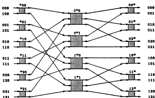
Figure 10: 3-stage design, N_1 = 2, N_2 = 3, N_3 = 2
