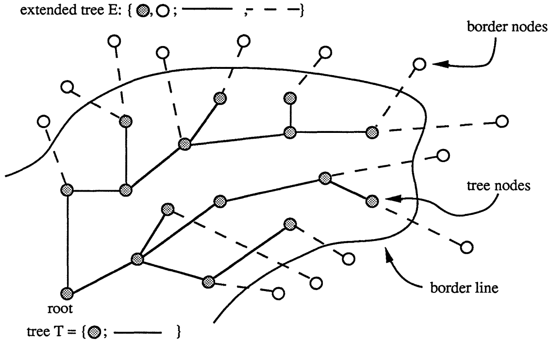
Figure 4: Illustration of the structure of the extended tree E .
