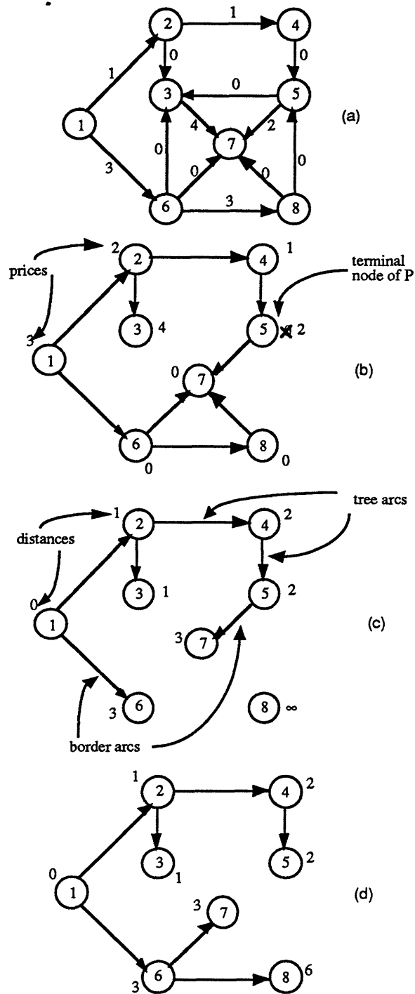
Figure 3: Illustration of the algorithm for an example problem.
