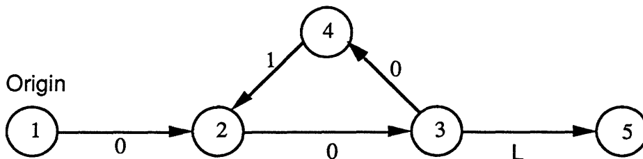
Figure 1: Illustration of pseudopolynomial behavior of the auction algorithm. Here the origin is node 1 and the destination is node 5. The arc lengths are shown next to the arcs. L is a large integer. Beginning with p_i = 0 , for all i , the price p_i is increased L times, by 1 unit, for i = 1, 2, 3, 4 . In fact, only when p_3 reaches L , an extension to the destination 5 is possible.
