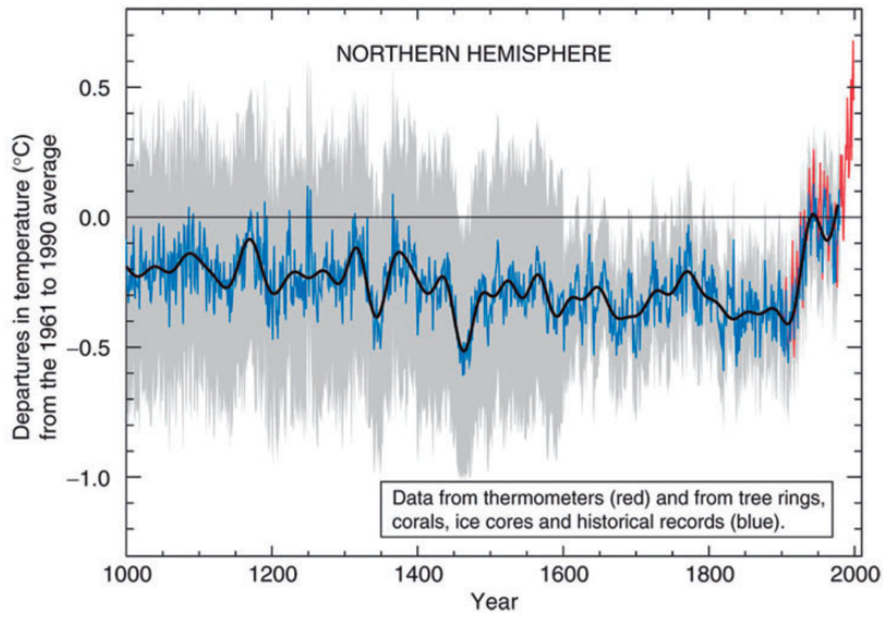
Figure 5. The ‘Hockey Stick’ graph (named because of its shape), from the 2001 Intergovernmental Panel on Climate Change (IPCC). This graph mobilized world-wide debate on the topic of global warming. Image courtesy of IPCC, available at: www.grida.no .
