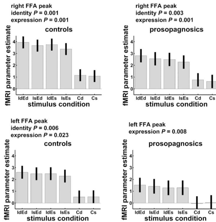
Figure 7. Identity and expression repetition suppression in individually defined FFA. Average peak parameter estimate (beta weight) with 95% confidence intervals in right and left for the six conditions. Also shown are p values near to or less than .05 for identity repetition suppression (denoted “identity”) and expression repetition suppression (denoted “expression”).
