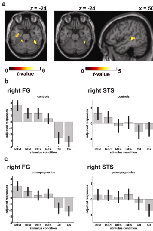
Figure 6. Identity and expression repetition suppression: SPM random effects analysis. (A) Regions in non-DP control participants showing significant identity repetition suppression in the right FG (left) and expression repetition suppression in right FG (middle) and right mid-STS (right). The right side of each transverse image represents the right hemisphere. (B) Pattern of mean “adjusted responses” (condition-wise beta weights, adjusted for other regressors in general linear model) in non-DP control participants from the peak right FG and right mid-STS voxels found in both identity and expression repetition suppression contrasts. (C) For comparison, we show the pattern of adjusted responses in DPs using the peak right FG and mid-STS voxels shown in (B). All participants were included in SPM analyses.
