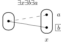
Figure 5: A value elimination pattern corresponding to neighbourhood substitution.
