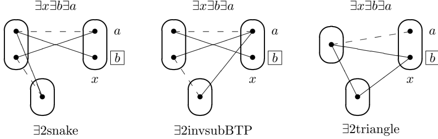
Figure 6: Three val-elim patterns.
