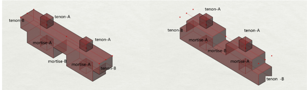
Figure 6 Tenon and mortise elements for Unit1 ( left ) and Unit2 ( right )
