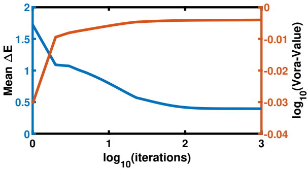
Figure 3: Algorithm convergence in terms of Vora-Value (to the right y-axis) and mean \Delta E^* with respect to iterations (to the left y-axis). Note that we plot the x-axis under \log_{10} .
