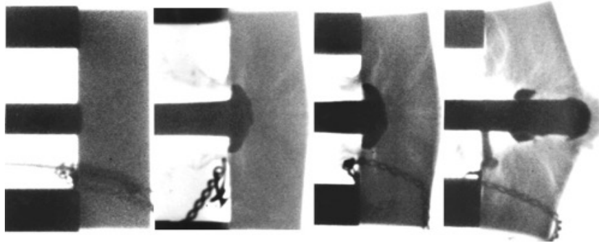
Figure 16. An X-ray sequence showing a steel rod 10 mm in diameter hitting a block of soda-lime glass at a velocity of about 540 \text{ m s}^{-1} [130].
