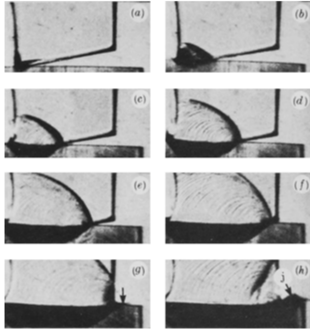
Figure 9. Liquid impact (at 150 \text{ m s}^{-1} ) using the two-dimensional gelatine technique. From [99].
