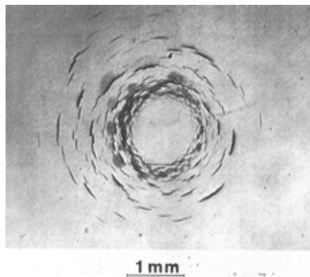
Figure 11. Liquid drop impact damage site on zinc sulphide. From [107].
