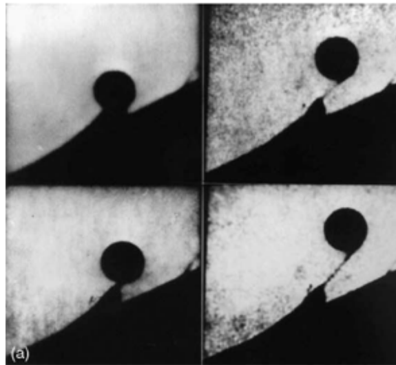
Figure 5. Selected frames from a high-speed photographic sequence showing the pulling out of a filament of polyethylene caused by the impact of a 4mm diameter steel ball at 190 m s -1 at 25° impact angle. Interframe time 19 μs. From [14].
