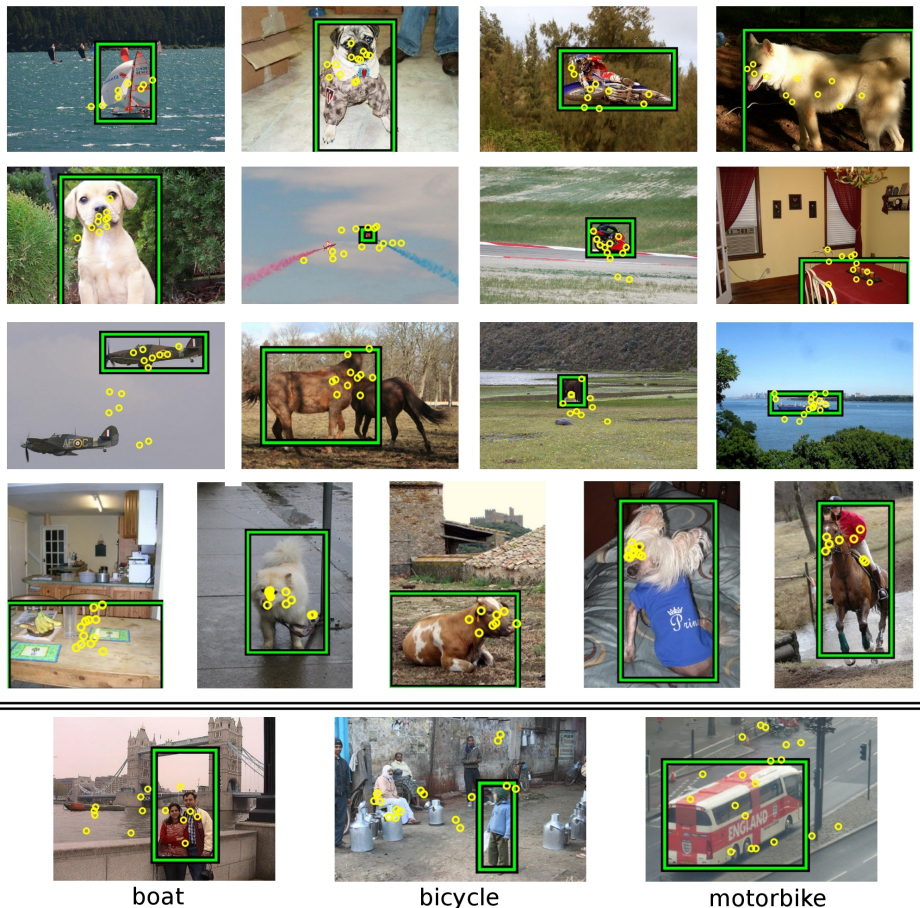
Fig. 7. Qualitative results of our method for localizing objects given fixations. The fixations are indicated with yellow circles while the predicted bounding-boxes are in green. Successful examples are shown in the first four rows for various classes, while some failure cases are shown in the last row. Note how our method nicely outputs a bounding-box covering the whole object even when the fixations are concentrated on only part of it, often the center, or the head.
