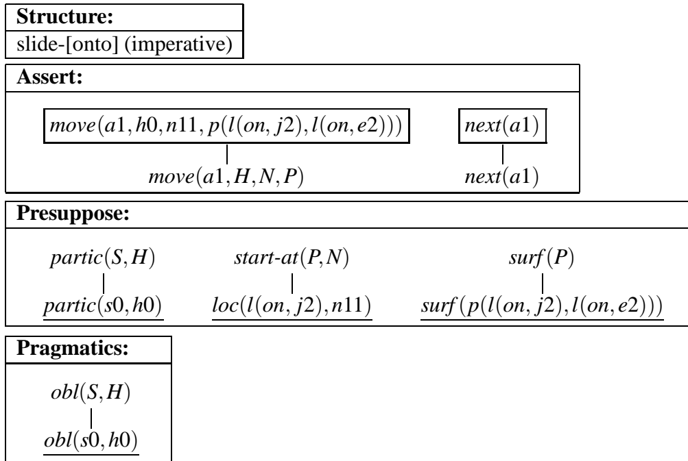
Figure 4: Interpretation of slide in (2). The speaker’s presumptions map out intended connections to discourse referents as follows: the speaker S , s0 ; the hearer H , h0 ; the nut N , n11 ; the path P , p(l(on, j2), l(on, e2)) ; the elbow E , e2 . The fuel-line joint is j2 .
