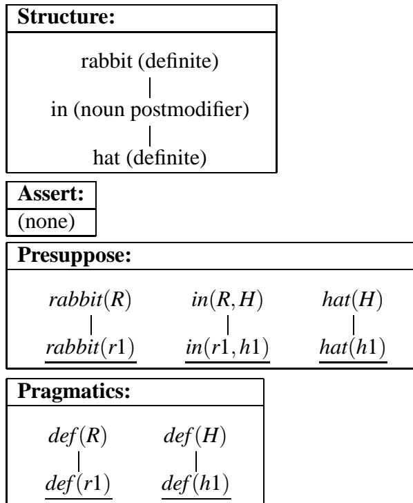
Figure 13: Communicative intent for the rabbit in the hat .
