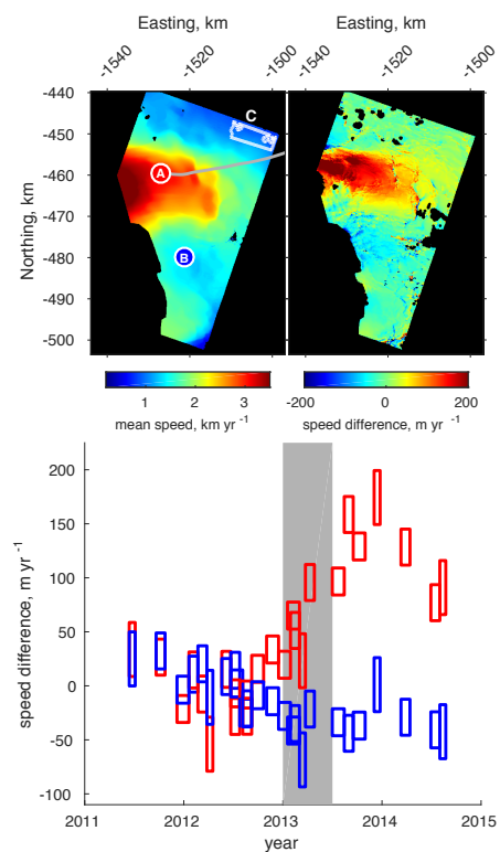
5 Figure 6. Detail showing speed change at the grounding line, based on Terrasar-X and TanDEM-X SAR velocities. Upper left: the mean speed between mid 2011 and late 2012. Upper right: Speed difference between the August 27, 2013 speed map, and the 2011-12 mean speed. The grey line indicates the position of the velocity profile in figure 5. Bottom: Speed change relative to the 2011-12 mean, for two regions, marked 'A' and 'B'. Data from region C were used to correct speed offsets as a function of time. The grey bar indicates the time range of the lake drainage.
