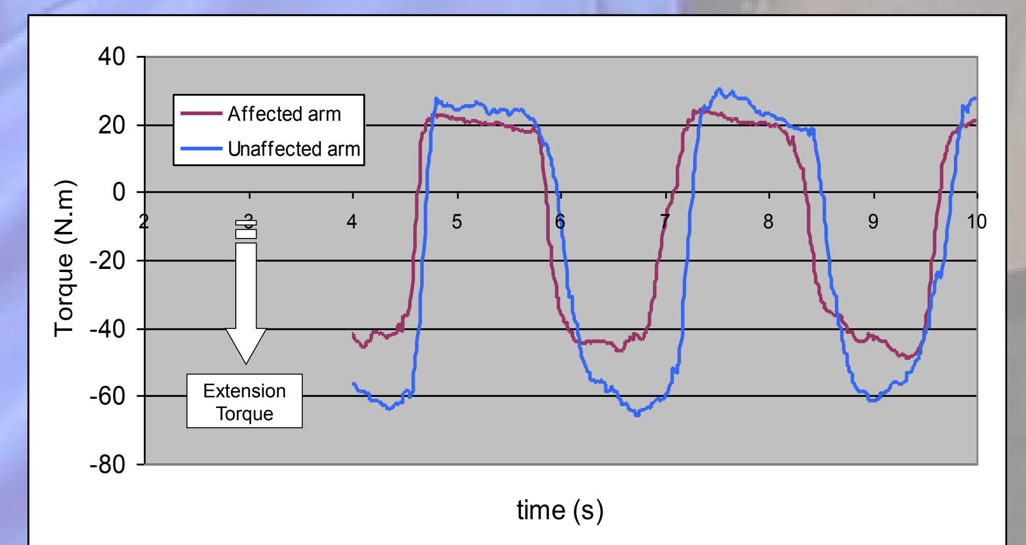
Figure 2. Typical extension torque curve.
