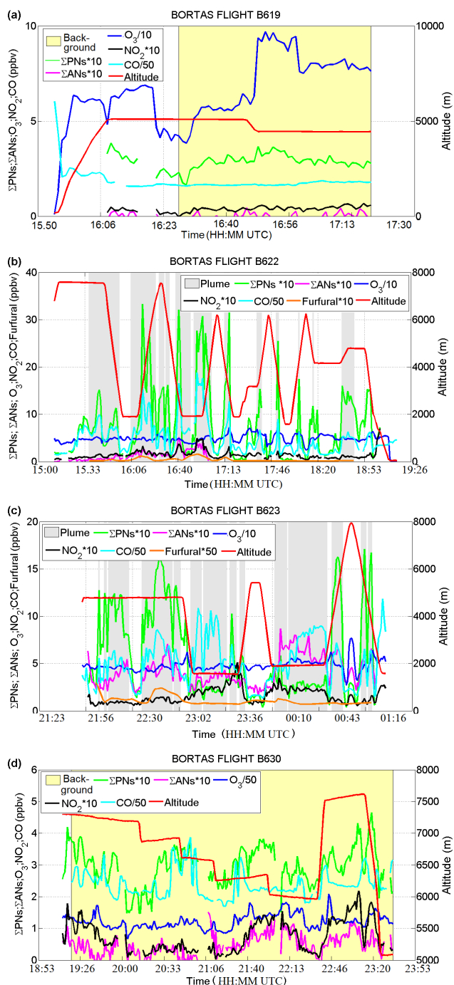
Figure 5. Time series of the \Sigma\text{PNs} , \Sigma\text{ANs} , \text{NO}_2 , \text{O}_3 , \text{CO} , furfural (ppbv) measured during the flights in this analysis: the flights B619 (a) and B630 (d) were background plumes, flight B622 was in part impacted by fire plume and in part by no fire (b), and flight B623 (c) was affected by fire plume. Time is reported in Coordinated Universal Time (UTC).
