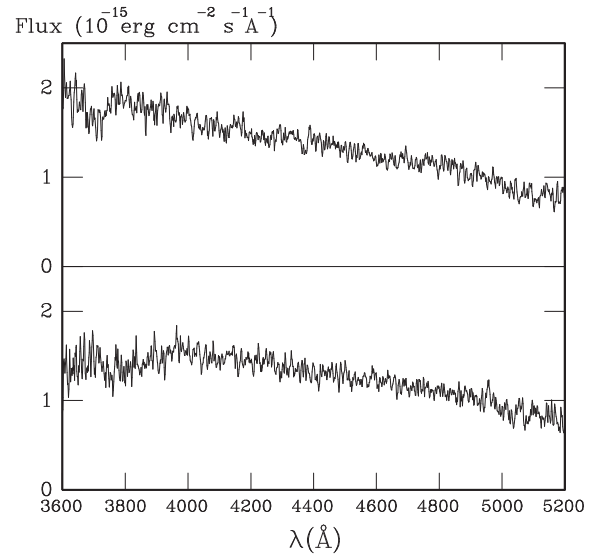
Figure 10. Spectrograms for EC 01302-2759 on the nights 1987 Dec 20/21 and 1989 Dec 21/22. These have been smoothed with a five-point running mean in the ratios 1:2:4:2:1.
