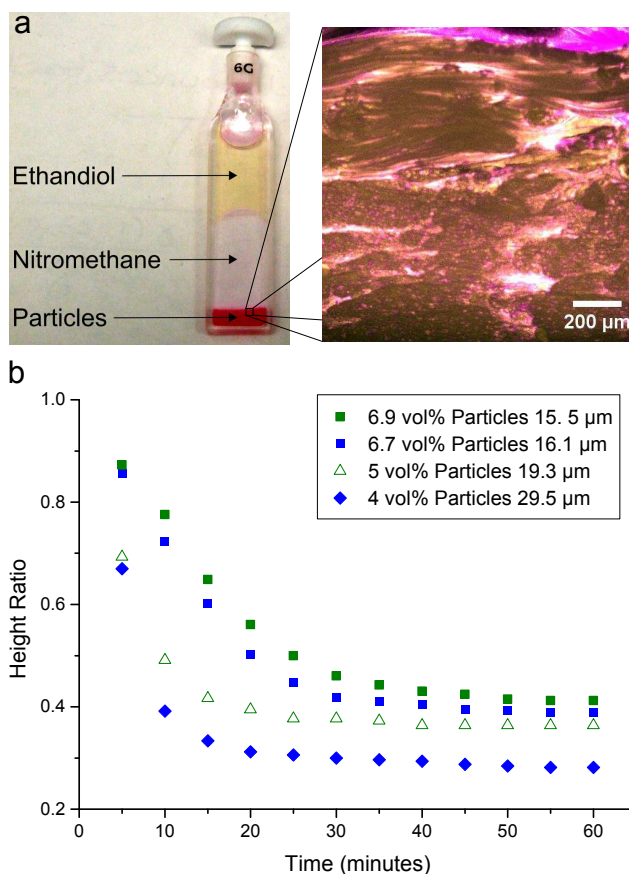
Fig. 2 a: An image showing the appearance of a bijel with 3 vol% particles and an interface separation of 60 \mu\text{m} that has been completely destroyed by centrifugal compression at 360 g for 30 minutes. A confocal image of the structure of the particle fraction is also shown where the particles are coloured yellow and the ethanediol coloured magenta. b: A height ratio ( H_c/H ) versus time graph for samples made with 7 vol% (filled squares), 5 vol% (open triangles) and 4 vol% (filled diamonds) of particles with different domain sizes centrifuged at 14 g.
