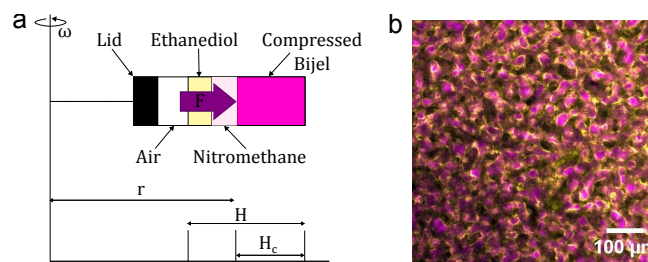
Fig. 1 a: Schematic of the experimental set-up for centrifuging bijels. b: A confocal microscopy image of the initial structure of a typical bijel with 5 vol% particles and an interface separation of 27 \mu\text{m} . The ethanediol phase is coloured magenta and the particles are coloured yellow.
