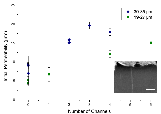
Fig. 8 A graph showing the relationship between the initial permeability and number of channels caused by bubbles in the sample where blue diamonds are the bijels with a domain size of 30 - 35 \mu\text{m} and green squares are the bijels with a domain size of 19 - 27 \mu\text{m} . Inset: An image showing a channel in a sample after centrifugation. The scale bar is 2 mm.
