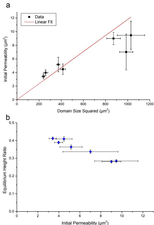
Fig. 3 a: A graph showing the relationship between the initial permeability and the square of the domain size of samples centrifuged at 14 g. b: A graph showing the relationship between the initial permeability and the final height ratio achieved after 1 hour of centrifuging at 14 g.
