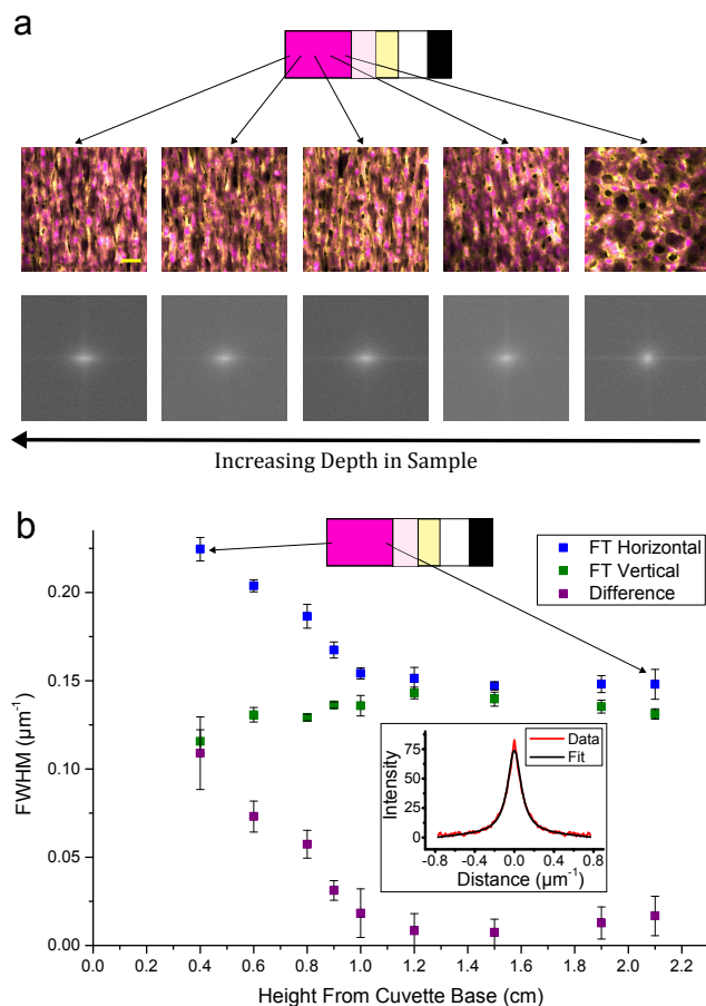
Fig. 5 a: Images of a compressed bijel with 5 vol% particles and an interface separation of 32\ \mu\text{m} which was centrifuged at 15\ \text{g} for 5 minutes with increasing depth in the sample where the ethanediol rich phase is coloured magenta and the particles are coloured yellow. The scale bar is 50\ \mu\text{m} . The bottom line is the fast Fourier transform (FFT) of these images. b: A graph showing the full width half maximum (FWHM) of the FFT peak obtained using a heuristic fit function versus the height from the cuvette base. The schematic shows the orientation within the sample. Inset: A graph showing a peak from the fast Fourier transform (red) and the respective fit functions (black).
