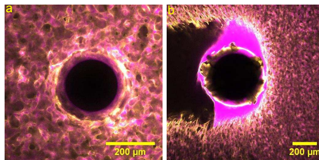
Fig. 7 a: An image taken on the confocal microscope of an air bubble in a bijel with 5 vol% particles and an interface separation of 40 \mu\text{m} . b: An image taken on the confocal microscope of bubble and track after centrifuging for 5 minutes at 15 g in a bijel with 5 vol% and an interface separation of 23 \mu\text{m} . The ethanediol rich phase is coloured magenta and the particles are coloured yellow.
