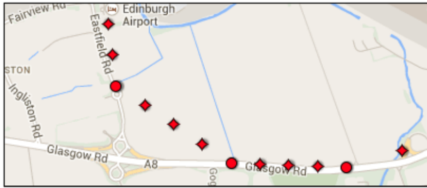
Fig. 7. Some simple interpolation is computed, but naively. The placement of these interpolation points suggests that the bus made the transition from Eastfield Road to Glasgow Road by driving across a field instead of navigating the roundabouts and joining via the slip road, as it of course did.
