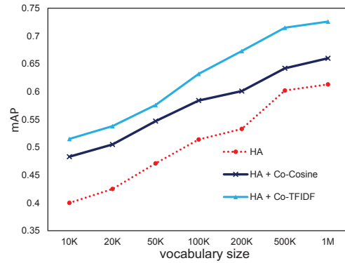
Fig. 6. Comparisons of HA and HA + Co-Sim (Co-Cosine and Co-TFIDF) with different sizes of hard-assigned vocabularies.
