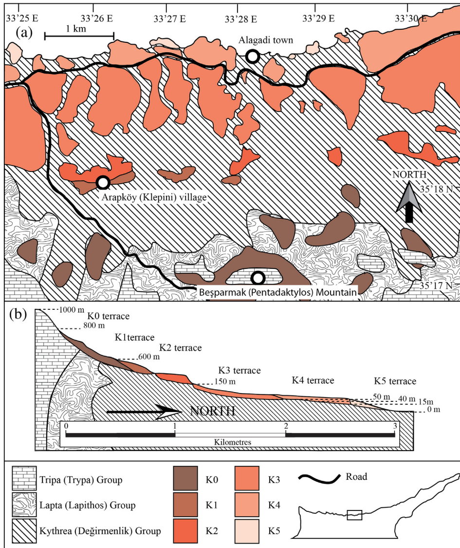
Fig. 2. (a) Geological map of part of the northern flank of the central Kyrenia Range showing the distribution of the K0 to K5 terraces (Ducloz, 1964) and (b) a simplified cross-section of the northern flank of the range showing the terrace relationships and heights.
