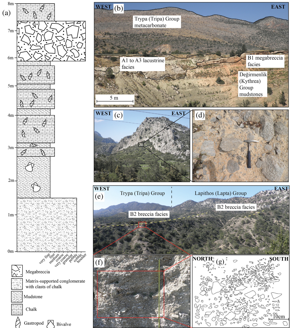
Fig. 3. Photographs and sketches of deposits of the K0 terrace system: (a) Summary log of the lacustrine facies (A1–A3 facies) preserved in the central Kyrenia Range; (b) labelled photograph of the interbedded relationship of the lacustrine facies and B1 facies megabreccia; (c) photograph of the K0 terrace megabreccia at the base of a metacarbonate-rock cliff; (d) photograph of the B1 facies megabreccia of the K0 terrace; (e) photograph of the B2 breccia deposit surface dipping away from the E–W axis of the Kyrenia Range; (f) photograph of the B2 facies breccia; (g) sketch of the B2 facies breccia.
