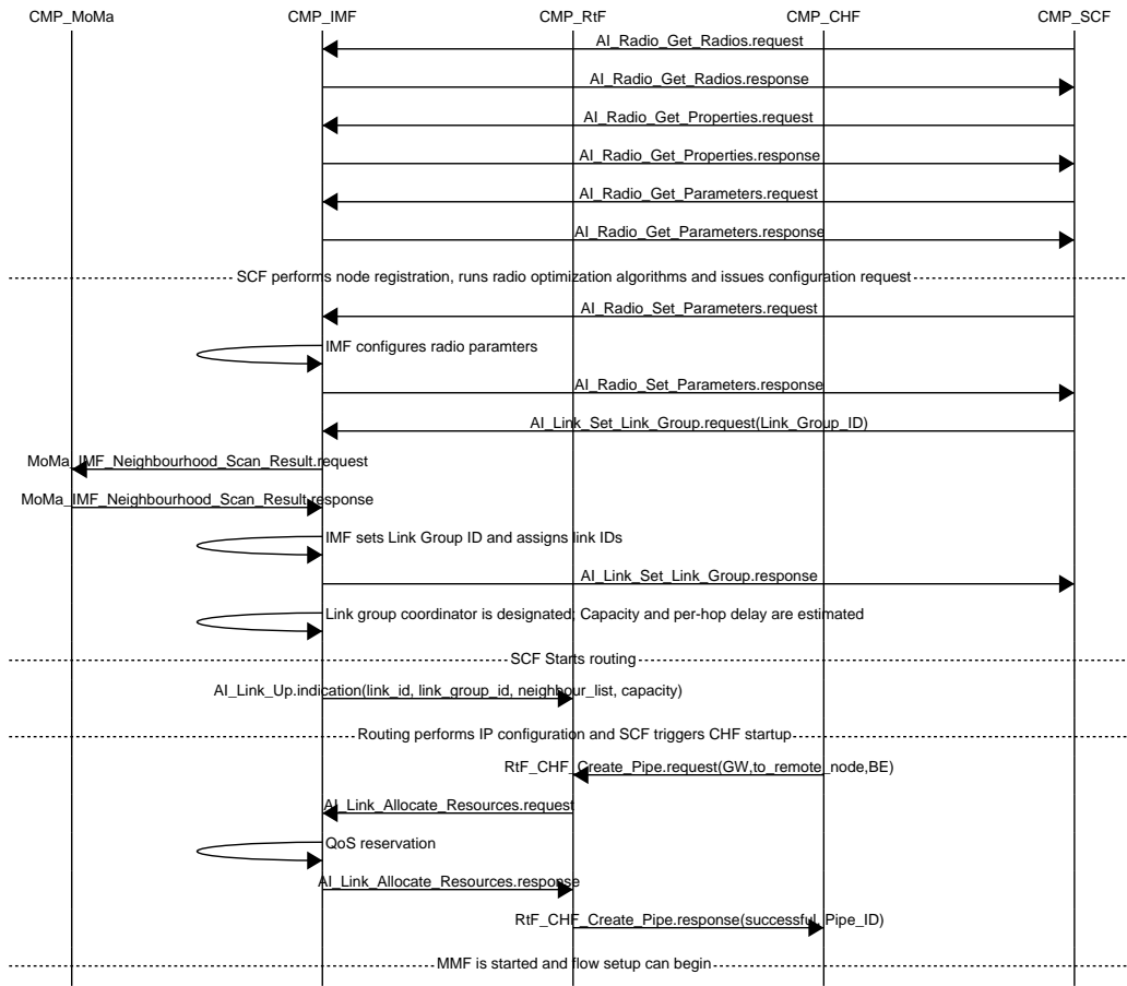
Figure 4: Message sequence chart for the bootstrap phase
