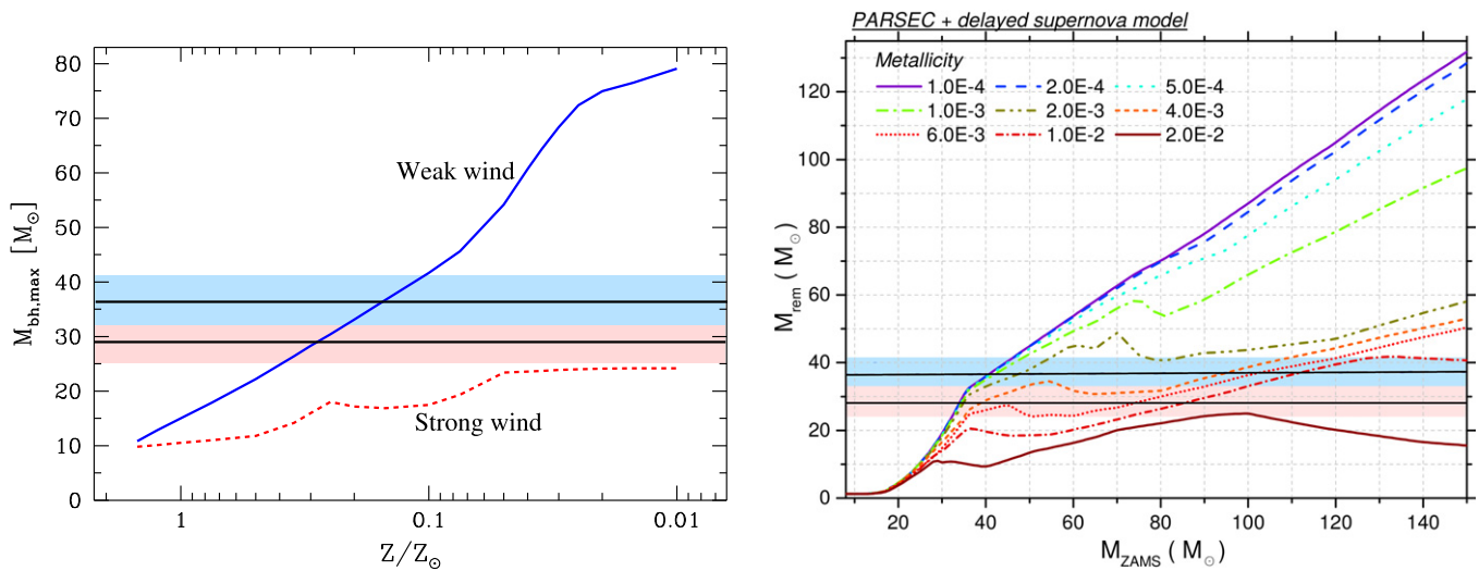
Figure 1. Left: dependence of maximum BH mass on metallicity Z , with Z_\odot = 0.02 for the old (strong) and new (weak) massive-star winds (Figure 3 from Belczynski et al. 2010a). Right: compact-remnant mass as a function of zero-age main-sequence (ZAMS; i.e., initial) progenitor mass for a set of different (absolute) metallicity values (Figure 6 from Spera et al. 2015). The masses for GW150914 are indicated by the horizontal bands.
